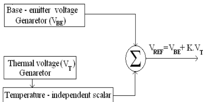
Figure 1. Concept of bandgap Voltage Reference
