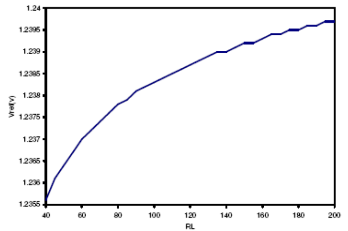
Figure 7. Variation of the reference voltage with RL at 27°C
