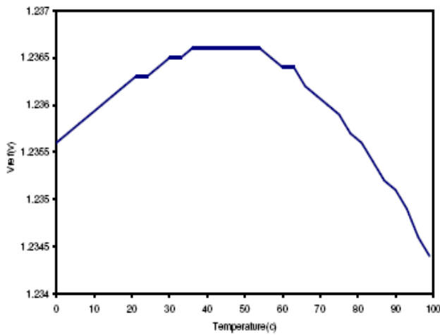
Figure 4. Variation of bandgap reference with temperature
