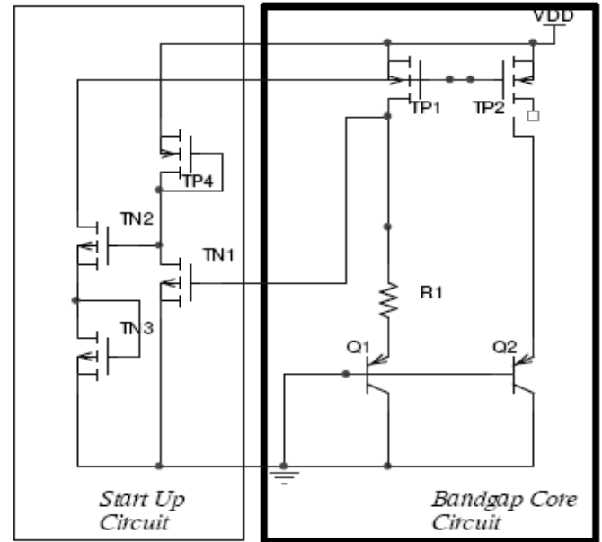
Figure 3. Schematic of Bandgap core Circuit with startup circuit
