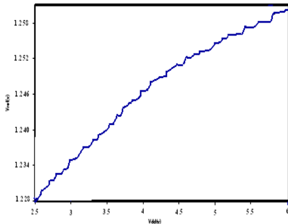
Figure 6. Variation of the reference voltage with supply voltage at 27°C
