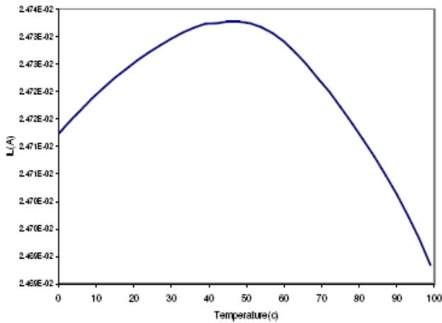
Figure 5. Variation of current load with temperature at Vdd=3.3v
