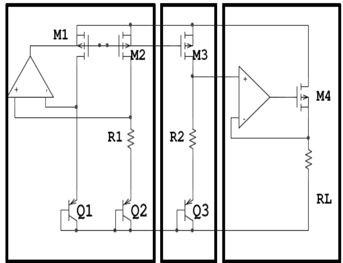
Figure 2. Schematic of Bandgap Reference Circuit showing the supply independent current source, generation of reference voltage and driving low Impedance block
