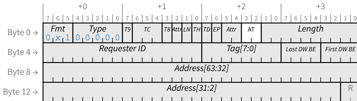
Figure 10-6 Memory Request Header with 64-bit Address
