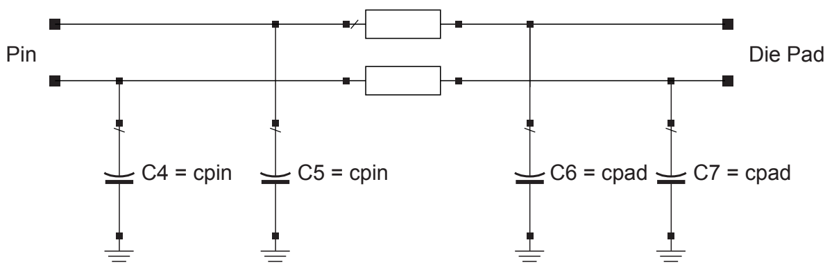
Figure 8-50 Tx/Rx Behavioral Package Models
