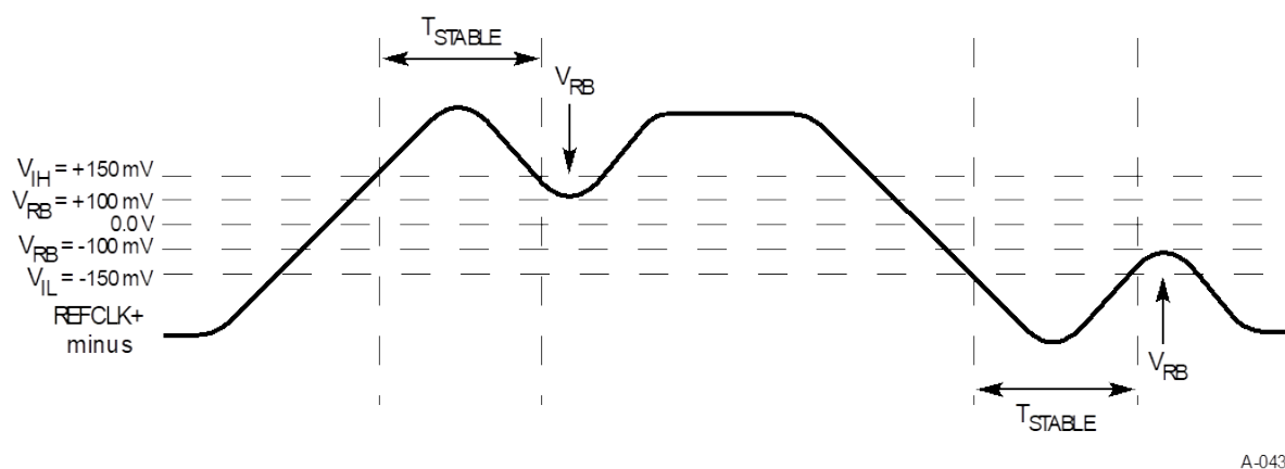
Figure 8-70 Differential Measurement Points for Ringback
