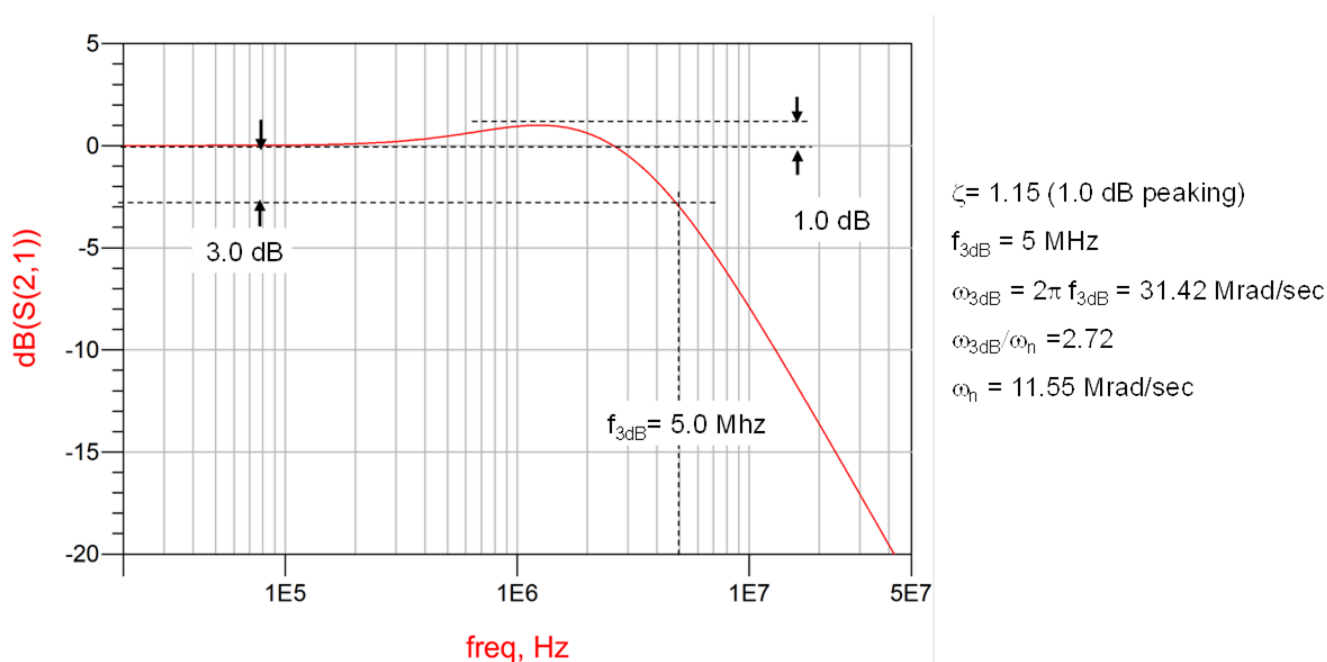
Figure 8-72 5 MHz PLL Transfer Function Example
