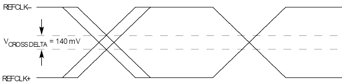
Figure 8-66 Single-Ended Measurement Points for Delta Cross Point
