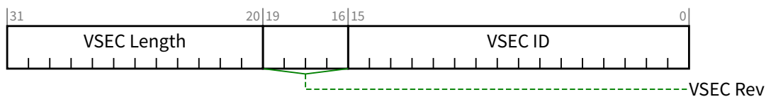
Figure 7-197 Vendor-Specific Header
