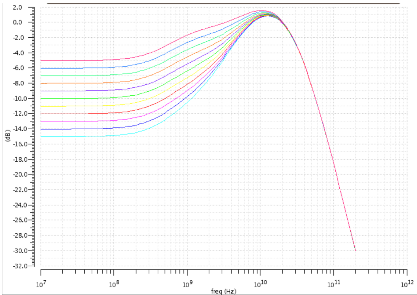
Figure 8-33 Loss Curves for 32.0 GT/s Behavioral CTLE
