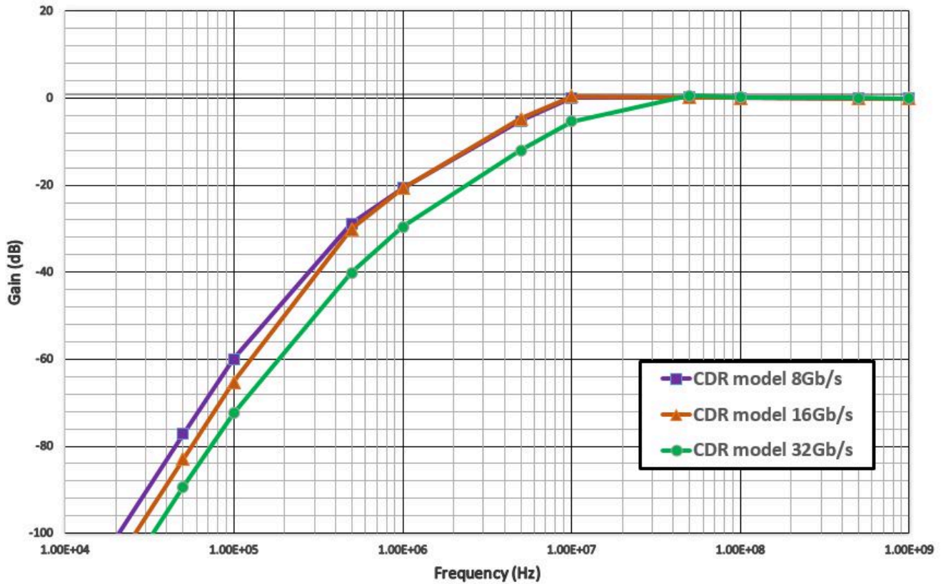
Figure 8-15 Behavioral SRIS CDR Function for 8.0 GT/s and SRIS and CC CDR for 16.0 GT/s
