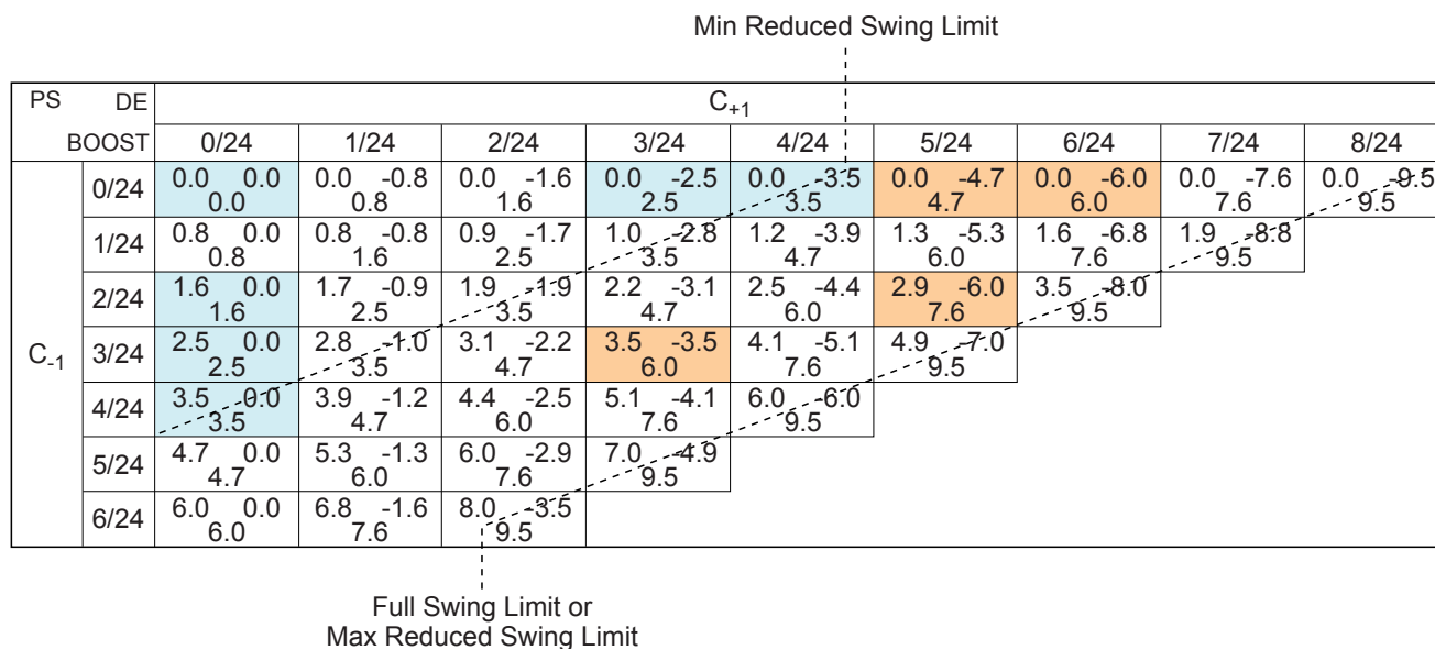
Figure 8-9 Transmit Equalization Coefficient Space Triangular Matrix Example
