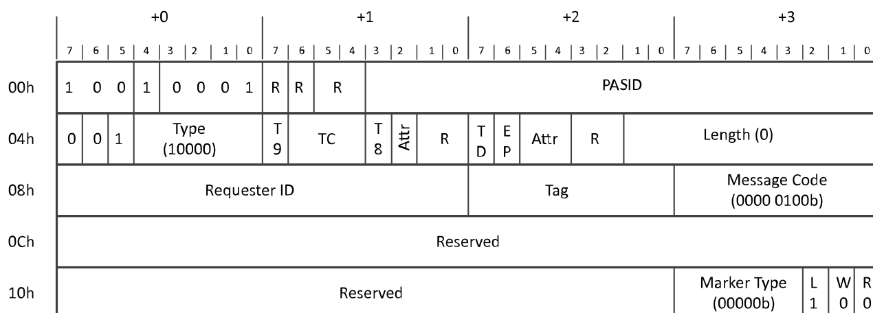
Figure 10-17 Stop Marker Message
