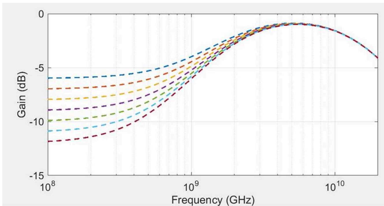
Figure 8-32 Loss Curves for 16.0 GT/s Behavioral CTLE
