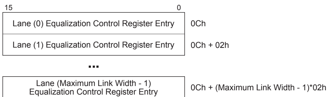
Figure 7-72 Lane Equalization Control Register
