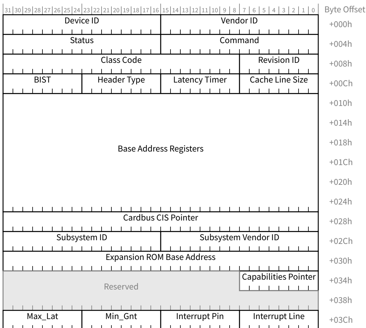
Figure 7-10 Type 0 Configuration Space Header
