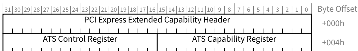
Figure 10-19 ATS Extended Capability Structure
