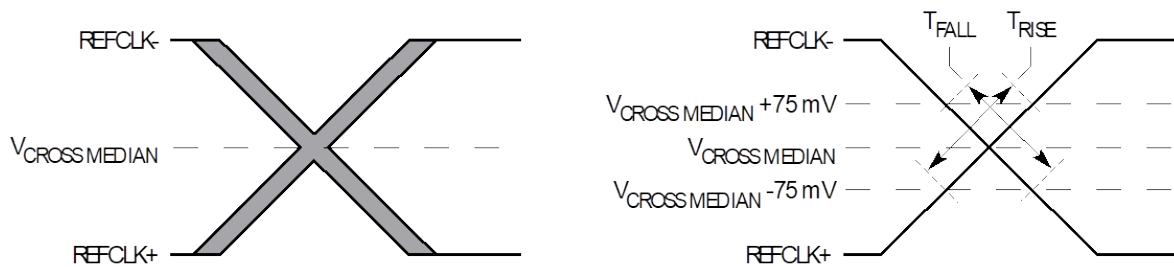
Figure 8-67 Single-Ended Measurement Points for Rise and Fall Time Matching
