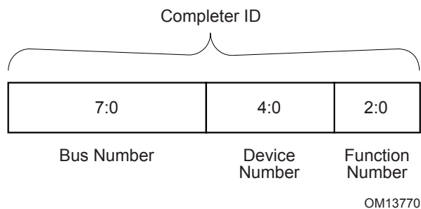
Figure 2-39 (Non-ARI) Completer ID
