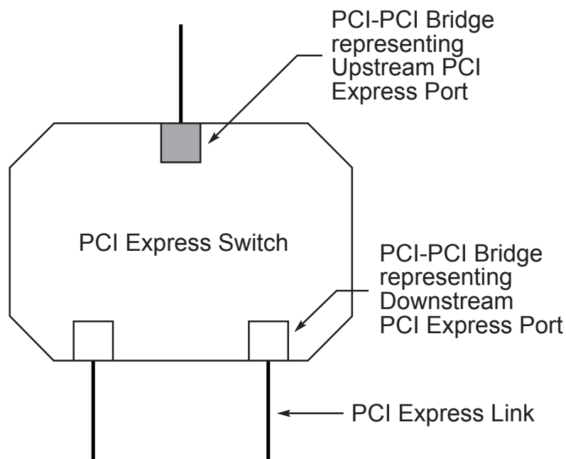
Figure 7-2 PCI Express Switch Device Mapping 130
