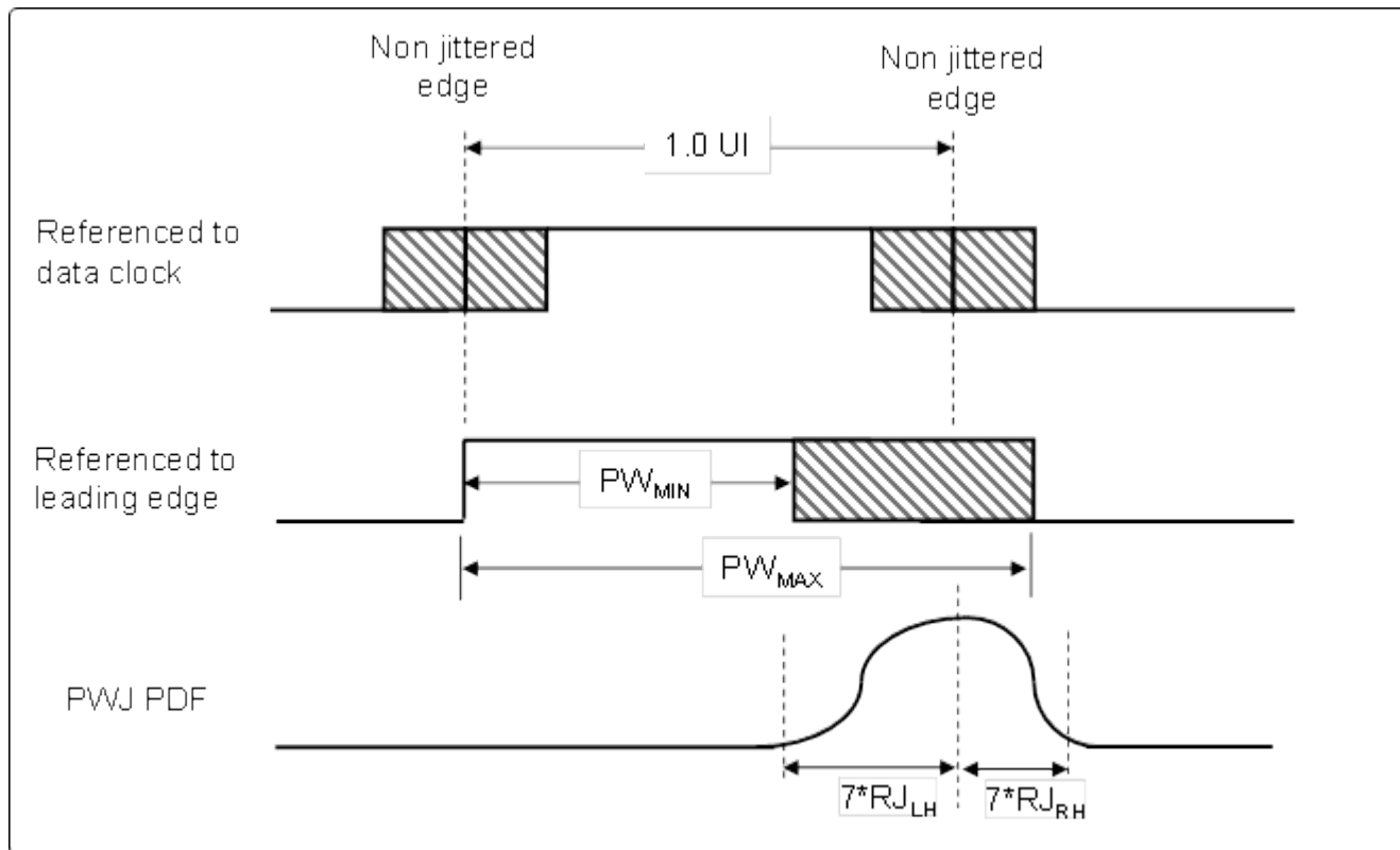
Figure 8-18 PWJ Relative to Consecutive Edges 1 UI Apart
