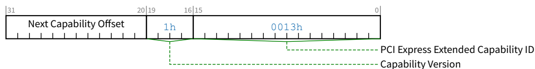
Figure 10-24 Page Request Extended Capability Header
