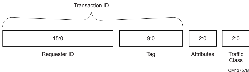
Figure 2-14 Transaction Descriptor
