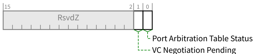
Figure 7-179 VC Resource Status Register
