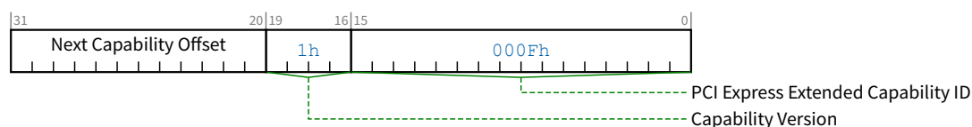
Figure 10-20 ATS Extended Capability Header
