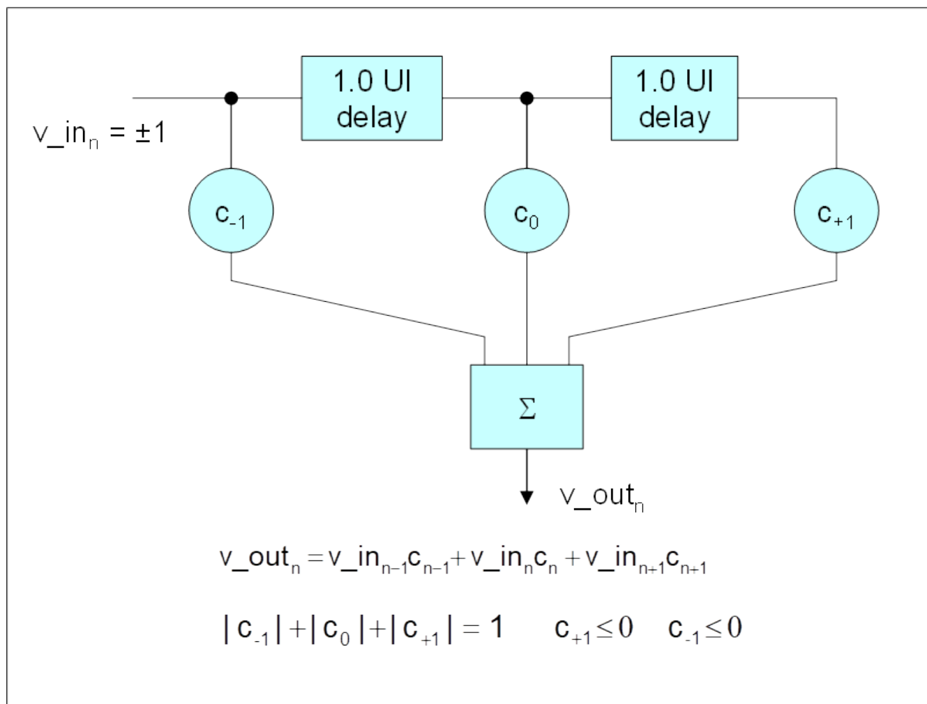
Figure 8-4 Tx Equalization FIR Representation
