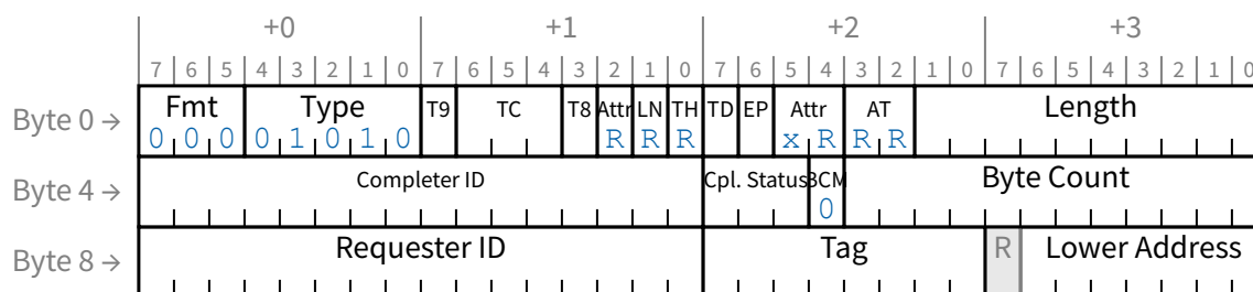
Figure 10-10 Translation Completion with No Data
