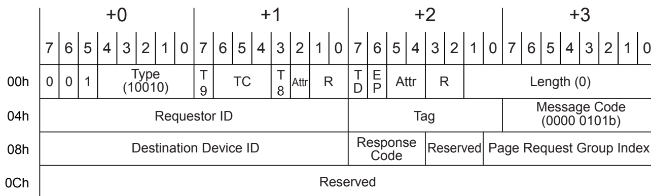
Figure 10-18 PRG Response Message
