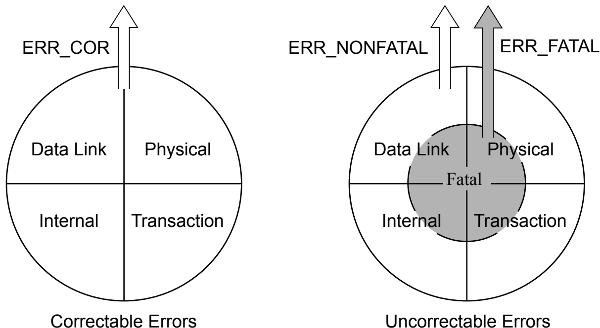
Figure 6-1 Error Classification
