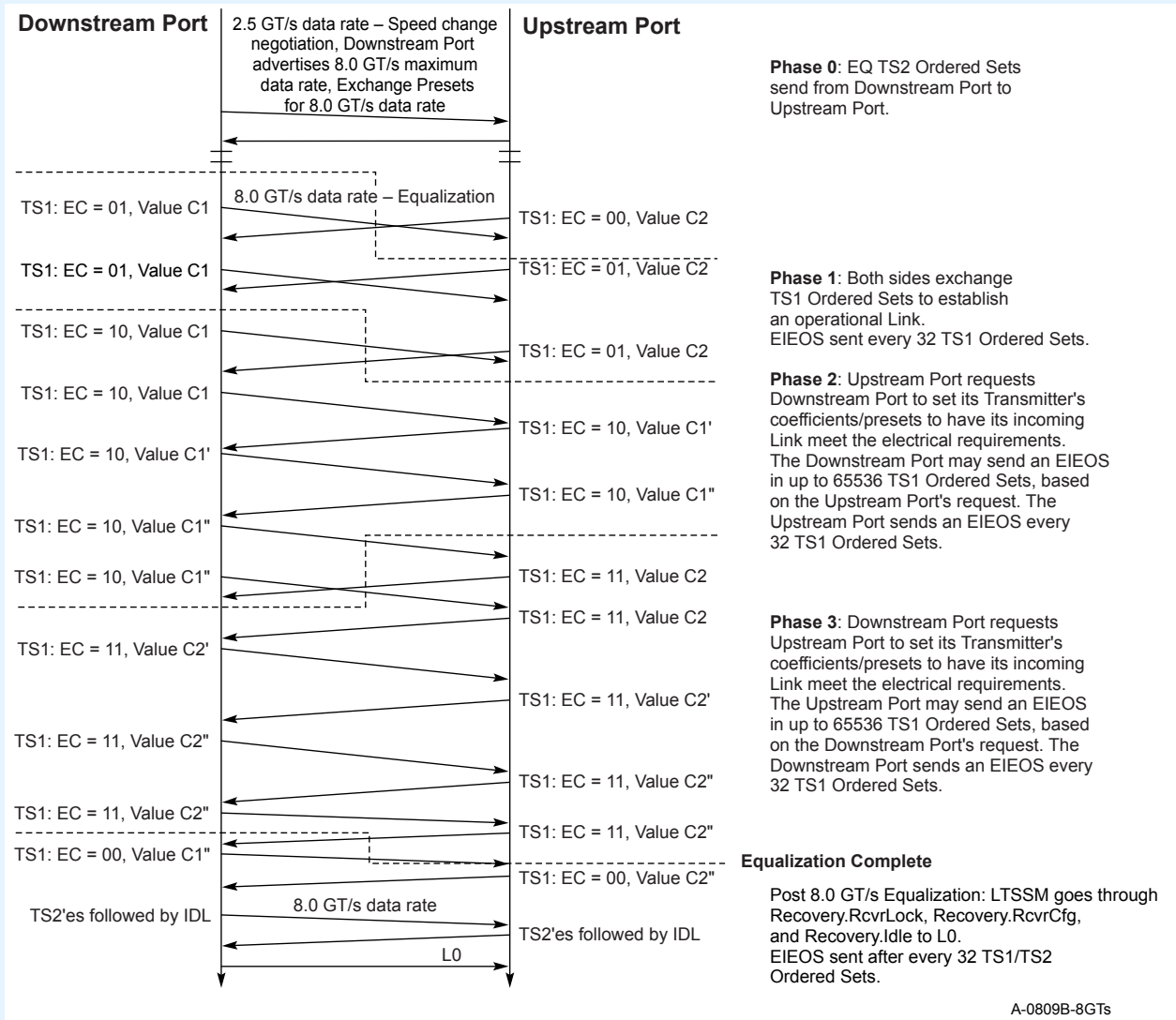
Figure 4-21 8.0 GT/s Equalization Flow
