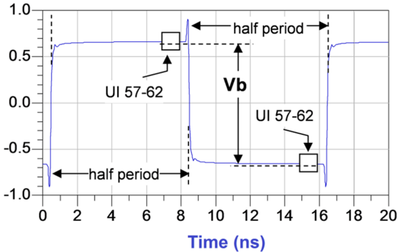
Figure 8-6 Waveform Measurement Points for Pre-shoot
