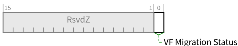
Figure 9-17 SR-IOV Status
