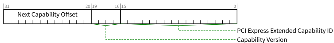
Figure 7-232 DPA Extended Capability Header
