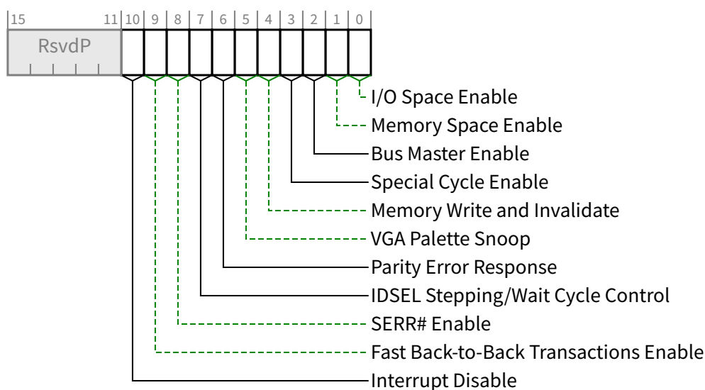
Figure 7-5 Command Register
