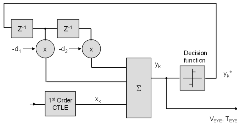
Figure 8-35 Diagram for 2-tap DFE
