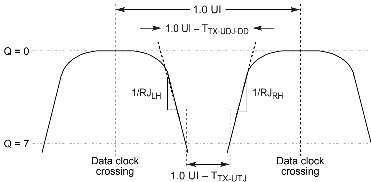
Figure 8-17 Derivation of T_{TX-UTJ} and T_{TX-UDJDD}
