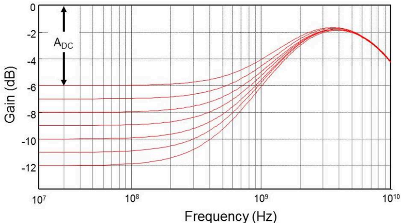
Figure 8-31 Loss Curves for 8.0 GT/s Behavioral CTLE
