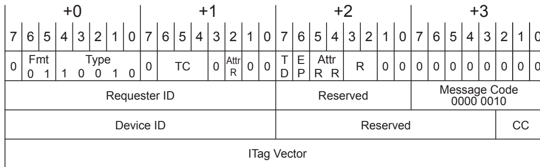
Figure 10-15 Invalidate Completion Message Format
