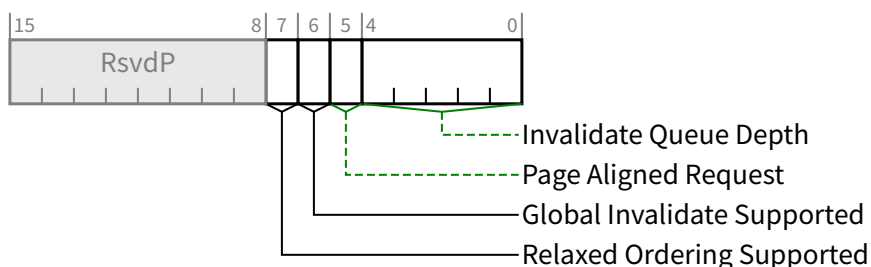
Figure 10-21 ATS Capability Register (Offset 04h)
