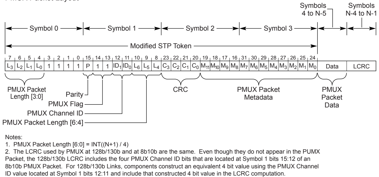
Figure G-6 TLP and PMUX Packet Framing (128b/130b Encoding)
