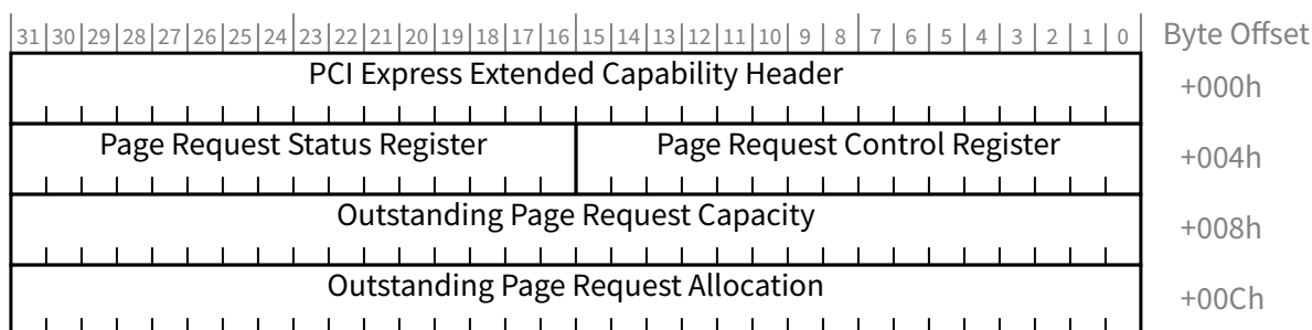
Figure 10-23 Page Request Extended Capability Structure
