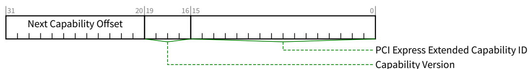
Figure 9-22 VF Resizable BAR Extended Capability Header
