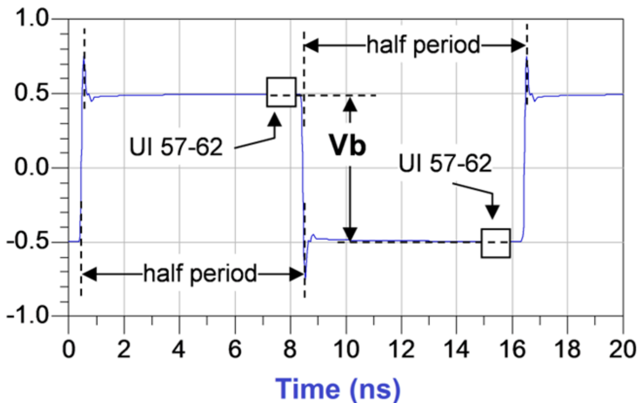
Figure 8-7 Waveform Measurement Points for De-emphasis
