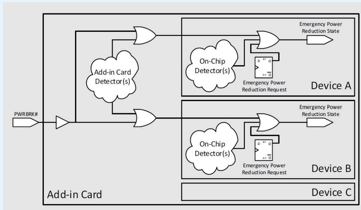
Figure 6-29 Emergency Power Reduction State: Example Add-in Card
