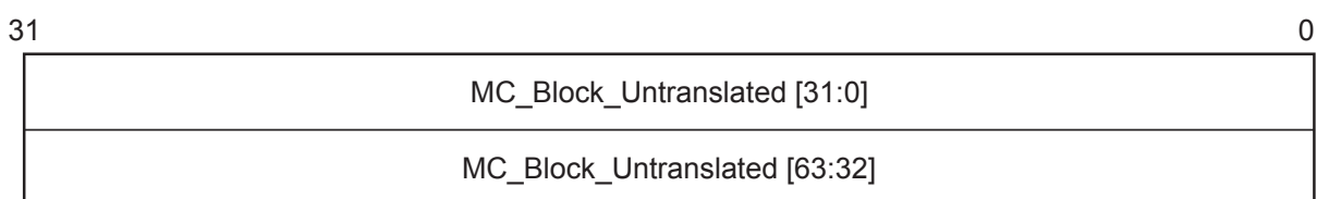
Figure 7-229 MC_Block_Untranslated Register
