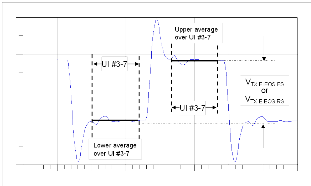
Figure 8-10 Measuring V_{TX-EIEOS-FS} and V_{TX-EIEOS-RS} at 8.0 GT/s
