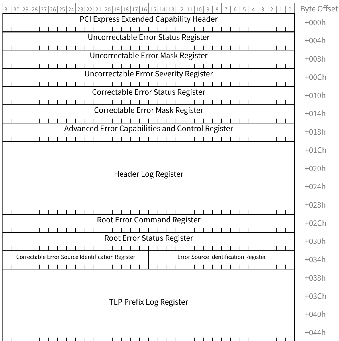
Figure 7-122 Advanced Error Reporting Extended Capability Structure
