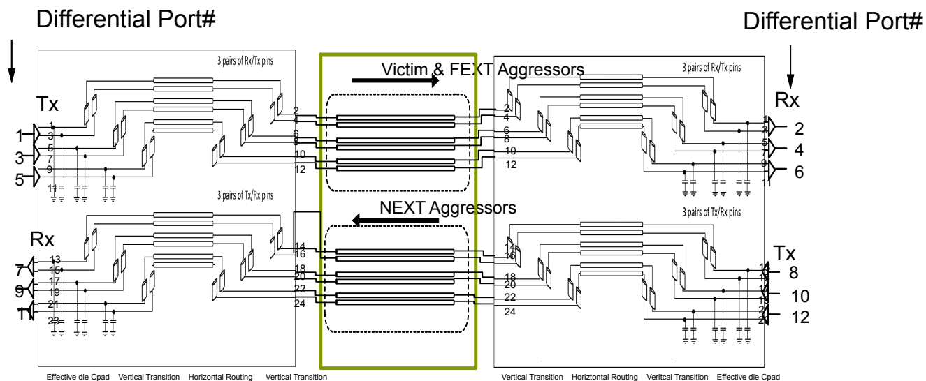
Figure 8-61 32.0 GT/s Reference Package Port Connections for Pin to Pin Channel Evaluation
