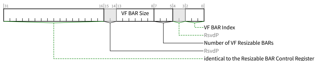
Figure 9-23 VF Resizable BAR Control Register
