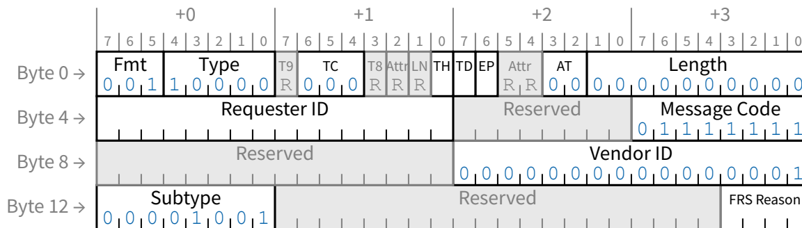
Figure 2-32 FRS Message
