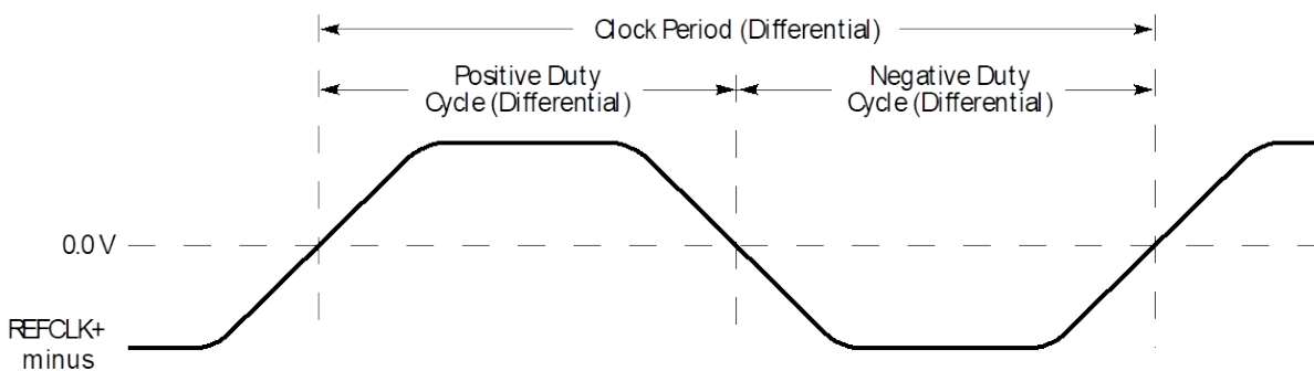
Figure 8-68 Differential Measurement Points for Duty Cycle and Period
