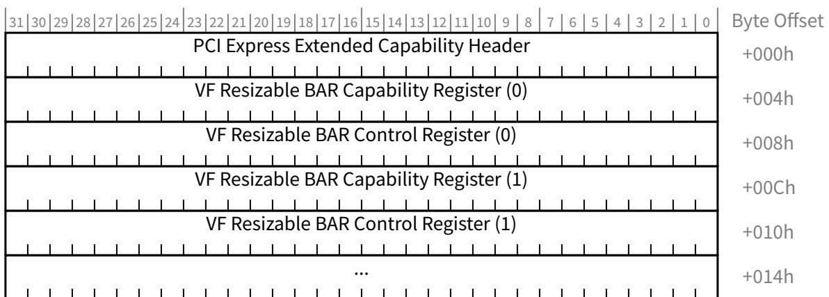
Figure 9-21 VF Resizable BAR Extended Capability
