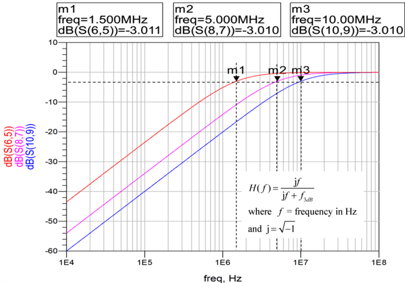
Figure 8-13 First Order CC Behavioral CDR Transfer Functions
