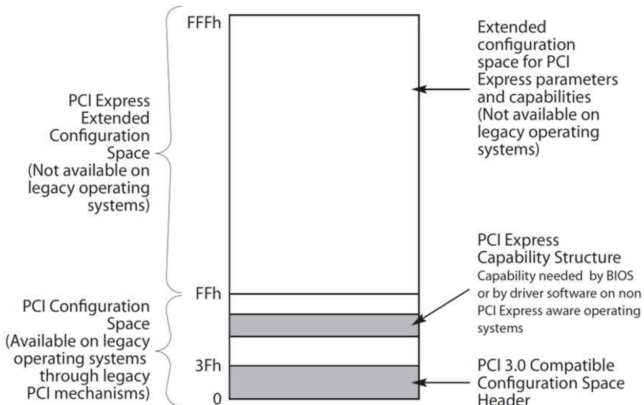
Figure 7-3 PCI Express Configuration Space Layout
