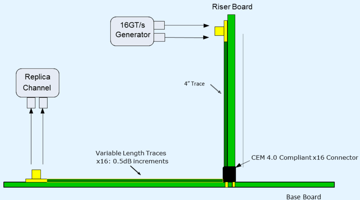
Figure 8-24 Example 16.0 GT/s Calibration Channel
