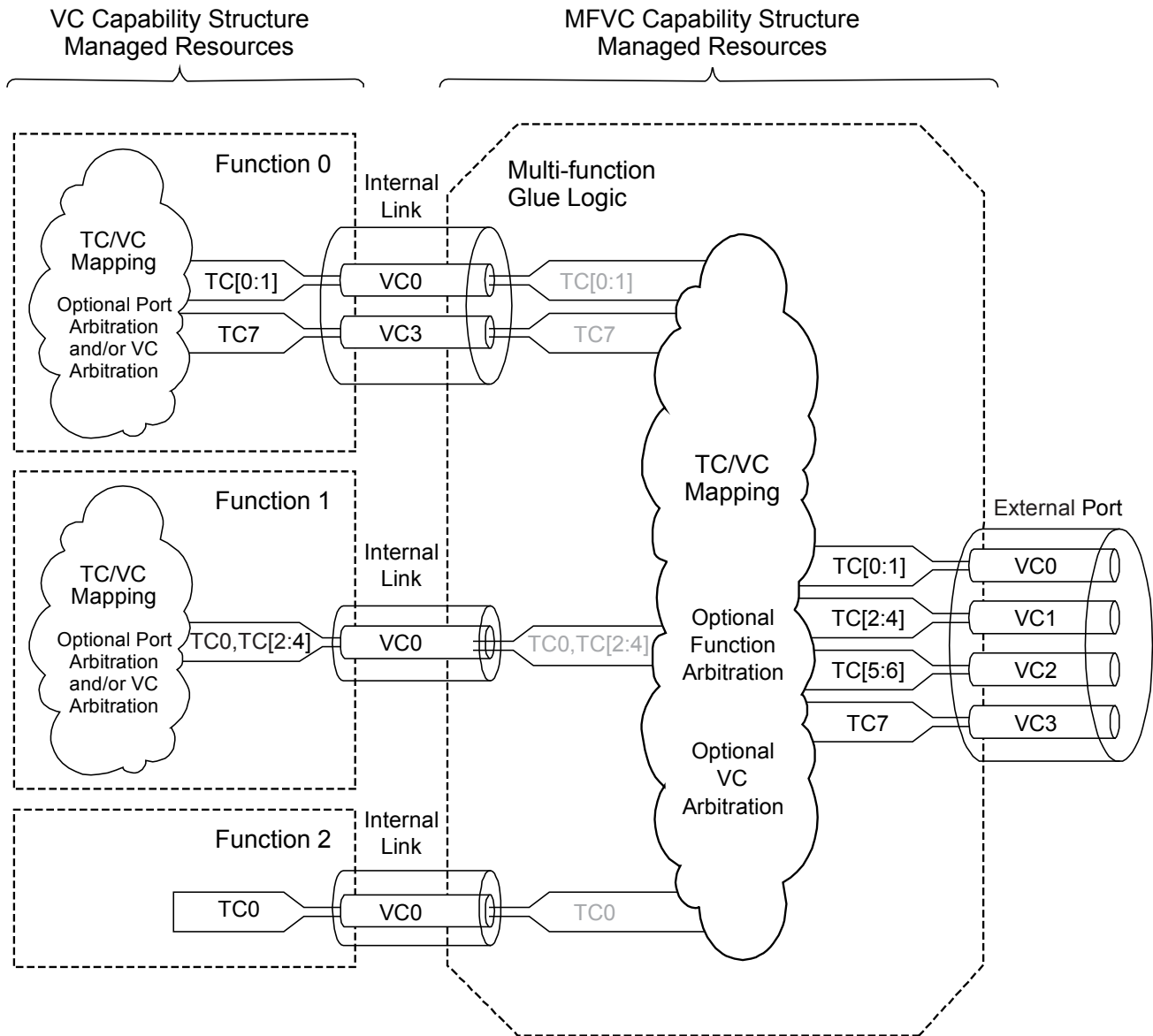
Figure 6-10 Multi-Function Arbitration Model
