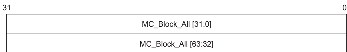
Figure 7-228 MC_Block_All Register
