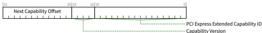
Figure 7-196 Vendor-Specific Extended Capability Header
