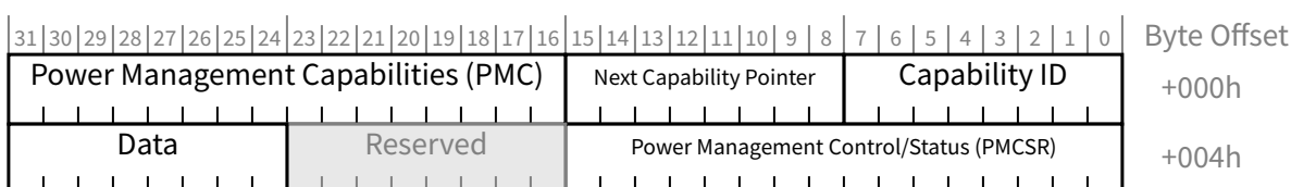
Figure 7-17 Power Management Capability Structure
