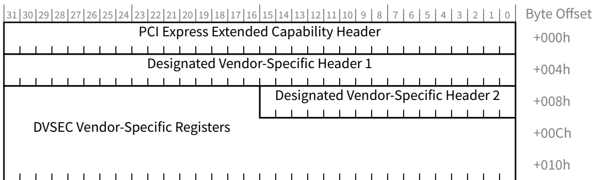
Figure 7-198 Designated Vendor-Specific Extended Capability
