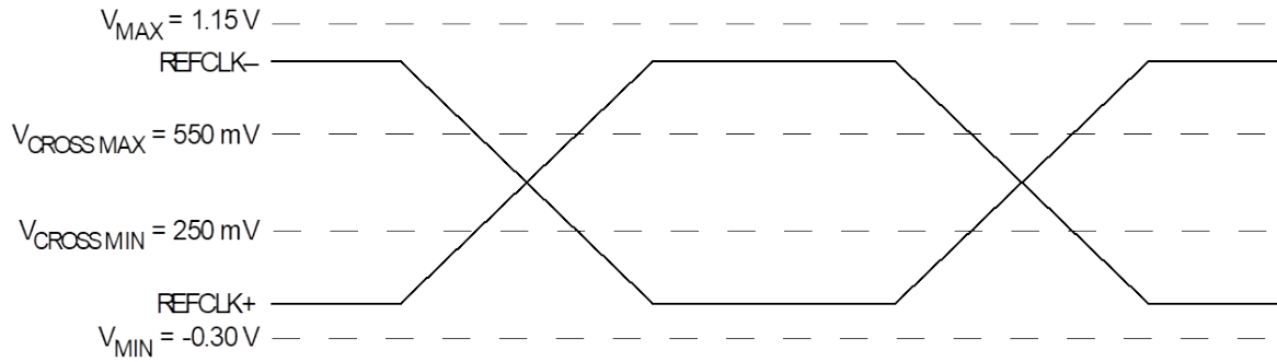
Figure 8-65 Single-Ended Measurement Points for Absolute Cross Point and Swing
