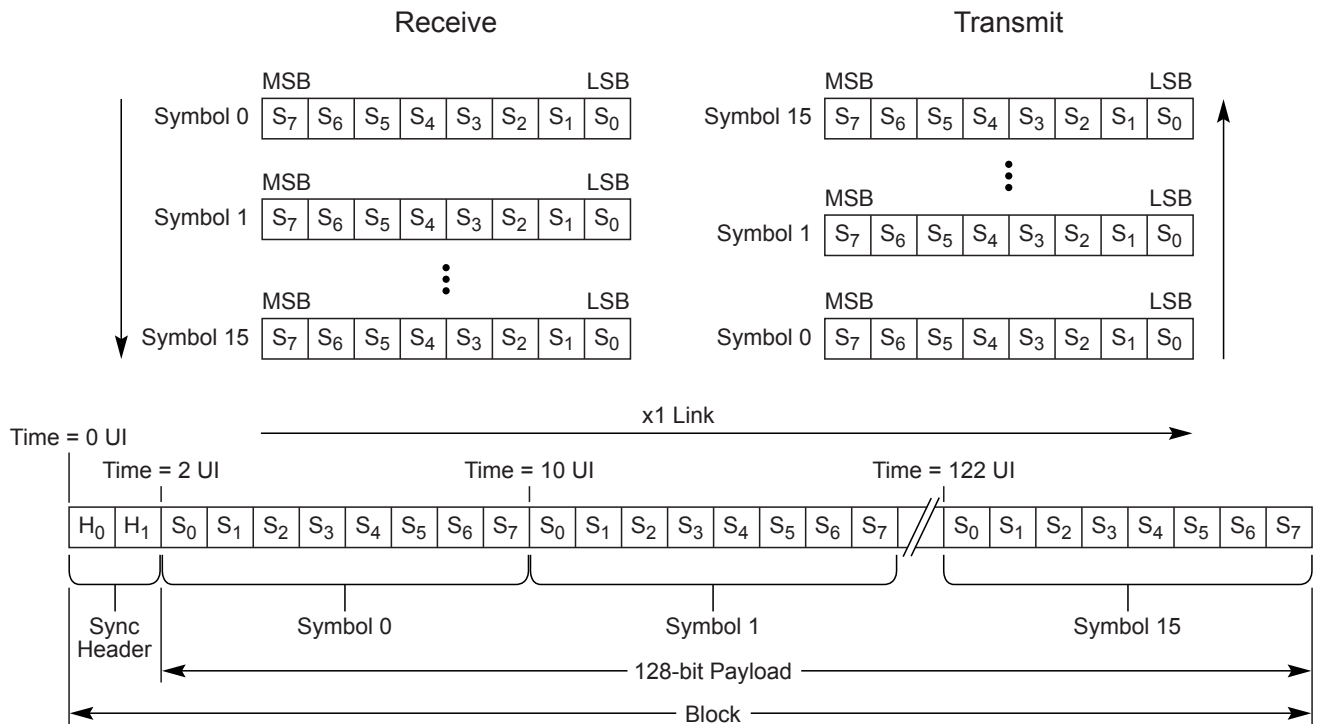
Figure 4-11 Example of Bit Transmission Order in a x1 Link Showing 130 Bits of a Block
