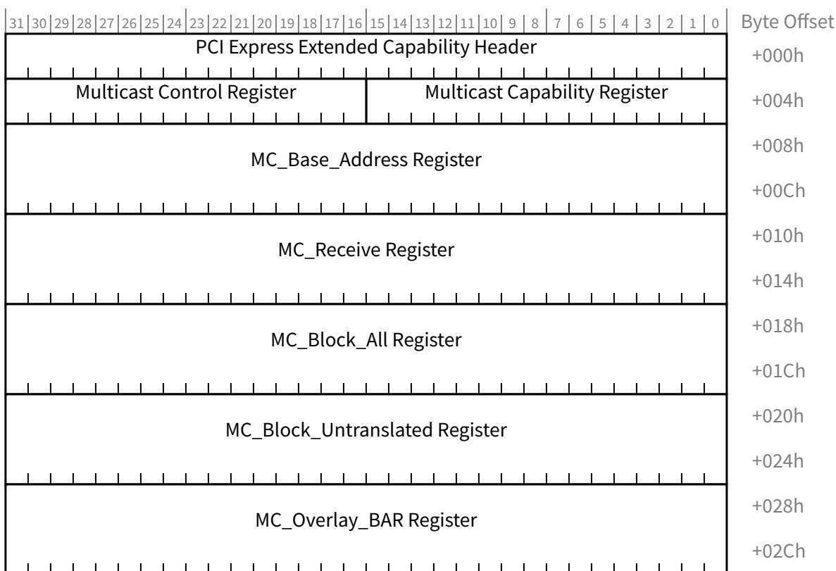
Figure 7-222 Multicast Extended Capability Structure
