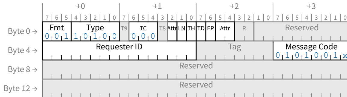
Figure 2-36 PTM Request/Response Message
