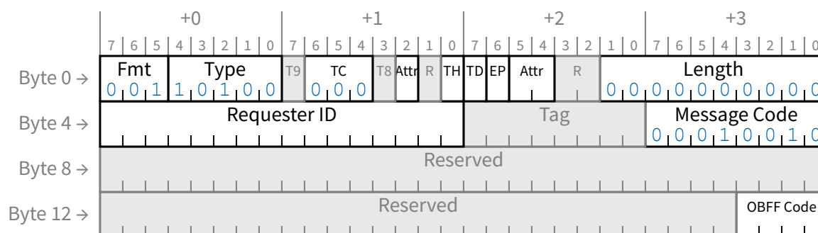
Figure 2-35 OBFF Message
