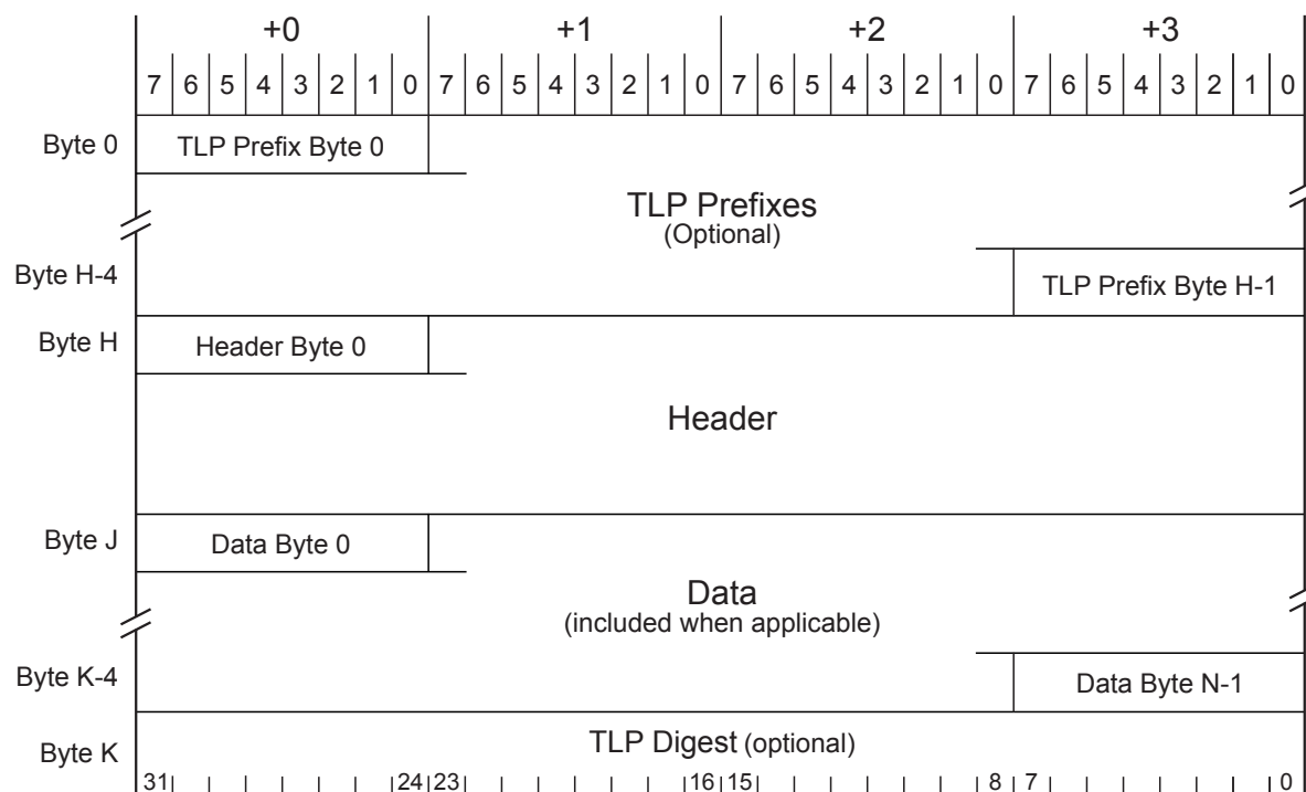
Figure 2-3 Generic TLP Format
