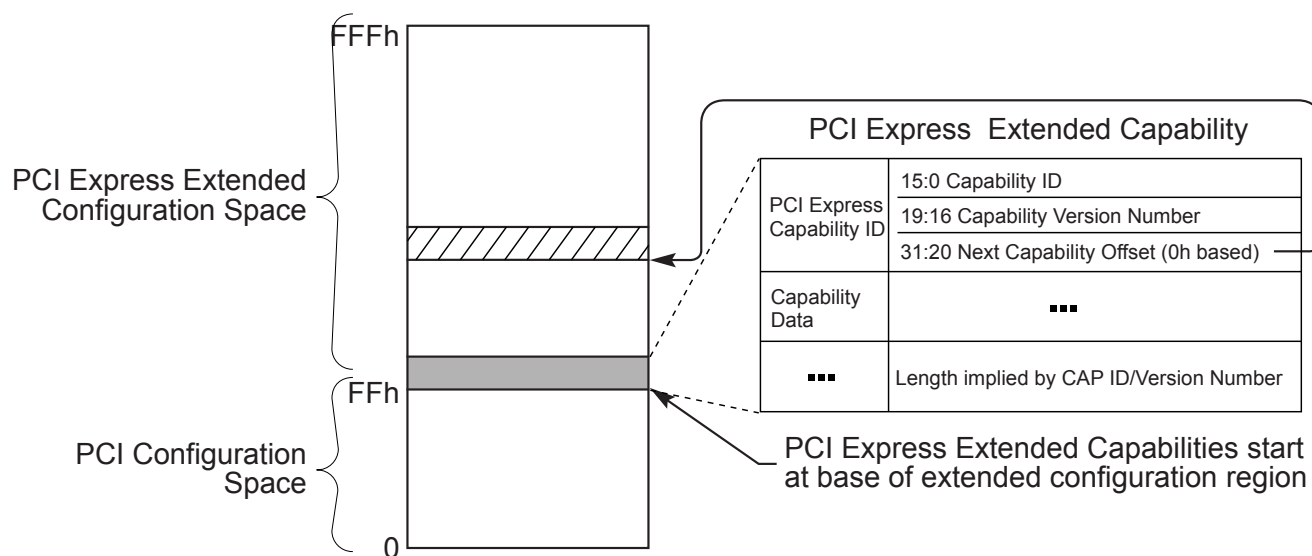
Figure 7-42 PCI Express Extended Configuration Space Layout
