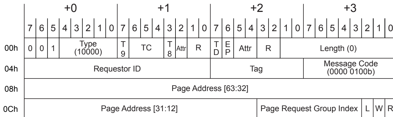
Figure 10-16 Page Request Message
