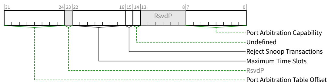
Figure 7-177 VC Resource Capability Register
