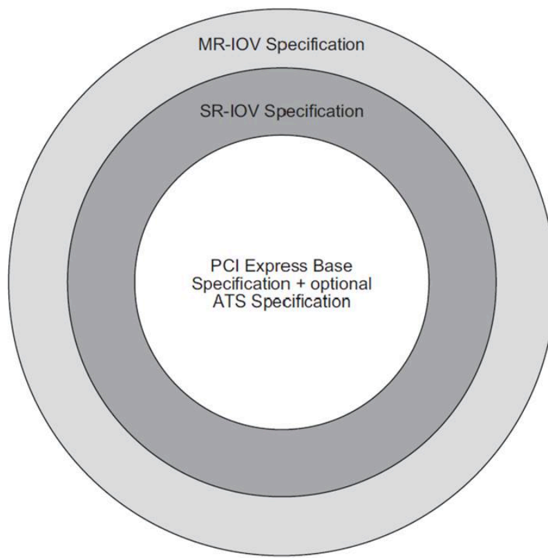
Figure 9-9 I/O Virtualization Interoperability
