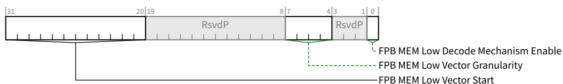
Figure 7-166 FPB MEM Low Vector Control Register
