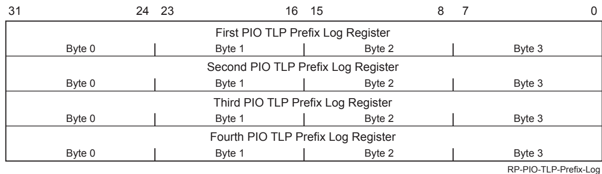
Figure 7-262 RP PIO TLP Prefix Log Register
