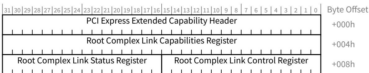
Figure 7-214 Root Complex Internal Link Control Extended Capability
