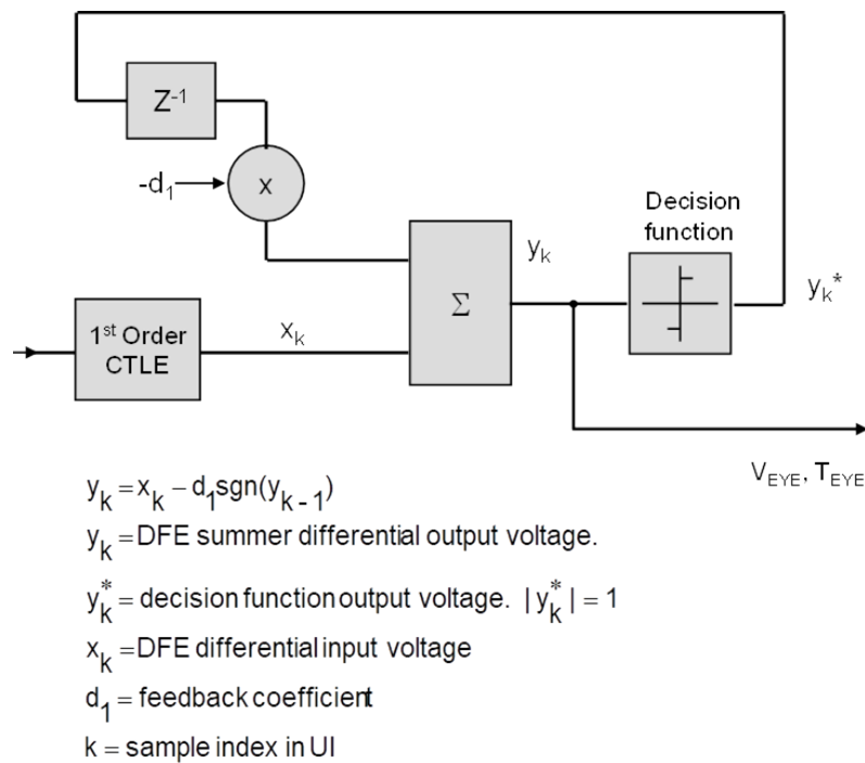
Figure 8-34 Variables Definition and Diagram for 1-tap DFE
