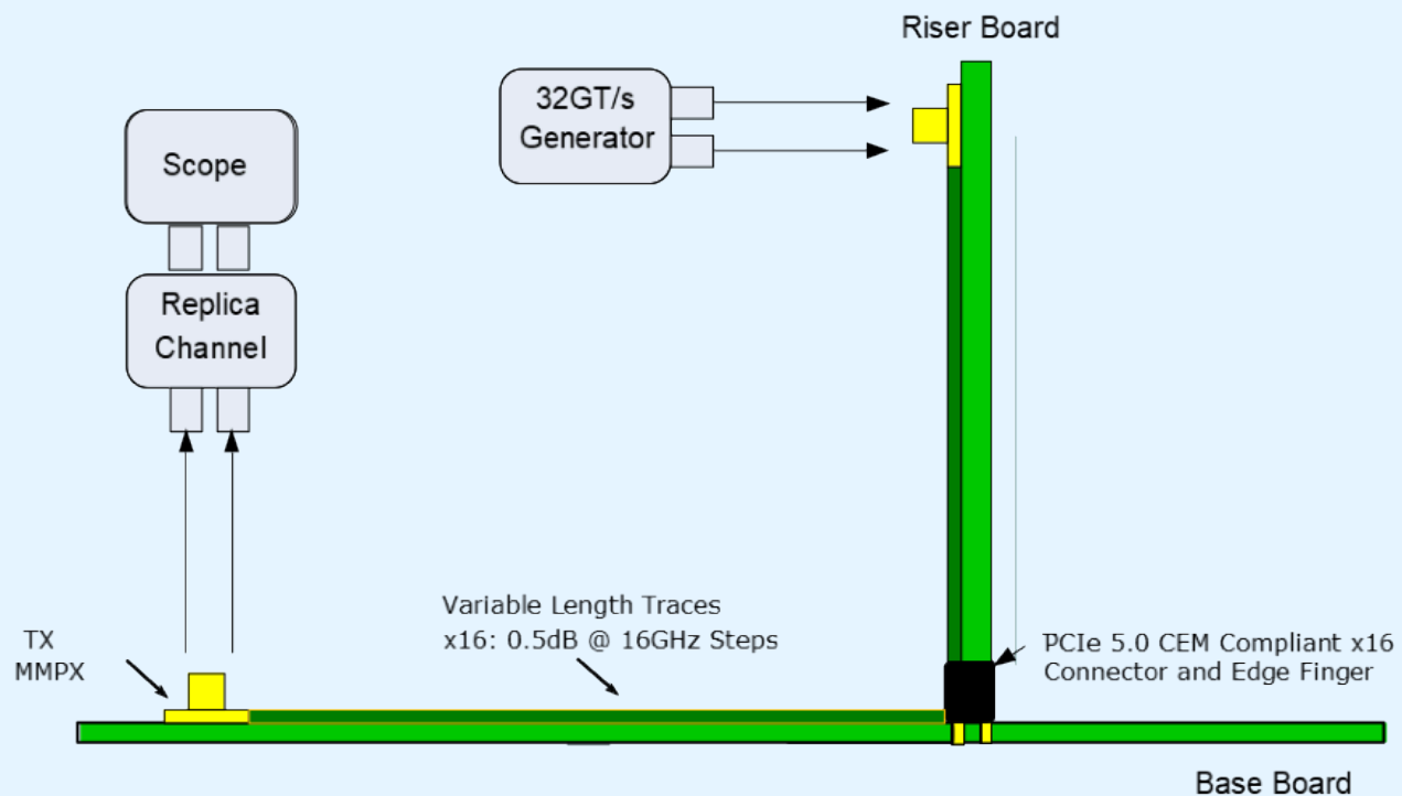
Figure 8-28 Example 32.0 GT/s Calibration Channel
