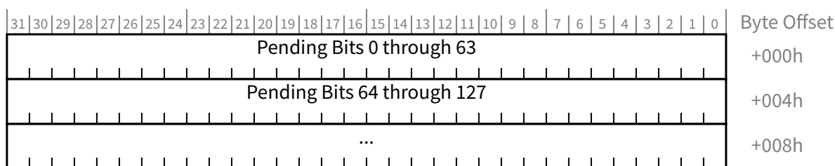
Figure 7-58 MSI-X PBA Structure
