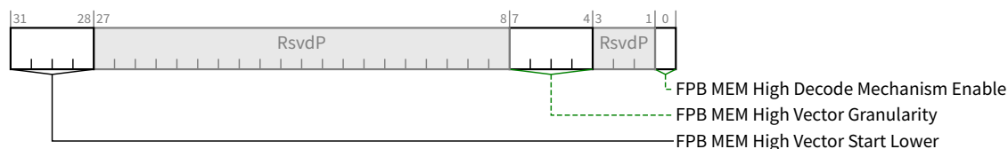
Figure 7-167 FPB MEM High Vector Control 1 Register
