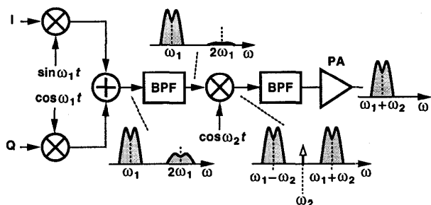
Fig. 20. Two-step transmitter.
