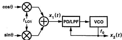
Fig. 21. Upconversion of a constant-envelope signal by means of a PLL.
