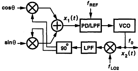
Fig. 24. Offset PLL including quadrature upconversion.
