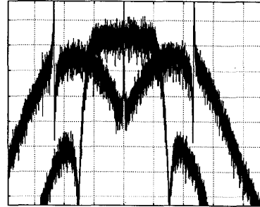
Fig. 26. Simulated spectra of the two terms in Eq. (4). (Horiz. scale normalized to bit rate, vert. scale: 5 dB/div.)
