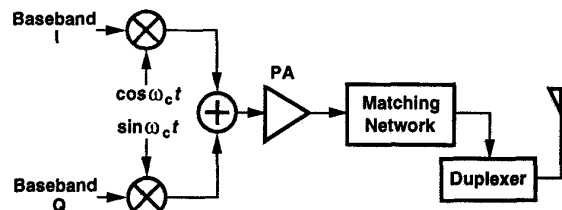
Fig. 16. Direct-conversion transmitter.
