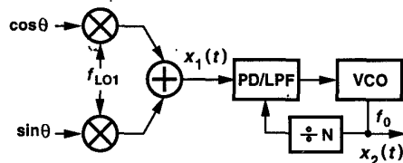
Fig. 22. Upconversion of a constant-envelope signal by means of a PLL with feedback divider.
