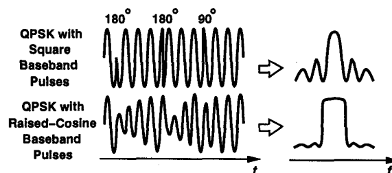
Fig. 4. Variation of envelope with raised-cosine baseband pulses.
