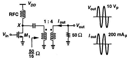
Fig. 27. Simple PA with matching network.
