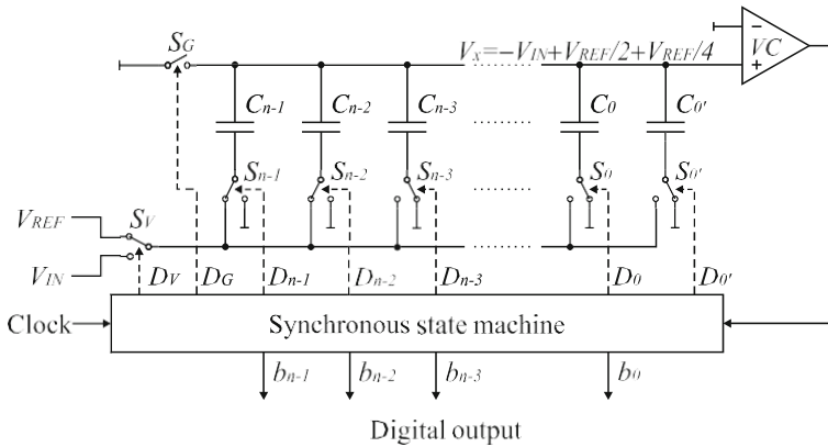
Fig. 6.13 The C-ADC circuit diagram. The controlled switch states correspond to the second step of redistribution mode assuming that the MSB has been evaluated to 'one'
