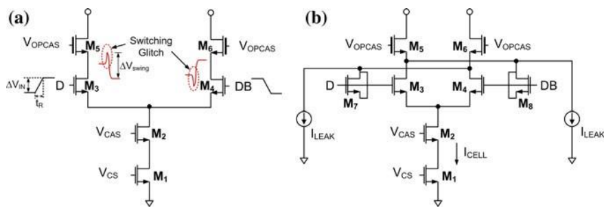
Fig. 3.19 a High-speed switching glitches in a DAC cell b A modified DAC cell with leakers and neutralization switches
