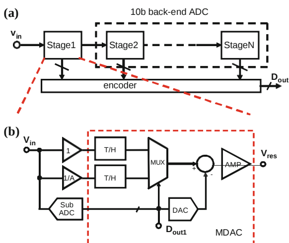
Fig. 1.12 a The architecture of the proposed pipeline ADC, b block diagram of the first pipelined stage with parallel sampling technique
