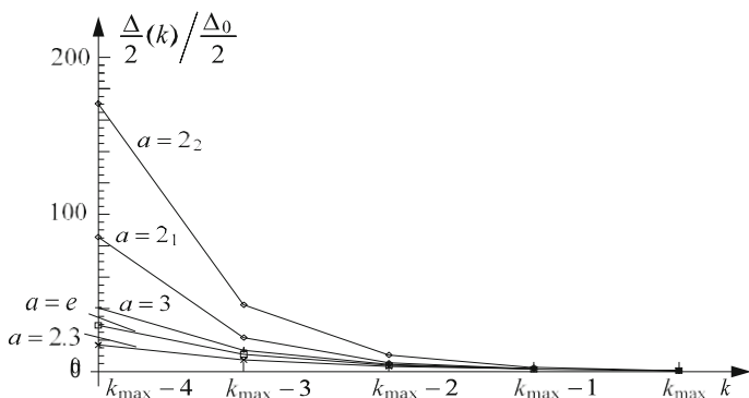
Fig. 9.8 The worst case settling to TD_0=2 during the last four steps ( a \approx 2_1; 2_2; 2.3; e; 3 )
