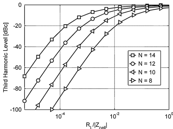
Fig. 3.14 HD_3 performance vs. R_L = Z_{CELL} \delta \theta_P
