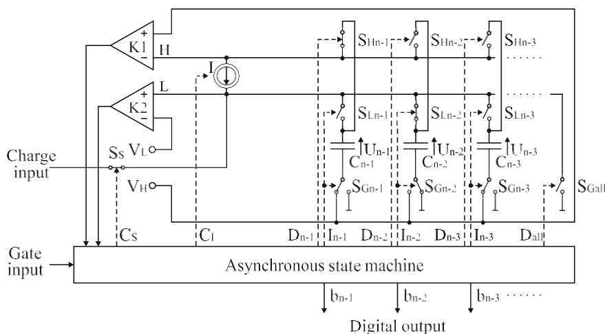
Fig. 6.23 Circuit diagram of the DSCR-ADC. The states of the controlled switches correspond to the second step of the accumulation/conversion phase when the input charge provided to the charge input is collected in the capacitor C_{n-2}
