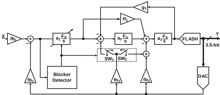
Fig. 2.22 Architecture of the proposed RD ADC
