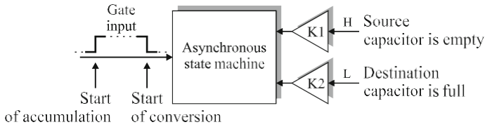
Fig. 6.8 Classes of events timing SCR-ADC conversion cycle
