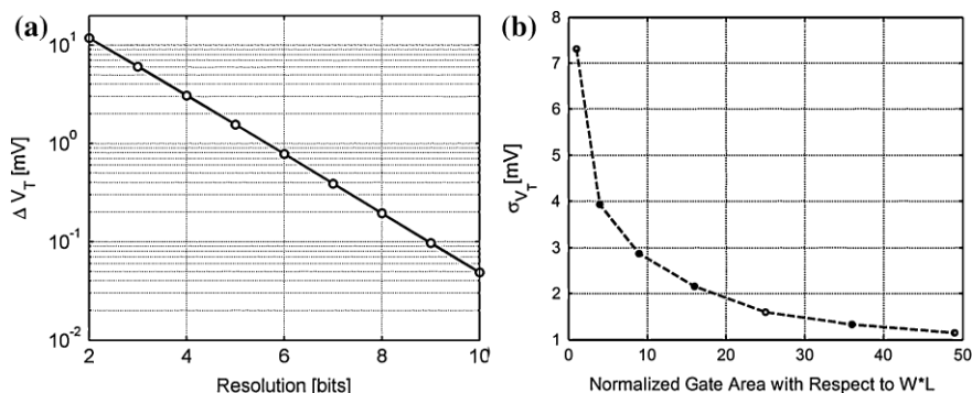
Fig. 3.23 a DV_T vs. Resolution b \sigma_{V_T} mismatch as a function of gate area
