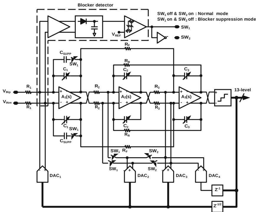
Fig. 2.38 Schematic of the proposed RD ADC
