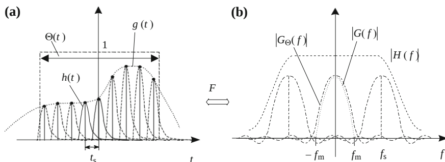
Fig. 9.3 Signal sampling process waveforms in the time domain (a) and the frequency domain (b) where |G_\Theta(f)| is the Fourier spectrum amplitude part of the signal before sampling and windowing, |G(f)| is the Fourier spectrum amplitude part of the windowed signal, and |H(f)| is frequency spectrum of the sampling pulses
