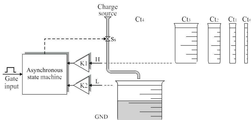
Fig. 6.1 Liquid accumulation
