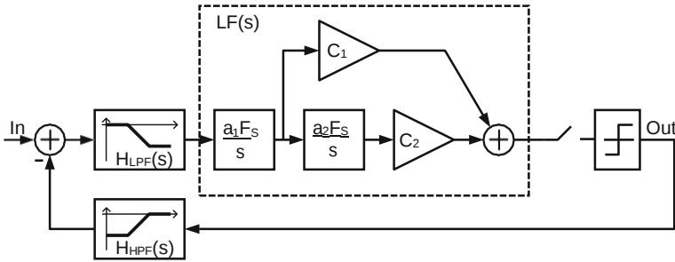
Fig. 2.17 RD ADC with increased interferer immunity (see footnote 15)
