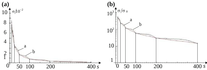
Fig. 9.23 Standard deviations (a) and ratios of the standard deviations to r_{D_0} (b) in relation to the sampling ratio s of the 12-bit adaptive A/D converter: a approximation using the probability distributions of the approximation steps like in Fig. 9.21; b results of tracking the signal
