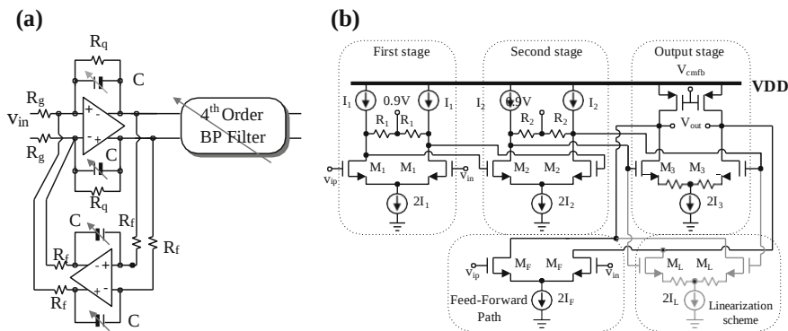
Fig. 4.8 6th order bandpass filter. a RC filter architecture b linearized OPAMP
