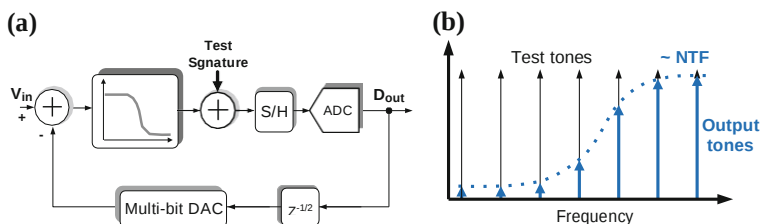
Fig. 4.5 a NTF characterization for a low-pass RD modulator b input and output test tones
