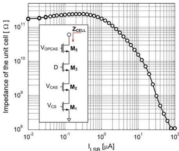
Fig. 3.16 DAC cell impedance as a function of current
