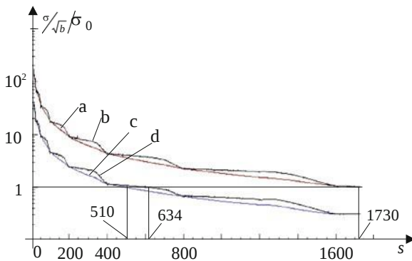
Fig. 9.24 Ratios of standard deviations of the adaptive A/D conversion to r_{D_0} in relation to the sampling ratio s : a approximation using the probability distributions of the approximation steps with 12-bit A/D converter; b results of tracking the signal with 12-bit A/D converter; c approximation using the probability distributions of the approximation steps with 10-bit A/D converter; d results of tracking the signal with 10-bit A/D converter
