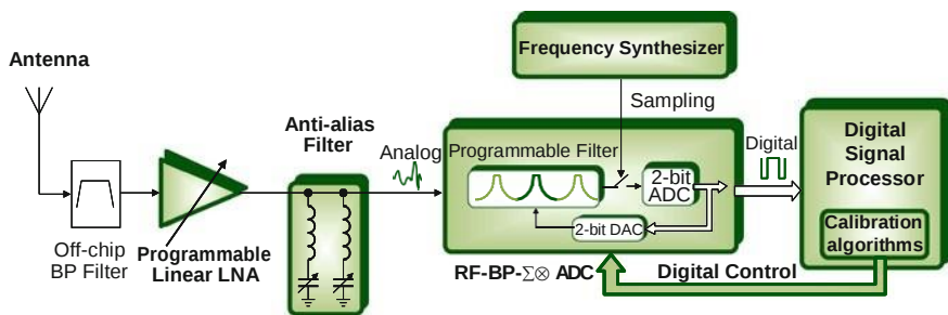
Fig. 4.14 RF-to-Digital converter employing an anti-alias filter and the BP-RD modulator
