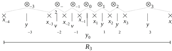
Fig. 9.5 Representatives y_i \propto 2^{i-1}D_0 and threshold levels x_i of the non-uniform exponential quantization in the measurement range R_3 for base a \propto 2 and i \propto 1; 2; 3
