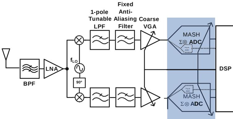
Fig. 2.15 Receiver architecture with a reconfigurable DT MASH RD ADC (see footnote 15)
