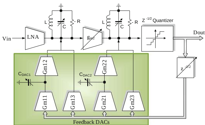
Fig. 4.15 Schematic for the 4th order RF BP-RD modulator
