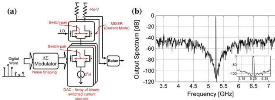
Fig. 3.27 a A simplified block diagram of a radio-frequency digital-to-analog converter b RF Output Spectrum using 2nd-order, 3-bit DR Modulator
