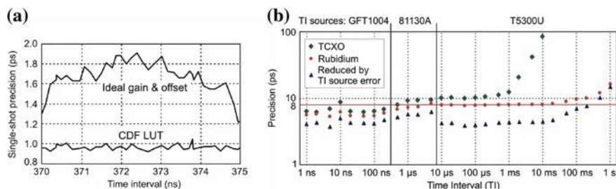
Fig. 7.25 Precision of a TIC within a single clock period (a) [21], and within a wide measurement range (b) [34]
