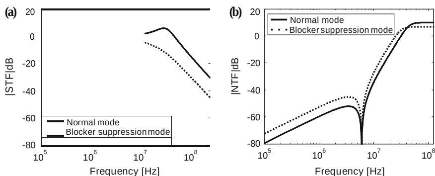
Fig. 2.23 RD ADC a STF and b NTF of the normal and blocker suppression mode
