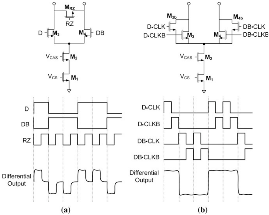
Fig. 3.25 DAC cell with a Return-to-zero (RZ) Switching b Differential-Quad Switching (DQS)
