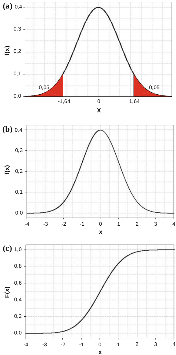
Fig. 13.3 Probability density function (PDF) for a Gaussian distribution M \sim N(l, r^2) ; b Probability density function (PDF); c Cumulative distribution function for standardized Gaussian Z \sim N(0, 1)
