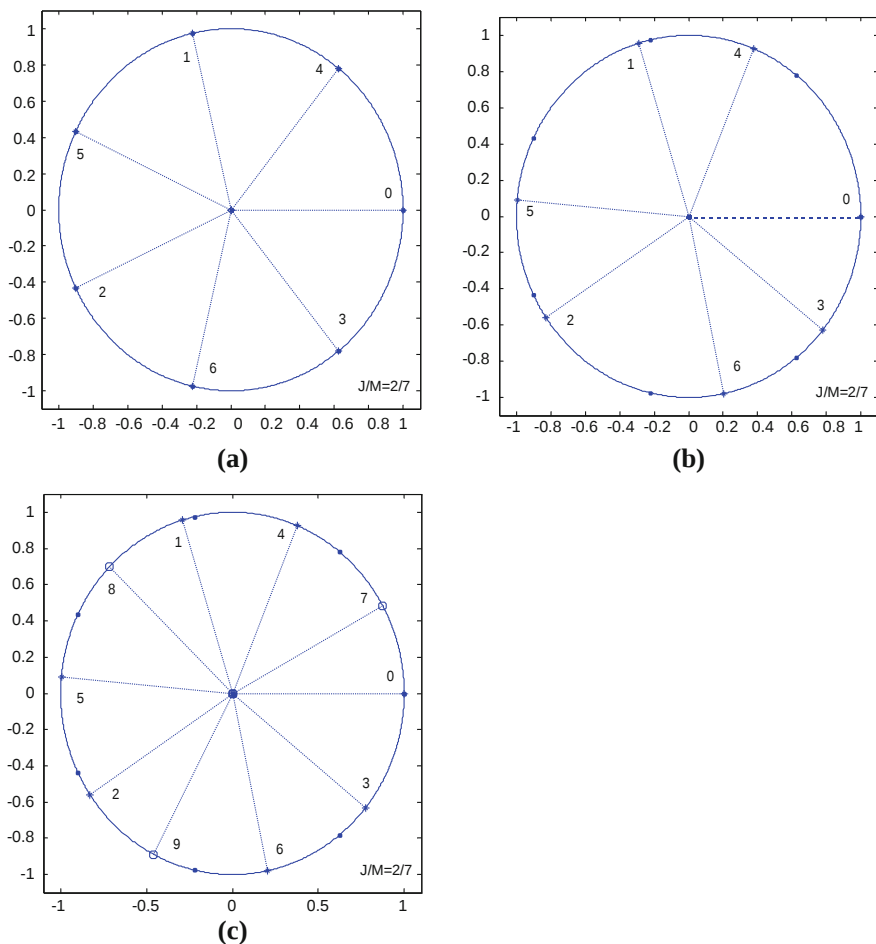
Fig. 11.5 Phase gaps D/ for M = 7 collected samples, with f_i/f_s = J/M = 2/7 , when sampling is coherent (a), and when the ratio slightly differs from 2/7 , before (b) and after (c) collecting 3 more samples
