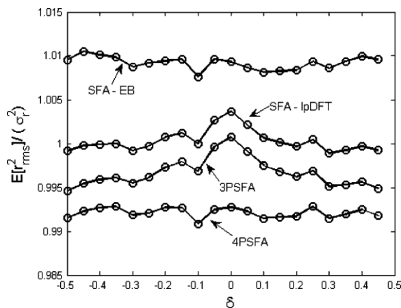
Fig. 10.2 Ratio E \hat{r}_{rms}^2 = r_r^2 provided by simulation results (circles) versus d . The number of acquired samples was M = 512
