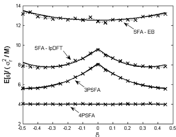
Fig. 10.1 Ratio E[\hat{r}_{rms}^2] / r_r^2 = M provided by theoretical (continuous line) and simulation (crosses) results versus d . The number of acquired samples was M = 512
