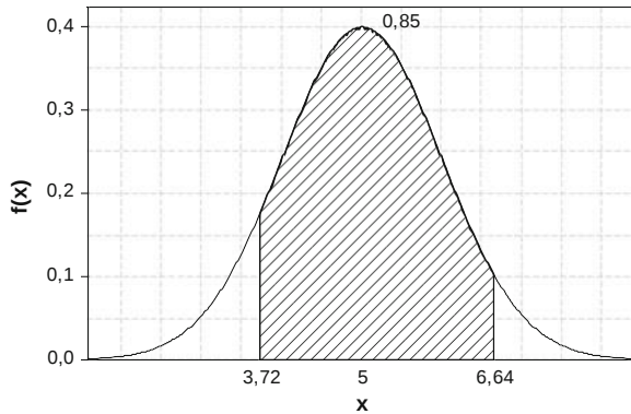
Fig. 13.7 PDF of a normal distribution with expected value equal to 5 and standard deviation equal to 1. The three regions under the curve, from the left, correspond respectively to a = 0.1 ; p = 0.85 and (1-p-a) = 0.05
