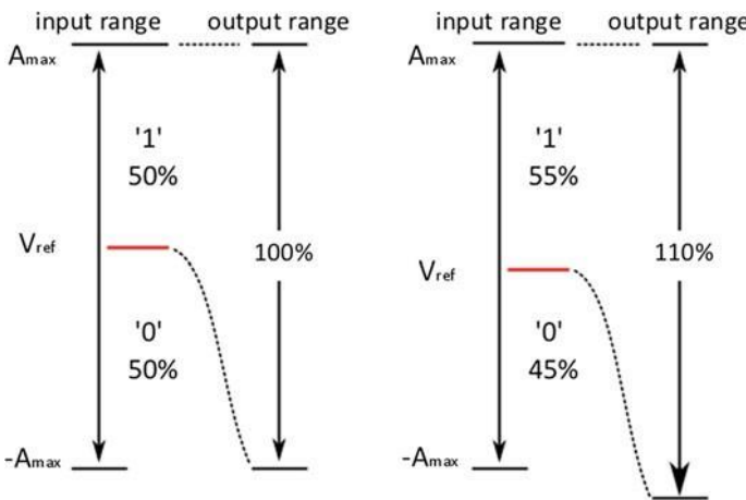
Fig. 1.8 Ideal behavior (left) and behavior in case of deviation of V_{ref} (right) of a 1b per stage converter
