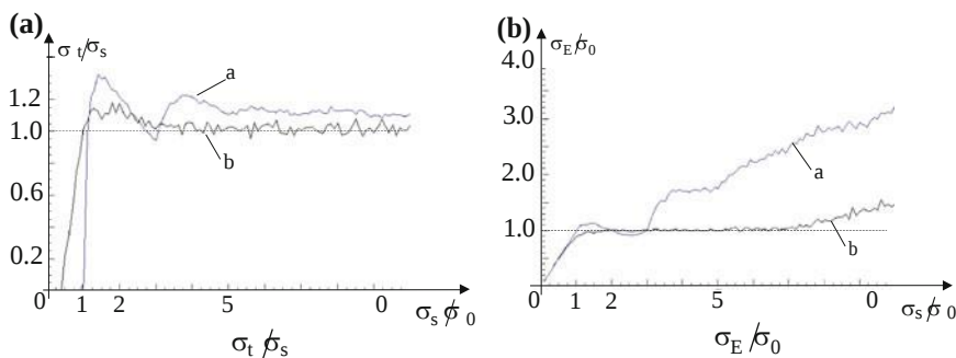
Fig. 9.19 Ratios of the standard deviations of the tracking values r_t to the standard deviation of the input noise r_s (a) and the standard deviations of the output errors ( r_{E \approx r_{g,-g}} ) to the minimal quantization standard uncertainty r_0 (b): a the rectangular noise distribution, b the Gaussian noise distribution
