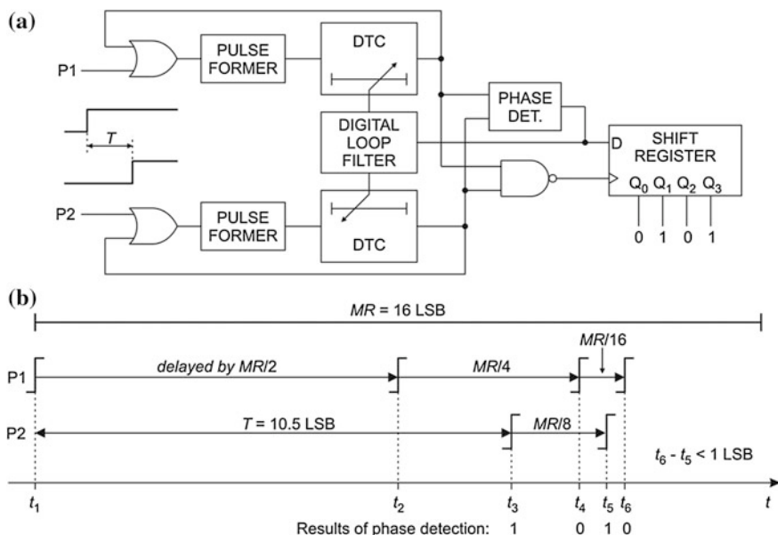
Fig. 7.17 Simplified block diagram of a 4-bit TDC based on CTDSA (a) and related timing diagram (b)
