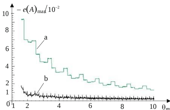
Fig. 9.25 Maximal errors of the amplitude estimations with 12-bit A/D converters in relation to the relative frequency: a the successive approximation A/D converter with s_0 \approx 1/4 samples per period; b the adaptive A/D converter with s \approx 1/4 b \approx s_0 \approx 1/4 48 samples per period
