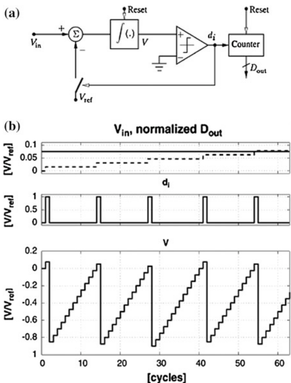
Fig. 5.4 a First-order incremental converter, b Signal waveform ( n_{\text{bit}} = 6 bits, V_{\text{in}} = 0.75V_{\text{ref}} )
