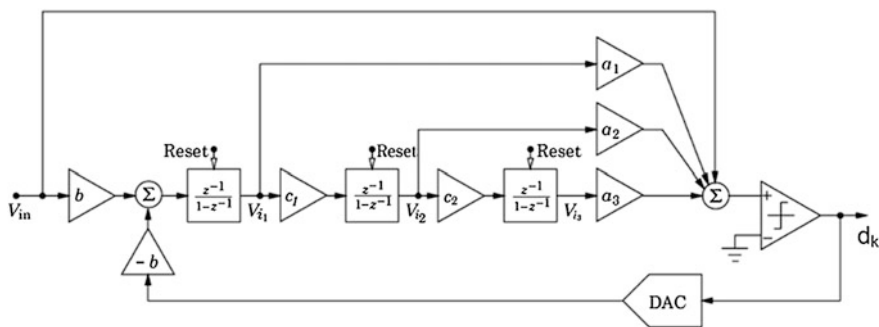
Fig. 5.5 Block diagram of a third-order DR loop
