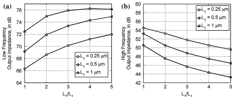
Fig. 3.15 (a) Low-frequency (DC) output impedance ( Z_{CS0} ) and (b) High-frequency output impedance ( Z_{CS} at 100 MHz)
