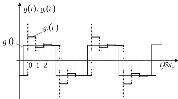
Fig. 9.17 Tracking of the square shape signal s \frac{1}{4} 8
