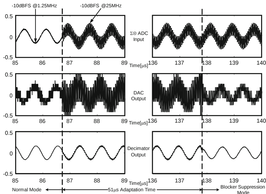
Fig. 2.59 RD ADC measured transient response with 25 MHz interferer applied to the system
