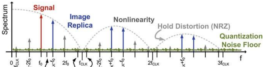
Fig. 3.3 Inherent DAC limitations
