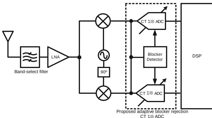
Fig. 2.19 Direct Conversion (DC) receiver architecture with the proposed adaptive blocker rejection CT RD ADC
