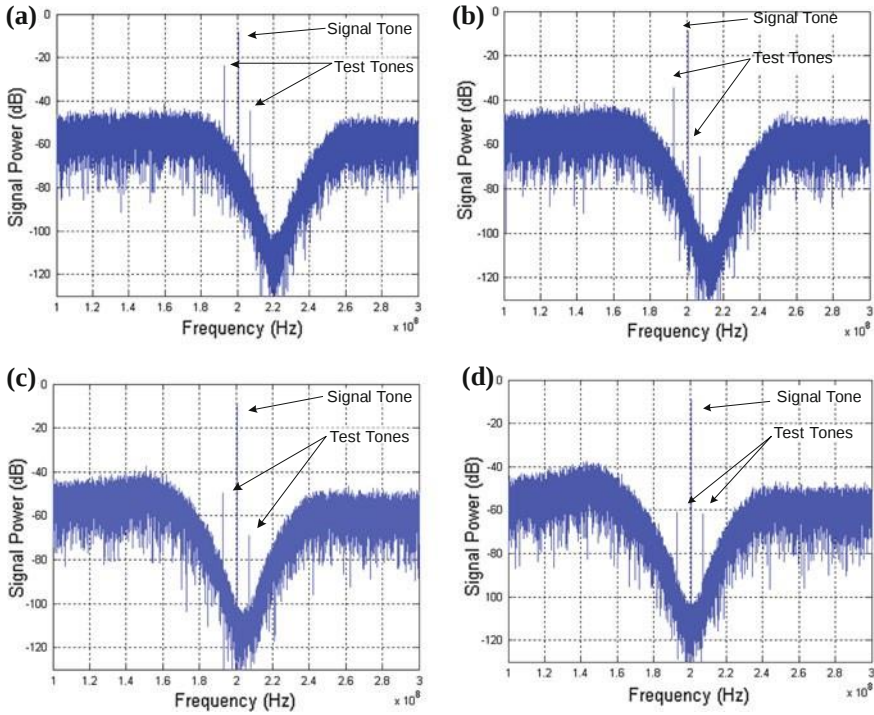
Fig. 4.7 Output spectrum of the 6th order RD modulator with digital calibration scheme vs. the number of iterations of the calibration scheme for 20 % PVT variations on ADC parameters
