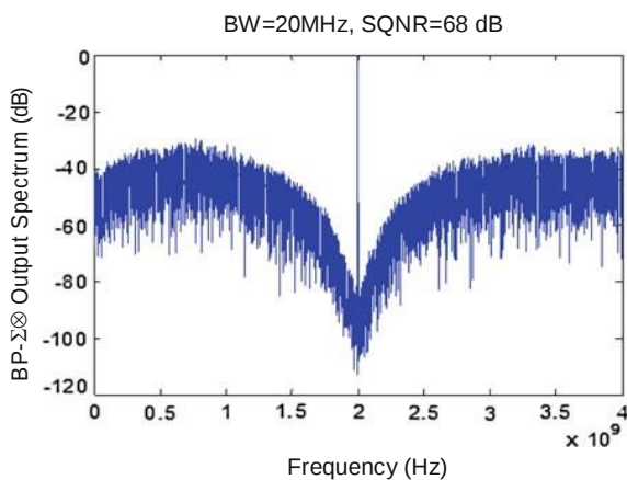
Fig. 4.16 Output Spectrum for F_0 = 2 GHz and F_s = 8 GHz
