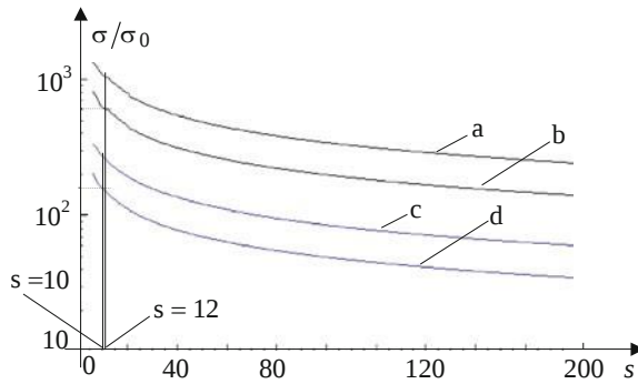
Fig. 9.18 Ratios of the standard deviations to r_0 , D_0 relation to the sampling ratio s in tracking the square signal: a with 12-bit A/D converter; b approximation using the probability distributions of the approximation steps of 12-bit A/D converter; c with 10-bit A/D converter; d approximation using the probability distributions of the approximation steps of 10-bit A/D converter
