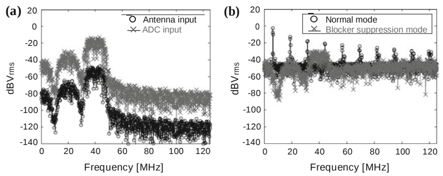
Fig. 2.37 Simulated PSDs of 16-QAM WiMAX signals at a the antenna and ADC inputs and b ADC output
