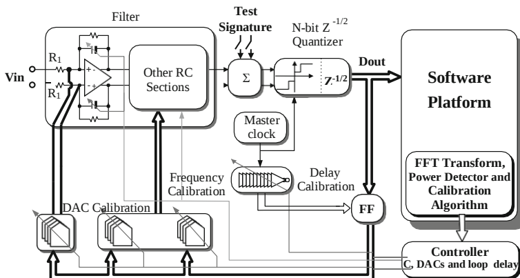
Fig. 4.6 Continuous-time sigma-delta modulator with frequency, excess loop delay and DAC calibration knobs
