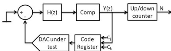
Fig. 12.13 Block diagram of the RD modulator DAC test scheme [32]
