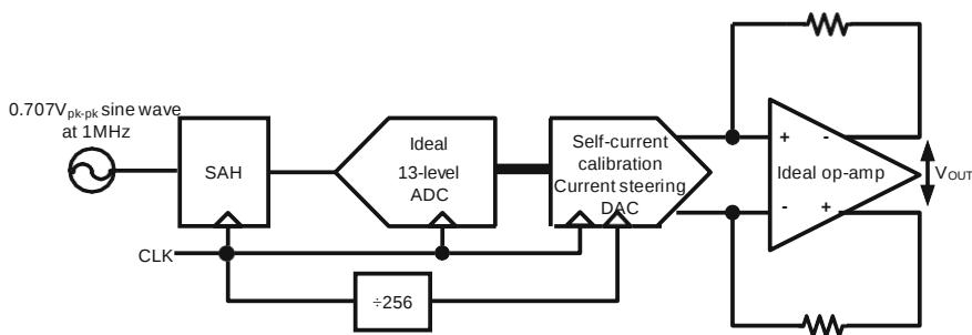
Fig. 2.50 Test setup for estimating performance of the self-current calibration DAC
