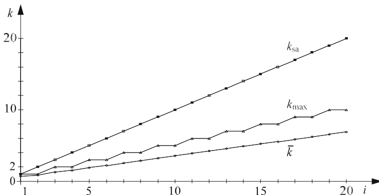
Fig. 9.11 Number of steps of A/D conversions: k_{sa} is a number of steps of the successive-approximation A/D conversion; k_{\max} and \bar{k} are the maximal and the average number of steps of the non-uniform differential A/D conversion
