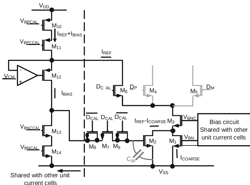
Fig. 2.49 Schematic of the self-current calibration technique
