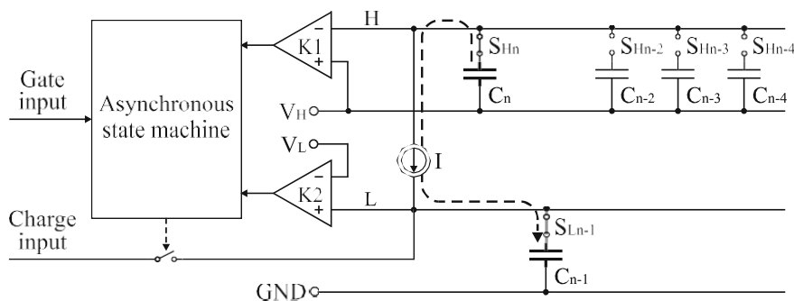
Fig. 6.16 Simplified version of SCR-ADC configuration shown in Fig. 6.15 referring to the first conversion step (compare to Fig. 6.2)
