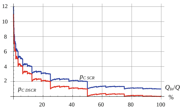
Fig. 6.21 Mean numbers of transfers of a charge unit per conversion cycle versus normalized input charge Q_{in}/Q for the SCR-ADC ( p_{C\_SCR} ) and the DSCR-ADC ( p_{C\_DSCR} ) if n = 12
