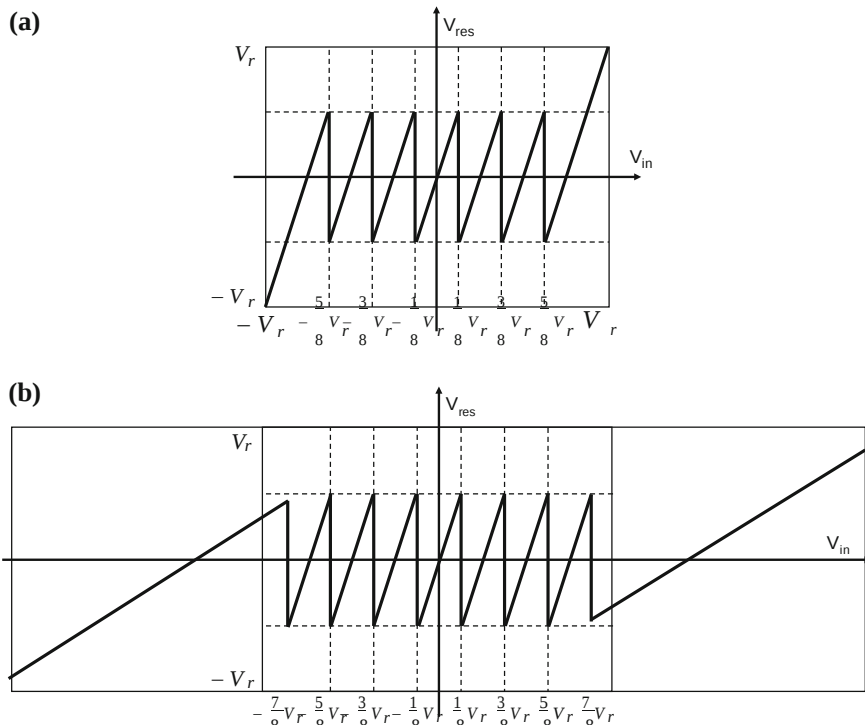
Fig. 1.14 First stage residue amplifier transfer curve: a conventional 2.5b stage, b proposed stage with enlarged input range
