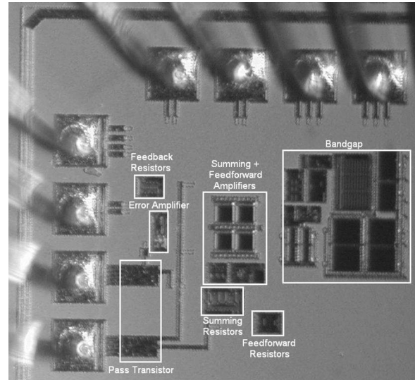
Fig. 20. Chip micrograph of the fabricated LDO with a total active area of 0.049 \text{ mm}^2 including the bandgap circuitry.
