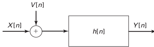
Figure P8.35 LSI system with random signal-plus-noise input.
