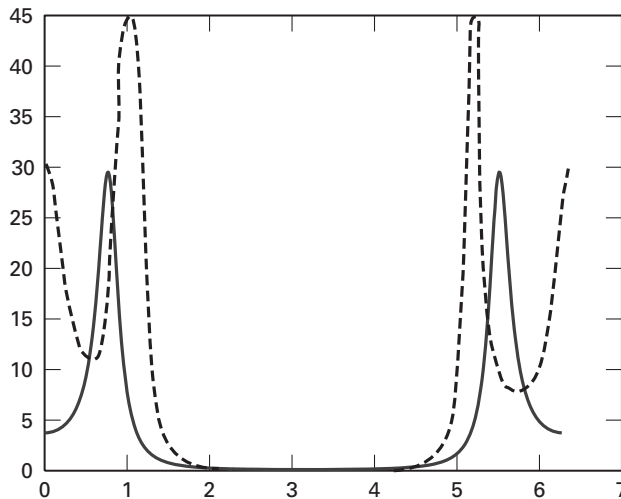
Figure 11.6-8 True (dashed) and MEM2 (solid) psd's for AR(3) model.
