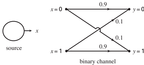
Figure 1.6-4 A binary communication system.
