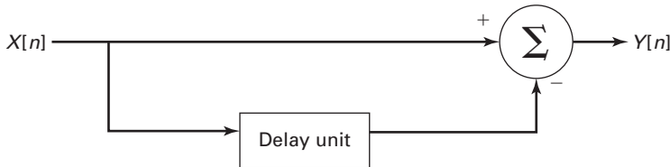
Figure 8.3-1 An edge detector that gives nearly zero output when X[n] \approx X[n-1] and a large output when |X[n] - X[n-1]| is large.
