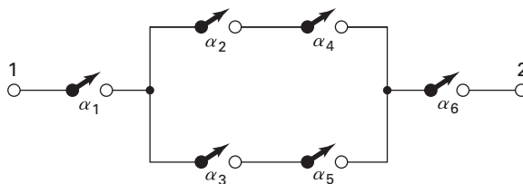
Figure P1.53 Switches in telephone link.
