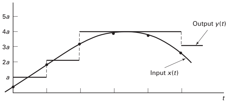
Figure 3.2-10 Quantizer output (staircase function) versus input (continuous line).
