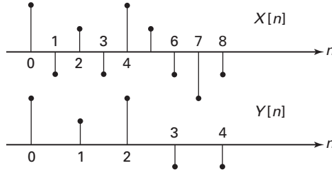
Figure 8.4-2 In decimation every other value of X[n] is discarded.
