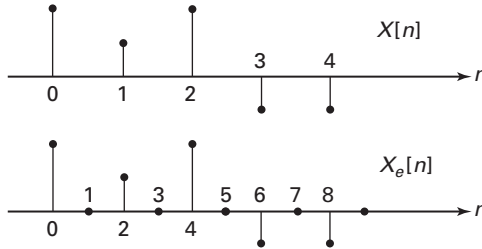
Figure 8.4-3 In interpolation, the expansion step inserts zeros between adjacent values of the X[n] sequence, to get the expanded sequence X_e[n] .
