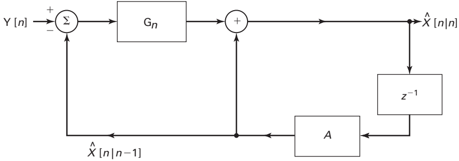
Figure 11.2-3 System diagram of Kalman Filter.
