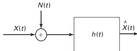
Figure P10.21 Linear estimator of X(t) from signal plus noise observations.
