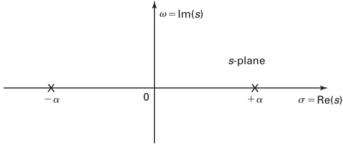
Figure A.3-3 Pole-zero diagram.
