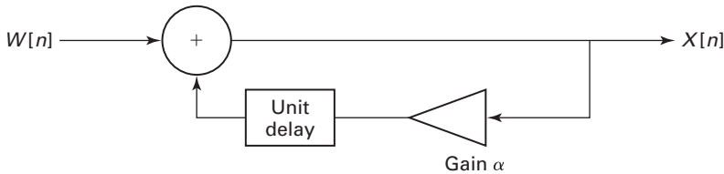
Figure 8.1-5 A feedback filter that generates correlated noise X[n] from an uncorrelated sequence W[n] .
