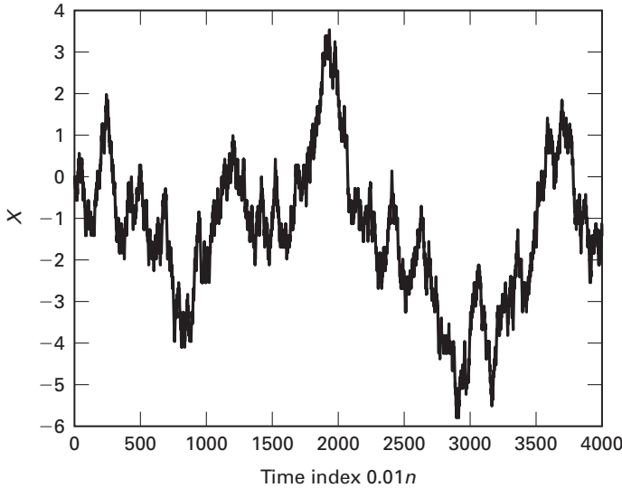
Figure 9.2-7 A Wiener process sample function approximation for \alpha = 1 calculated with T = 0.01 .
