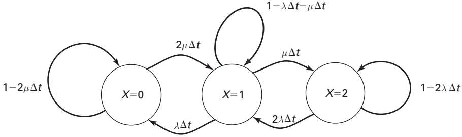
Figure 9.2-8 Short-time state-transition diagram with indicated transition probabilities.
