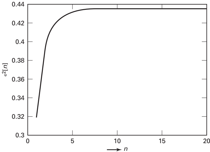
Figure 11.2-4 Prediction-error variance \varepsilon^2[n] .
