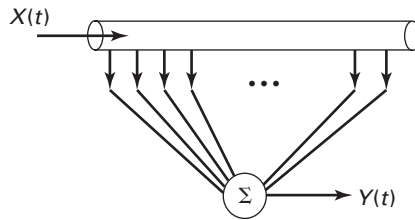
Figure P9.4 Tapped delay-line filter.
