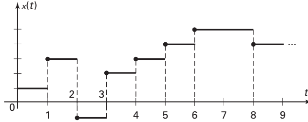
Figure P9.1 Typical output of sample-and-hold D/A converter.
