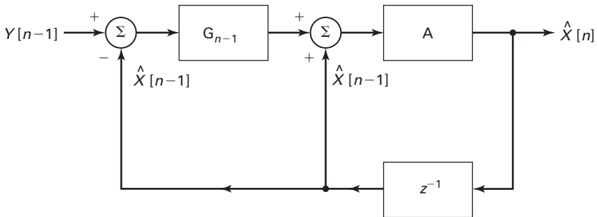
Figure 11.2-2 System diagram of Kalman predictor.
