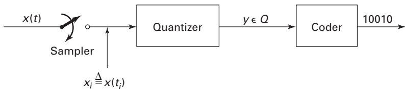
Figure 3.2-9 An analog-to-digital converter.
