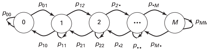
Figure 8.5-5 Markov chain model for M + 1 state communications buffer.
