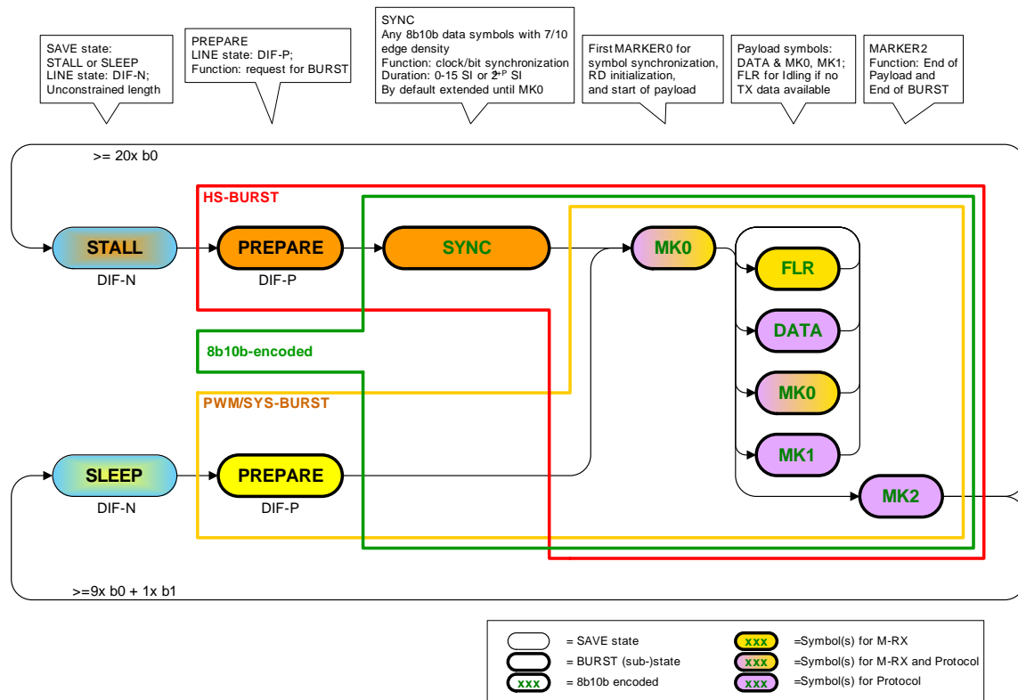
Figure 13 BURST-SAVE: Detailed Sub-FSM
