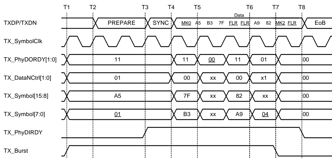
Figure 67 Interface Behavior for HS Transmission with Protocol Layer Throttling Data
