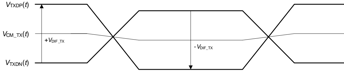
Figure 31 Impact of Output Signal Mismatch on Common-mode Voltage
