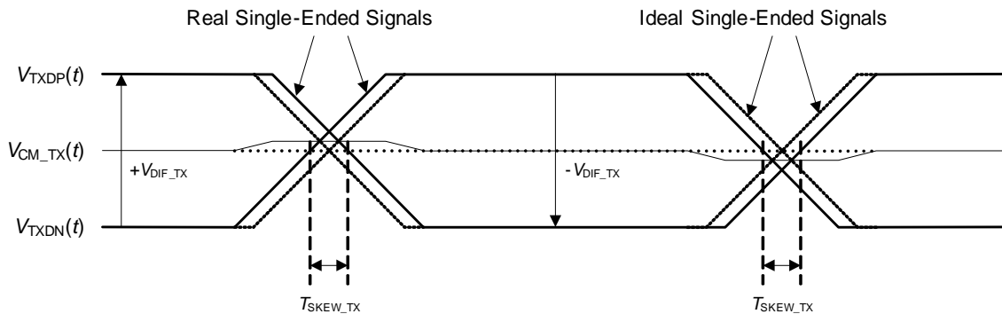
Figure 30 Impact of Signal Skew on Common-mode
