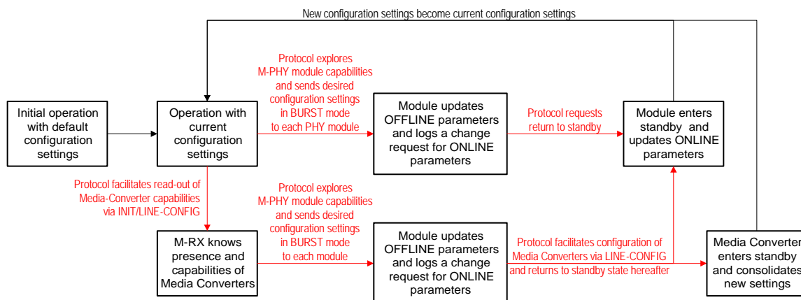
Figure 20 Configuration Flow Diagram
