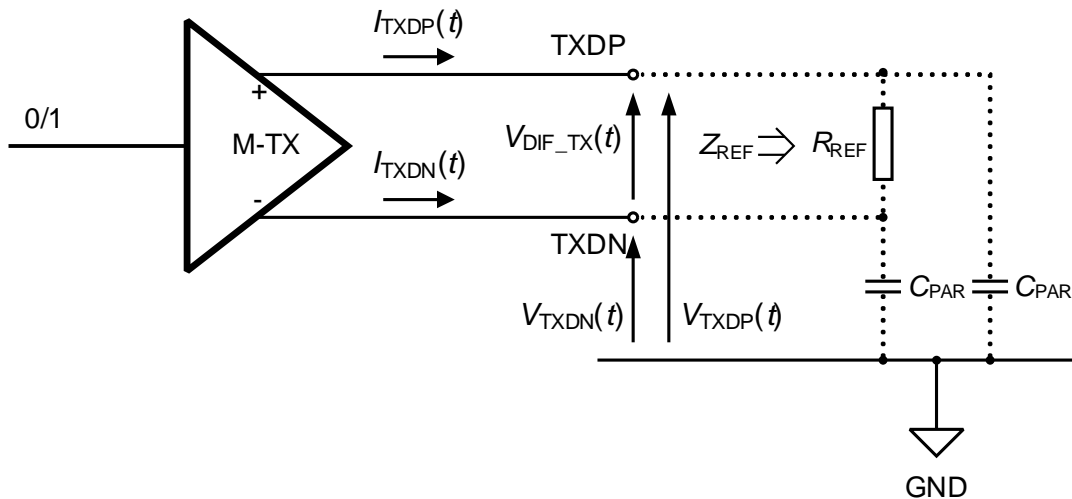
Figure 25 M-TX PIN Voltages, PIN Currents, and Reference Loads
