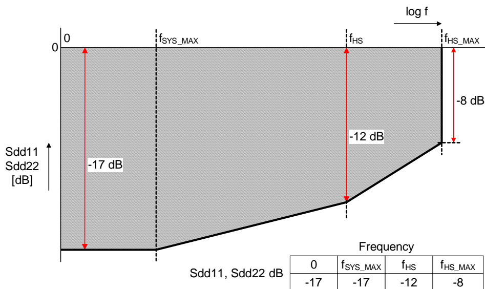
Figure 45 Template for Differential Return Loss at Both Ports
