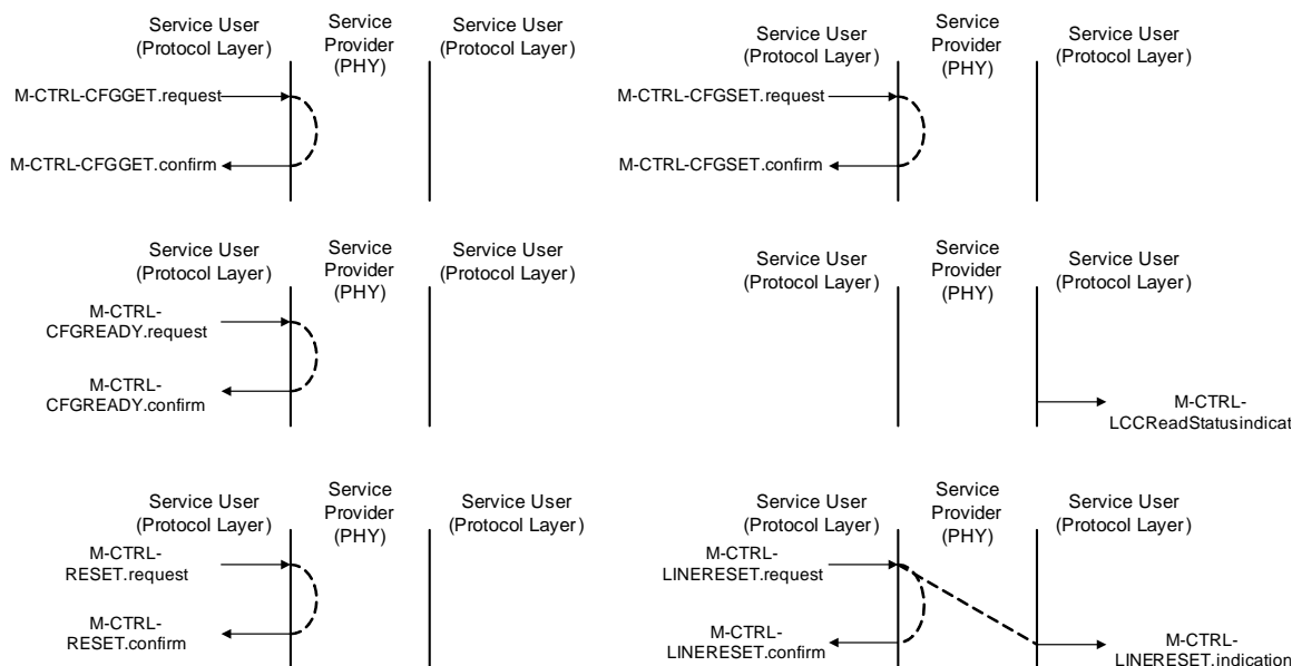
Figure 58 Sequence of Service Primitives at M-TX-CTRL SAP and M-RX-CTRL SAP
