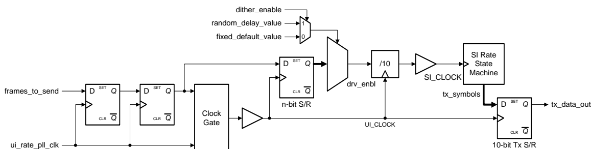
Figure 70 Dithering Circuit Example
