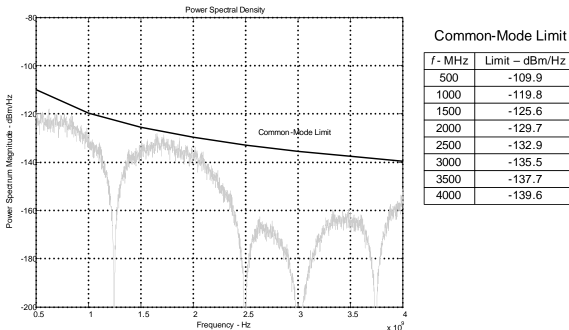
Figure 33 Common-mode Power Spectral Magnitude Limit
