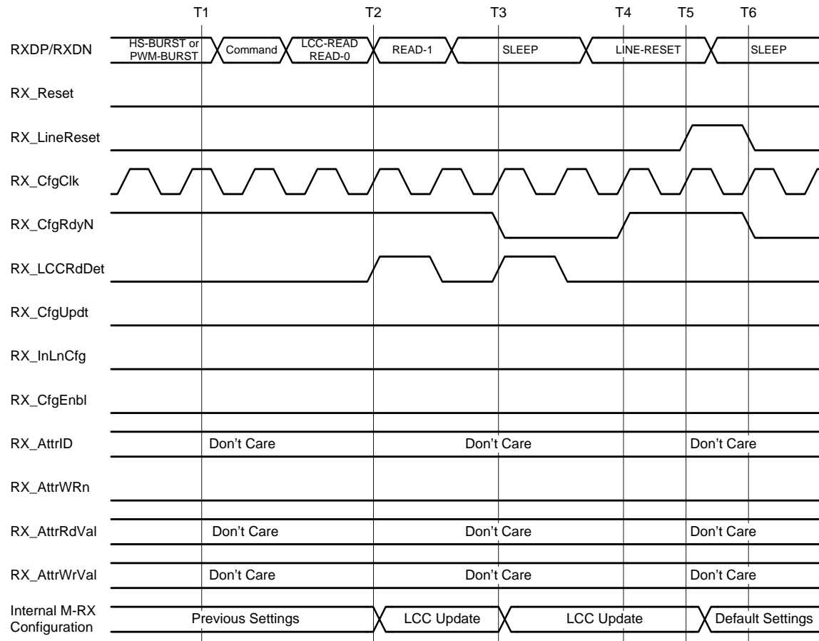
Figure 64 Interface Behavior for LCC Command and LINE-RESET
