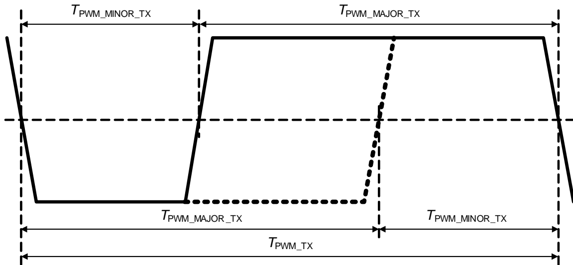
Figure 34 TX Minor and Major Duration in a PWM Signal
