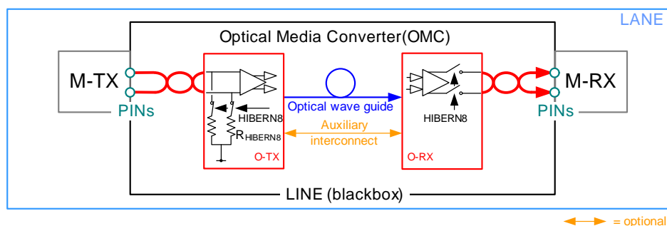
Figure 51 DIF-Z OMC Implementation
