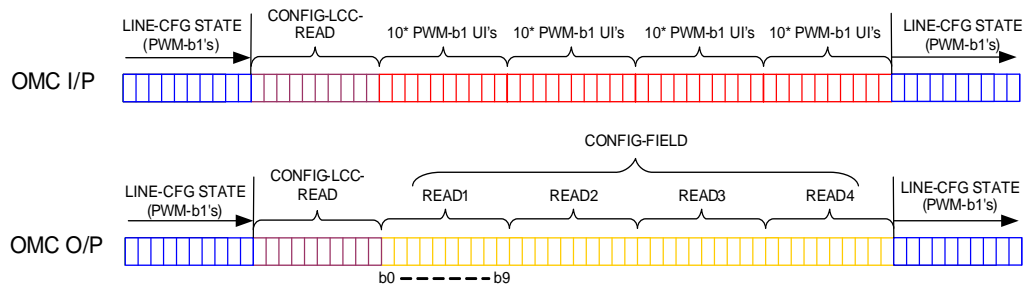
Figure 55 OMC READ Function
