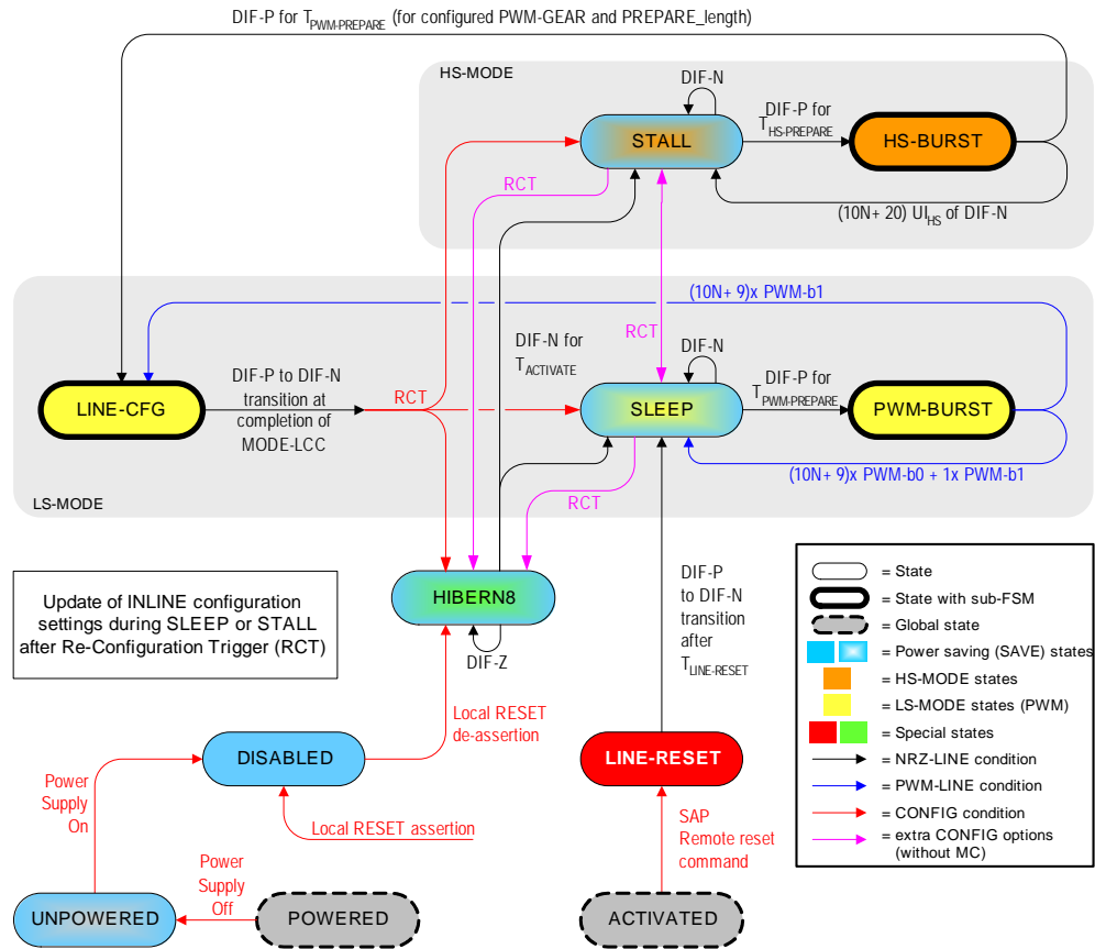
Figure 7 State Diagram for Type-I M-TX MODULES
