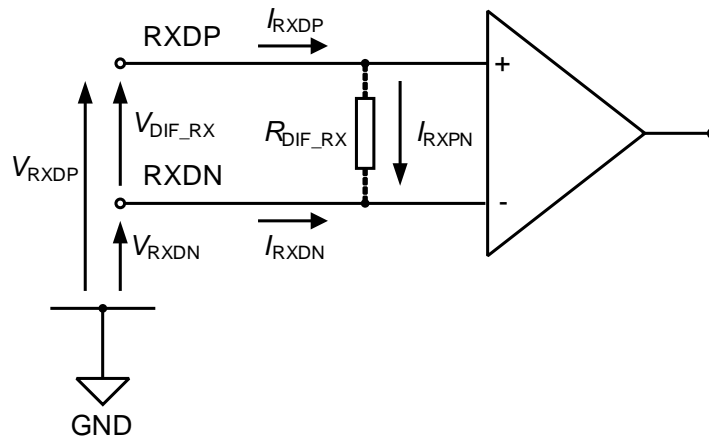
Figure 35 PIN Voltages and PIN Currents of an M-RX
