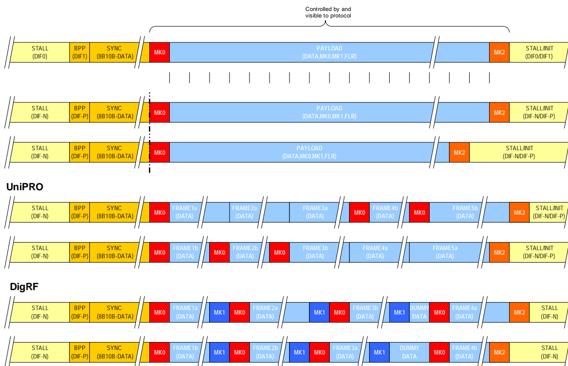
Figure 23 Multilane Operation in UniPro and DigRF
