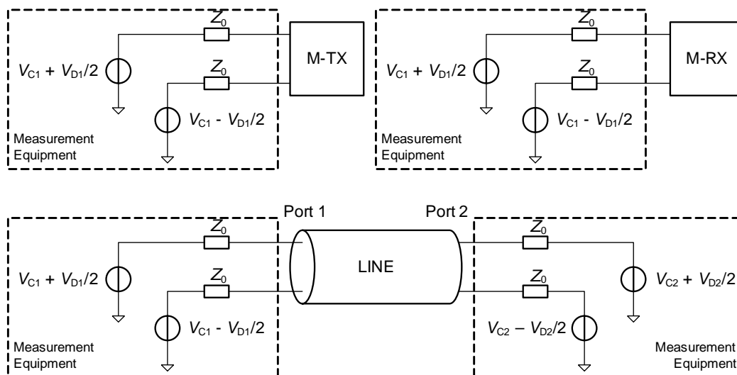
Figure 43 Setup for S-parameter Characterization of M-RX, M-TX, and LINE
