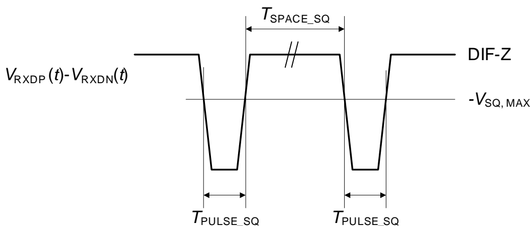
Figure 41 Pulse Rejection and Non-squelch State Detection
