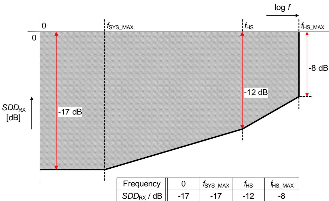
Figure 37 Template for Differential Receiver Return Loss SDD_{\text{RX}}
