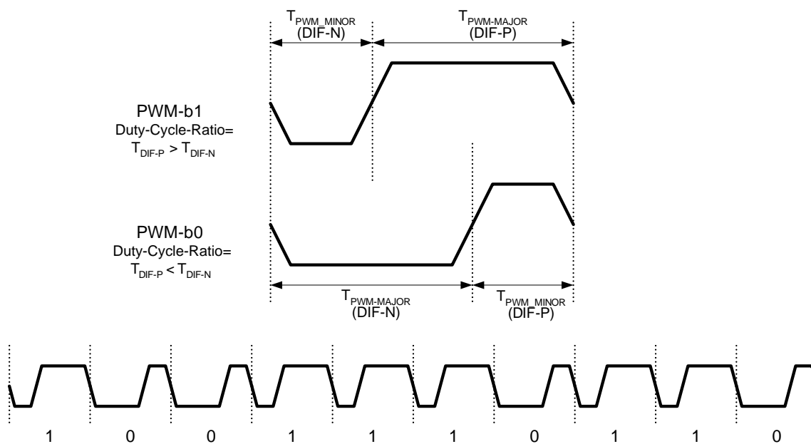
Figure 4 PWM Bit Waveforms and Bit Stream Example
