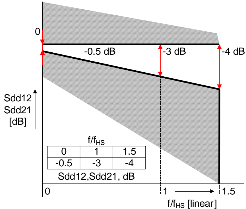
Figure 44 Template for Differential Insertion Loss for HS-GEAR1 and PWM GEARS
