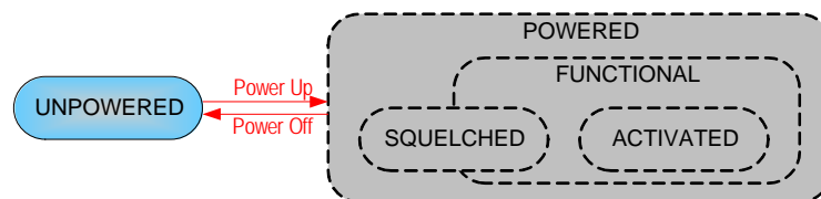
Figure 11 Relationship between Global States
