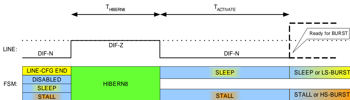
Figure 12 Entry and Exit of HIBERN8
