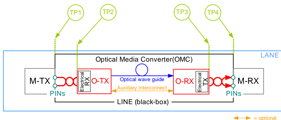
Figure 52 Electrical Specification Test Points
