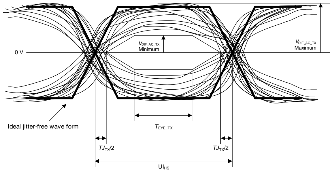
Figure 32 Differential Transmit Eye Diagram
