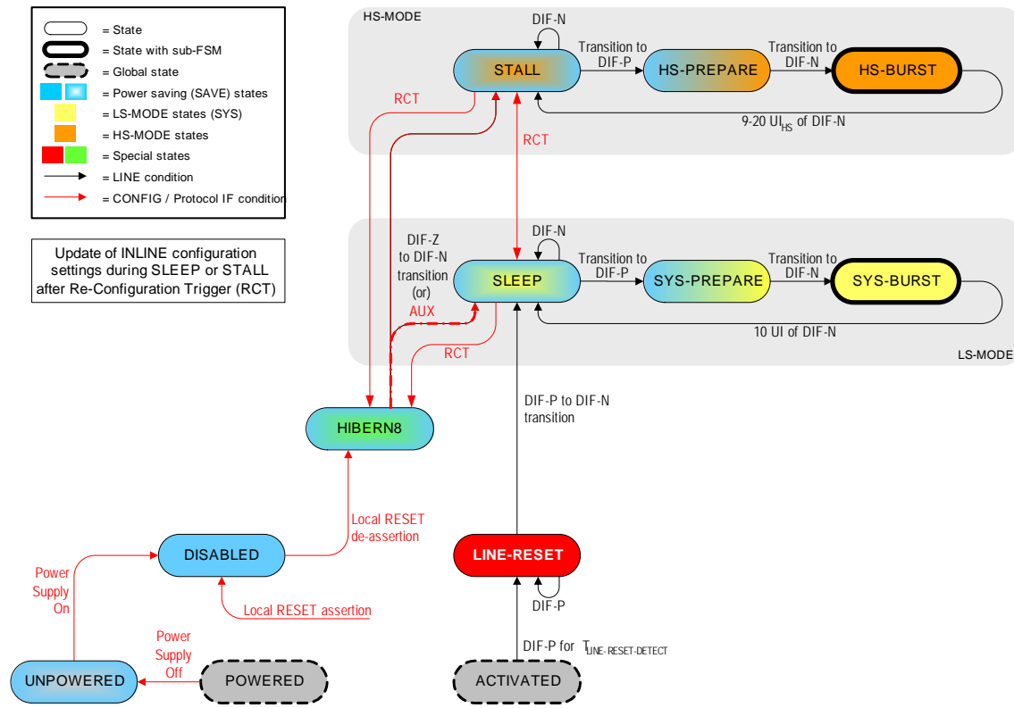
Figure 10 State Diagram for Type-II M-RX MODULEs
