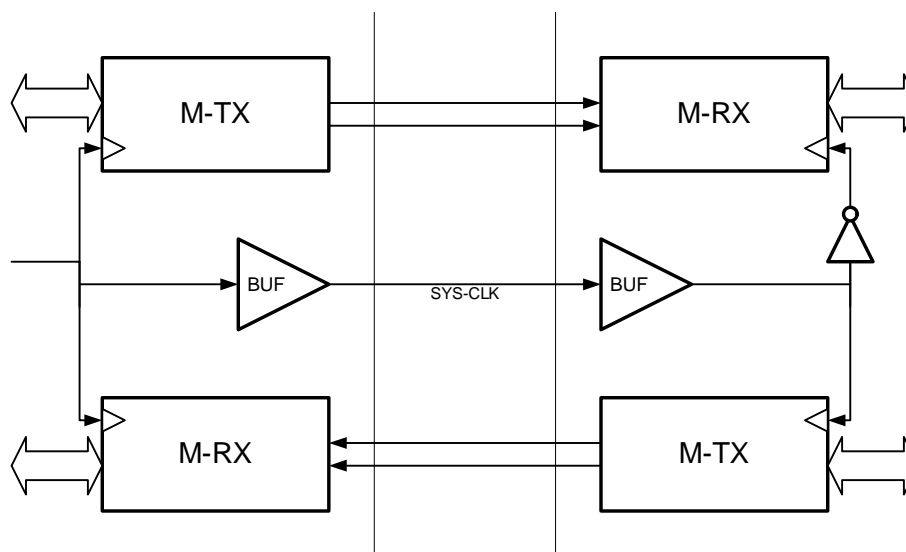
Figure 15 Bidirectional SYS-BURST Clocking Example
