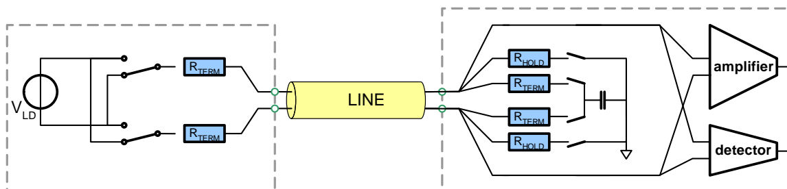
Figure 3 Example I/O Termination
