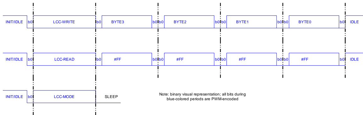
Figure 18 Format of Different LCC Frames on the LINE
