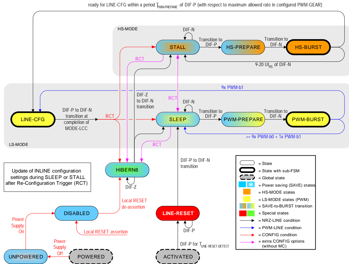
Figure 8 State Diagram for Type-I M-RX MODULEs
