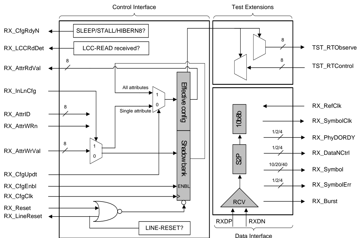
Figure 59 M-RX Signal Interfaces Diagram
