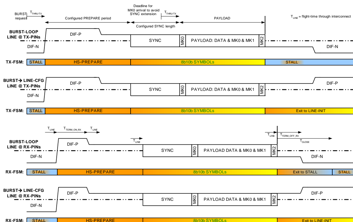
Figure 14 HS-MODE BURST Operation
