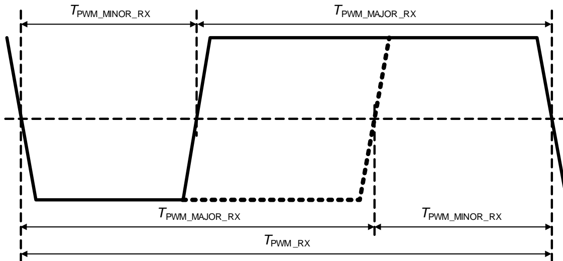
Figure 40 RX Minor and Major Duration in a PWM Signal
