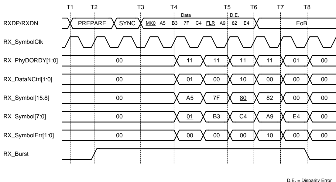
Figure 65 Example 20-bit Interface Behavior for HS Data Reception
