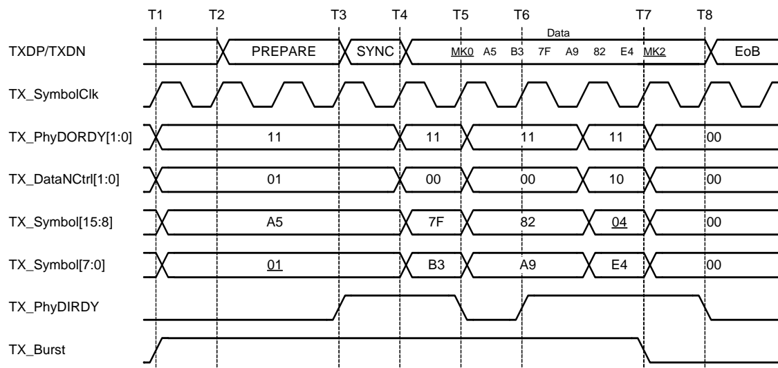
Figure 68 Interface Behavior for HS Transmission with M-TX Throttling Data
