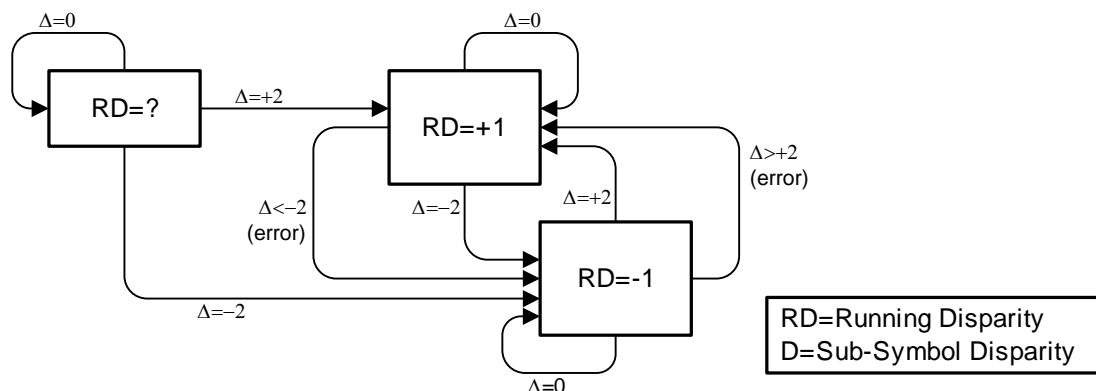
Figure 6 Running Disparity (RD) State Diagram
