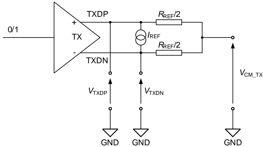
Figure 28 Measurement Setup for Single-ended Output Resistance
