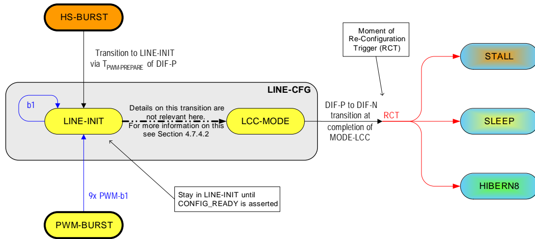
Figure 19 Re-Configuration Trigger after LINE-CFG
