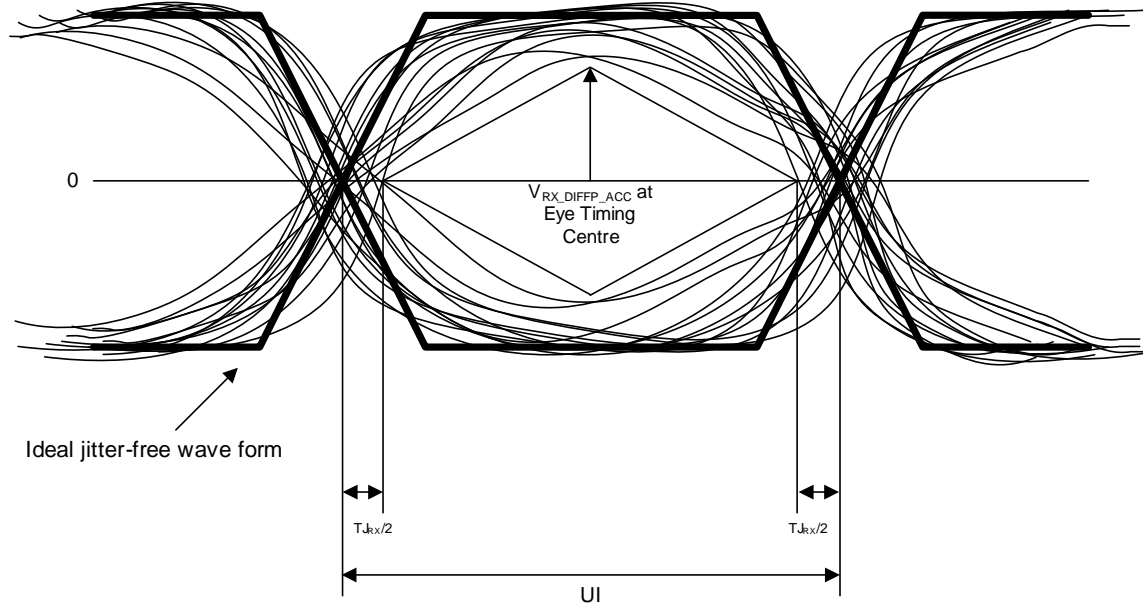
Figure 48 Eye Margins from LINE Simulation Results
