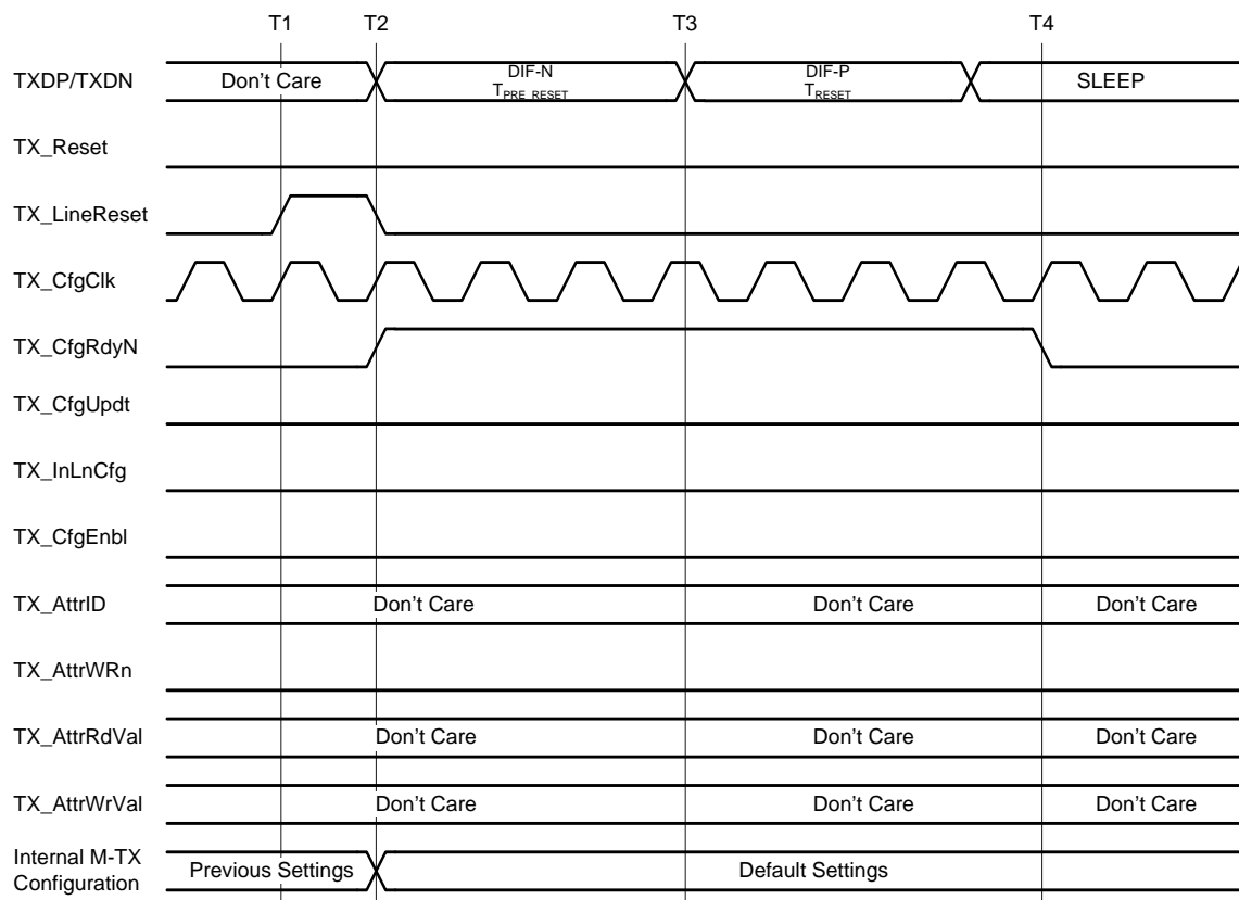
Figure 66 Interface Behavior for a TX_LineReset Command
