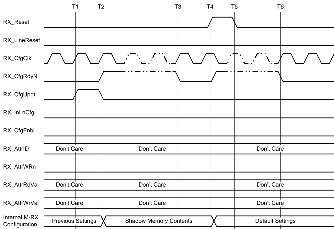
Figure 63 Interface Behavior for RX_CfgUpdt and RX_Reset
