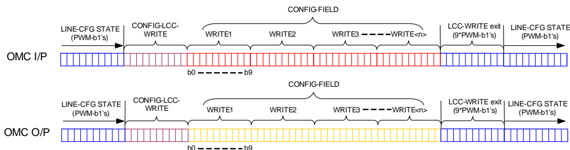
Figure 54 OMC WRITE Function
