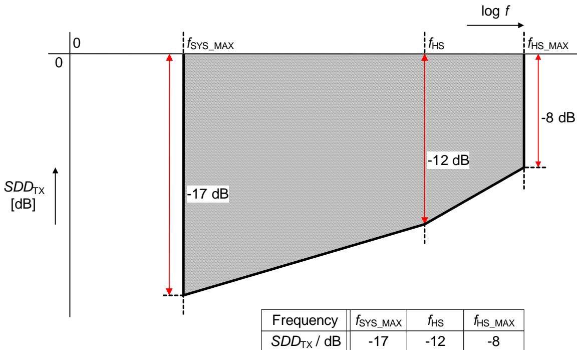
Figure 29 Template for differential Transmitter Return Loss SDD_{\text{TX}}
