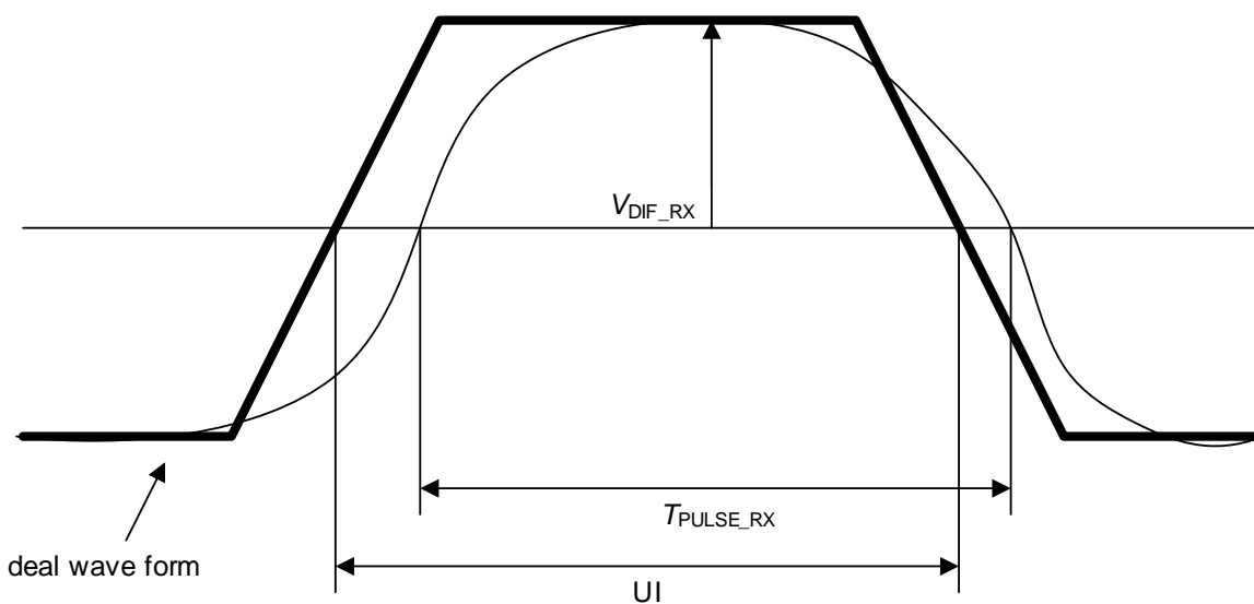
Figure 39 Receiver Pulse Width
