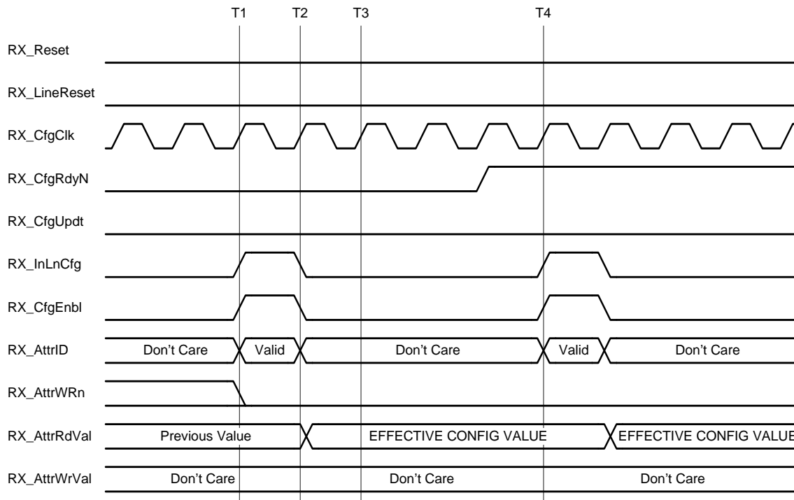
Figure 61 Interface Behavior for Attribute Read Operations
