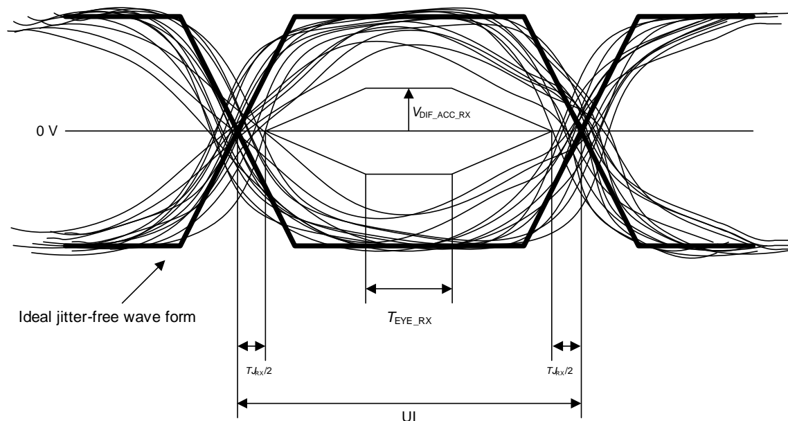
Figure 38 Receiver Eye Diagram
