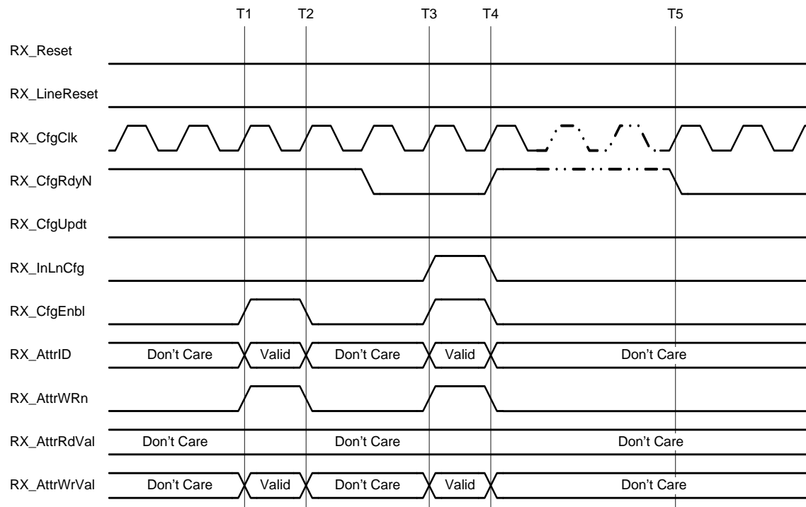
Figure 62 Interface Behavior for Attribute Write Operations
