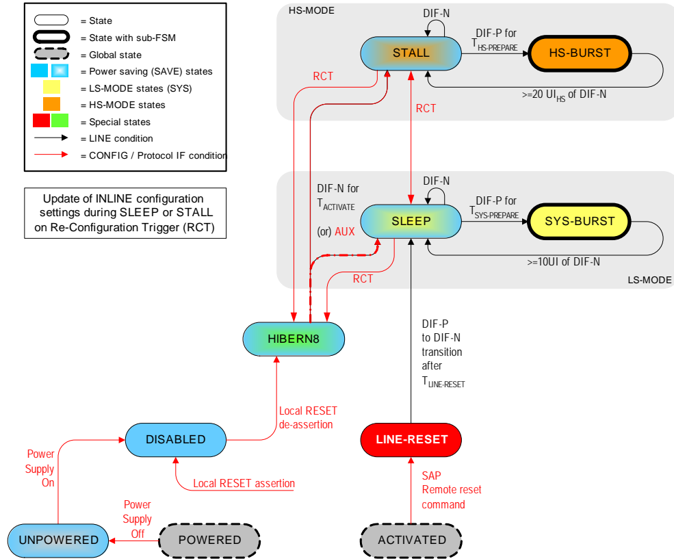
Figure 9 State Diagram for Type-II M-TX MODULES
