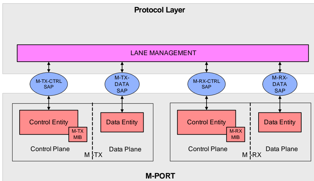
Figure 56 M-PORT Protocol Interface
