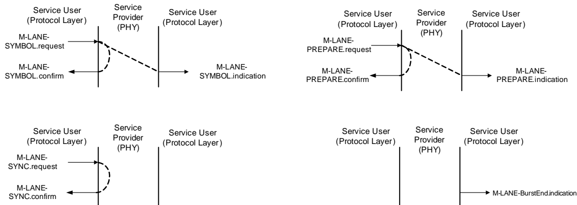
Figure 57 Sequence of Primitives at M-TX-DATA SAP and M-RX-DATA SAP
