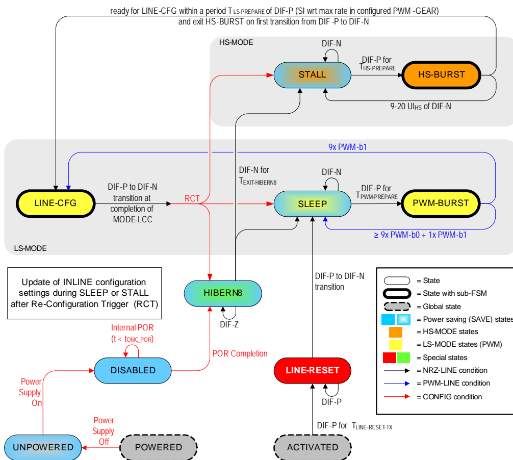
Figure 50 OMC State Diagram (based on Type-I M-RX)
