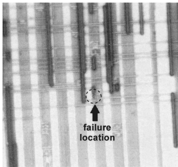
Fig. 18. Typical EMMI picture to show the failure location of ESD damage (indicated by the arrow) on the internal circuits due to pin-to-pin ESD stress.
