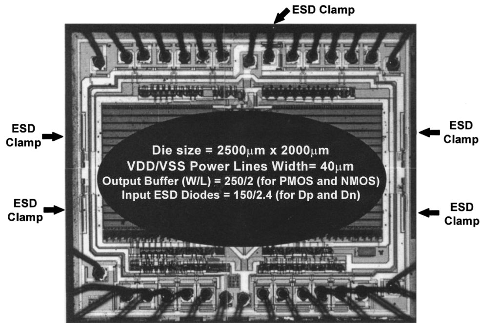
Fig. 19. Microphotograph of a 0.8- \mu\text{m} CMOS IC product using the proposed whole-chip ESD protection design with five VDD-to-VSS ESD clamp circuits (indicated by the arrows).
