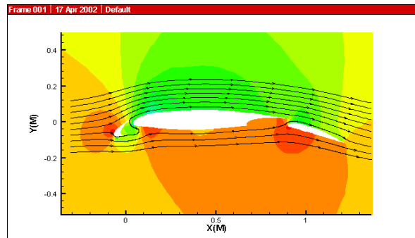
Figure 21-16. A three element airfoil solution.
