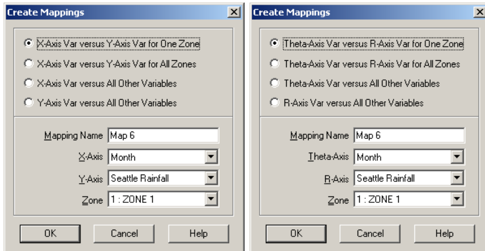
Figure 7-2. Create Mappings dialogs for XY Line plots (left) and for Polar Line plots (right).
