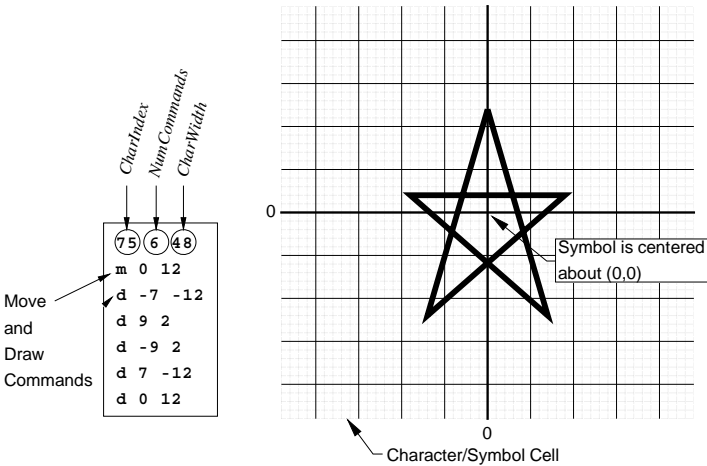
Figure 32-4. Defining a user-defined plotting symbol.
