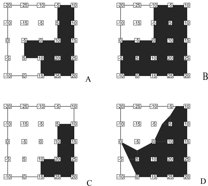
Figure 19-2. The effects of the different value-blanking options in 2D field plots for a constraint where a variable is less than or equal to zero. The dark shading indicates the areas that are not blanked.
