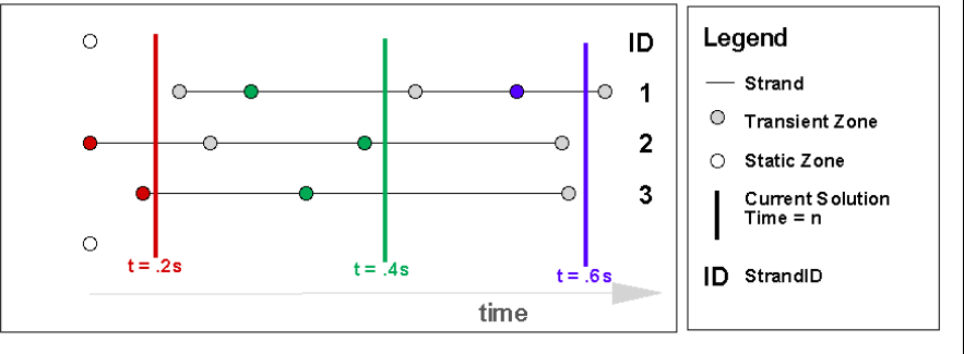
Figure 8-7. An illustration of how relevant zones are determined (based on the data in Table 8 - 1 ). For a given solution time, the relevant zones ONLY are displayed in the plot. NOTE: static zones are always considered as relevant zones.
