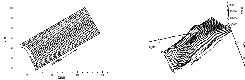
Figure 3-4. Left, a 2D mesh of IJ-ordered data points. Right, a 3D mesh of IJ-ordered data points. NOTE: Ordered axes do not necessarily correspond to physical axes.
