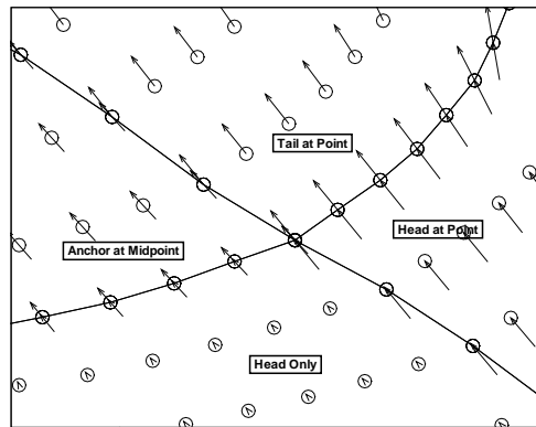
Figure 11-3. The Vector plot types: tail at point, head at point, anchor at midpoint, and head only.
