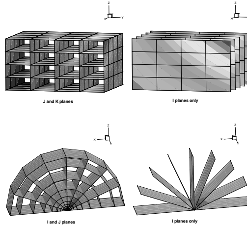
Figure 8-5. Examples of plotting I-, J-, and K-planes.
