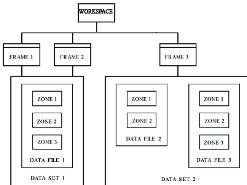
Figure 2-1. Data Hierarchy in Tecplot 360. Frames 1 & 2 share Data Set 1, and Data Set 1 contains 3 zones from 1 data file. Frame 3 contains data set 2, which is composed of 5 zones (2 from data file 2 and 3 from data file 3).
