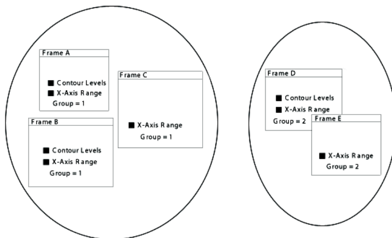
Figure 2-3. Five frames in two groups with different linking options.
