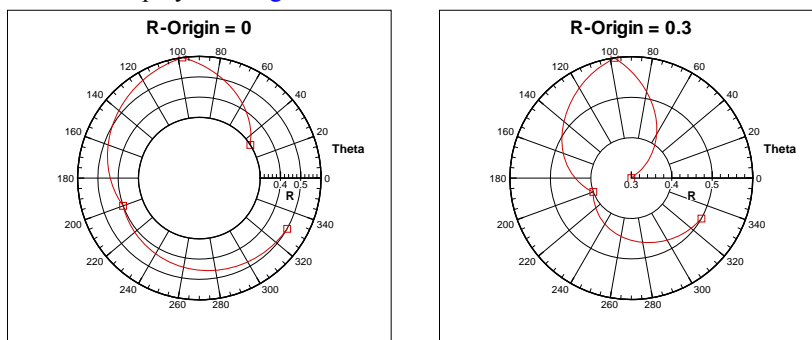
Figure 18-4. An example of changing the R-origin on a polar plot
