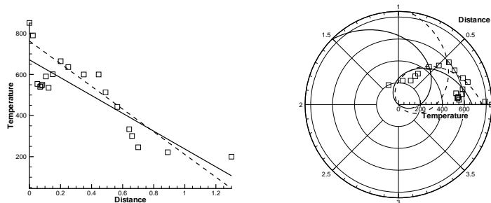
Figure 7-6. Weighted linear fits.
