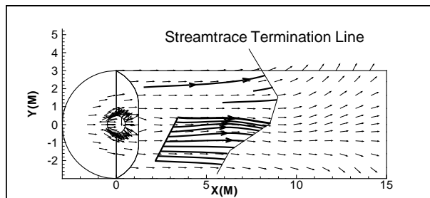
Figure 16-2. A streamtrace termination line drawn through surface streamlines (created with demo file cylinder.plt ).
