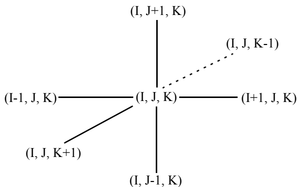
Figure 3-2. IJK-ordered data point neighbors.
