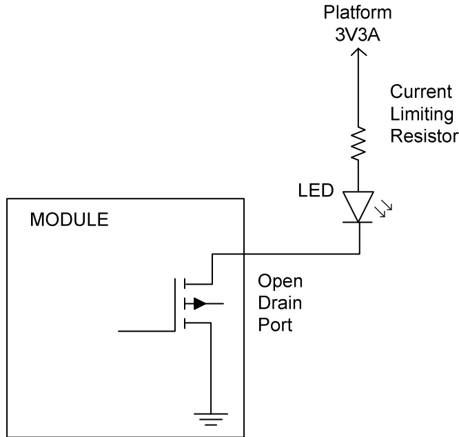
Figure 85. Typical LED Connection in Platform/System
