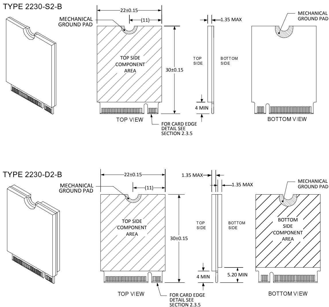
Figure 10. M.2 Type 2230 Mechanical Outline Diagram Examples
