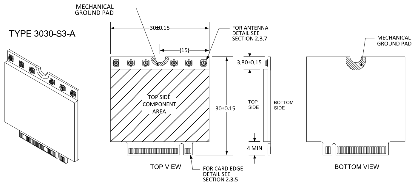
Figure 8. M.2 Type 3030 Mechanical Outline Diagram Example
