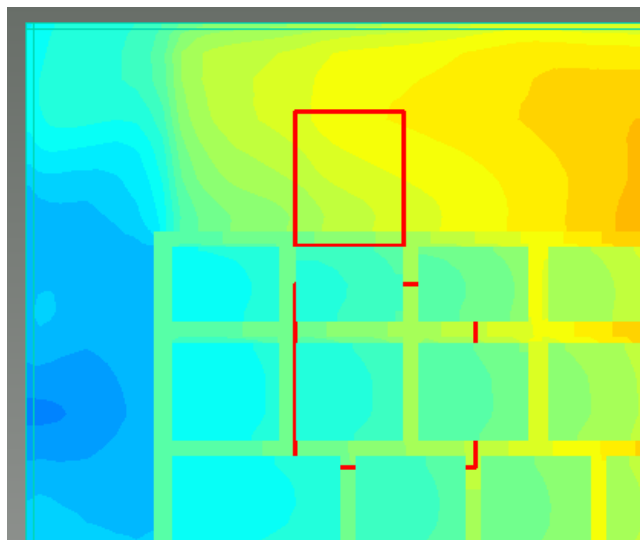
Figure 104. Example View of Hot Spot Over Modules
