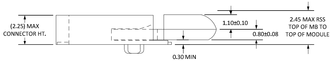
Figure 37. H2.3-S1 - Stack-up Top Mount Single-Sided Module for 1.2 Maximum Component Height
