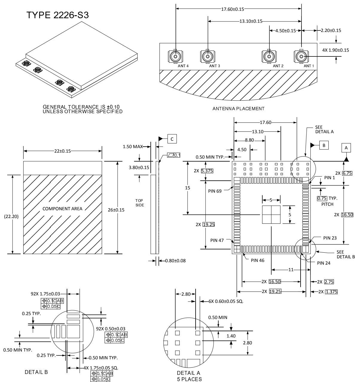
Figure 22. M.2 Type 2226-S3 Mechanical Outline Drawing
