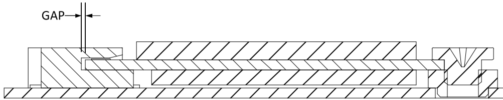
Figure 70. Screw Guidelines
