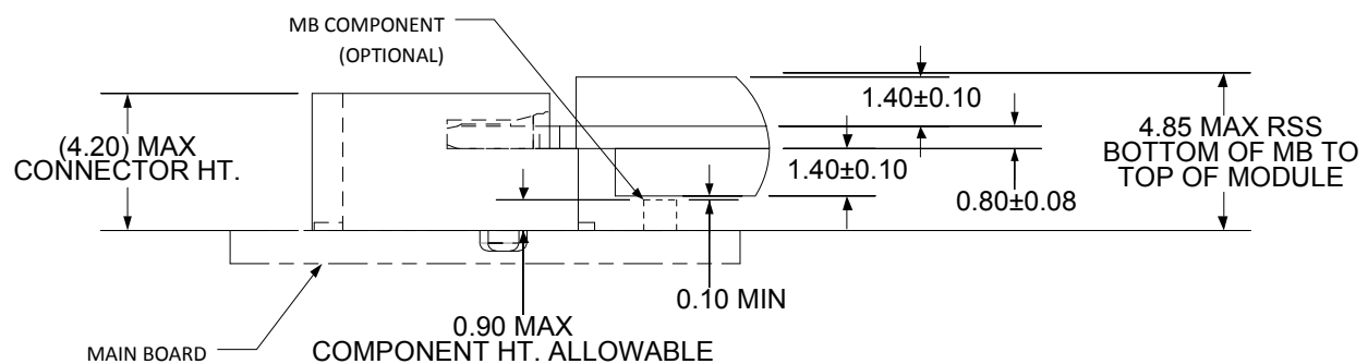
Figure 47. H4.2-D5 - Stack-up Top Mount Double-sided Module for 1.5 Maximum Top-side Component Height with 1.5 Maximum Bottom-side Component Height
