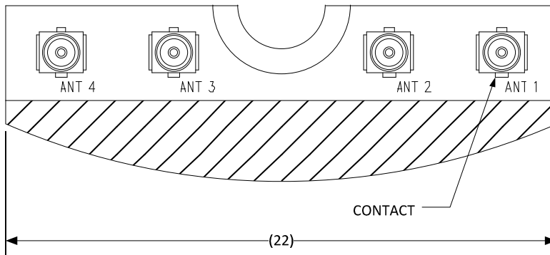
Figure 26. Board Type 2230 Antenna Connector Designation Scheme
