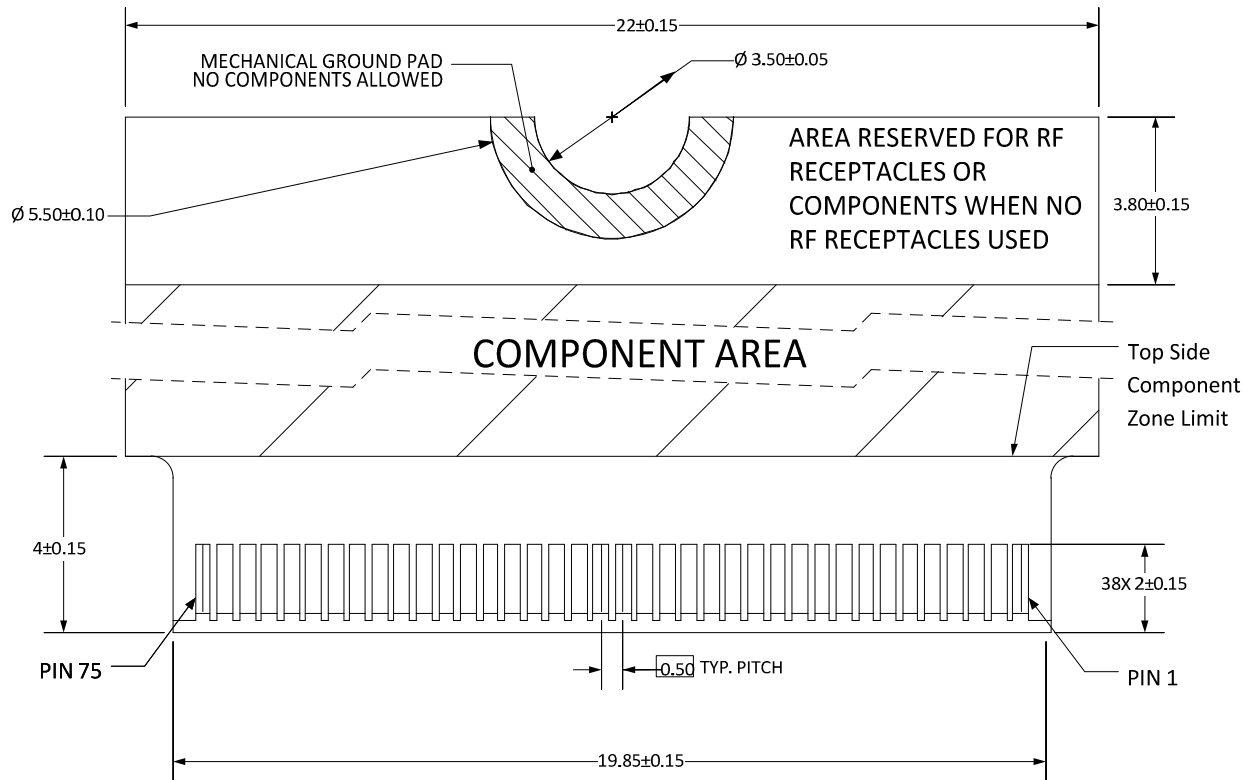
Figure 16. Card Edge Outline-Topside
