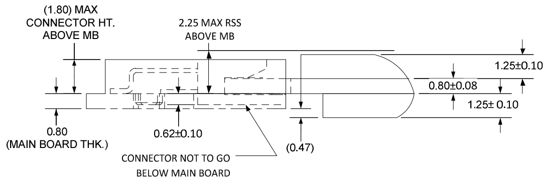
Figure 55. Stack-up Mid-Line (In-line) Double-sided (D2) Module for 1.35 Maximum Top-side Component Height
