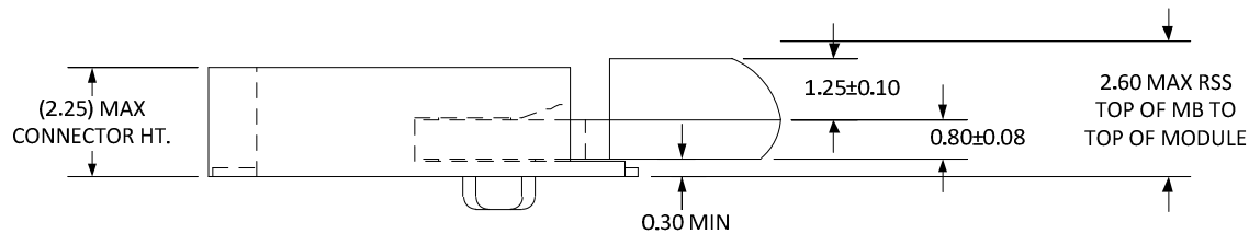
Figure 38. H2.3-S2 - Stack-up Top Mount Single Sided Module for 1.35 Maximum Component Height
