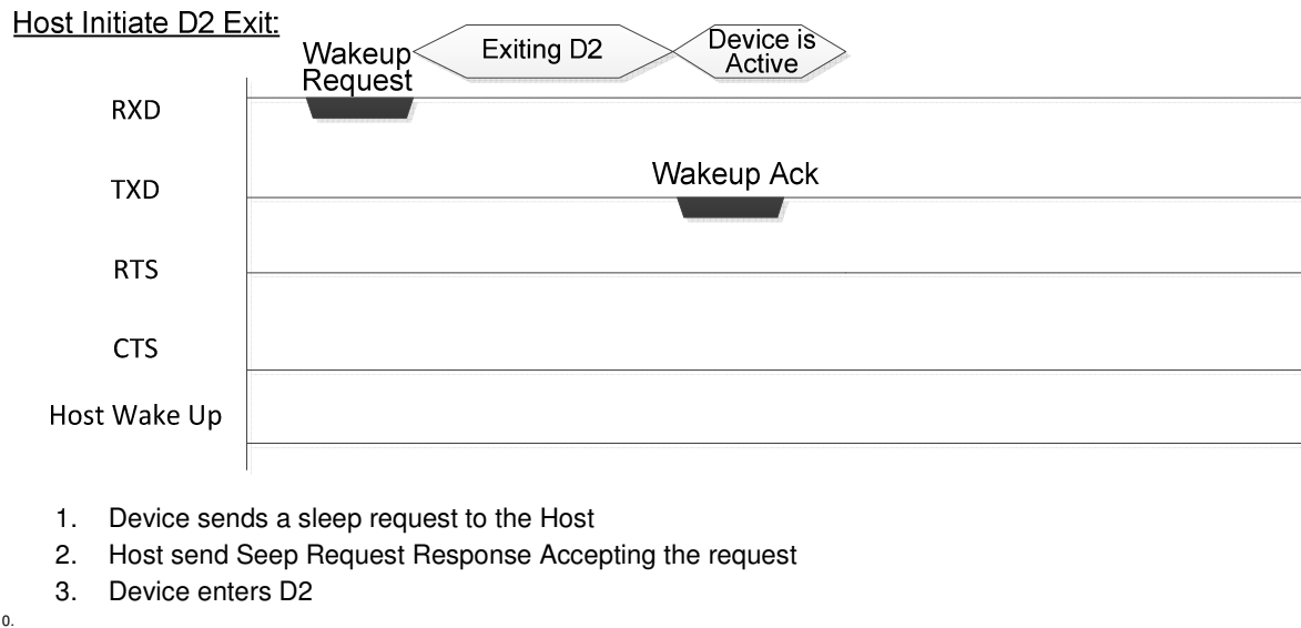
Figure 81. Sleep Request Initiated by the Device
