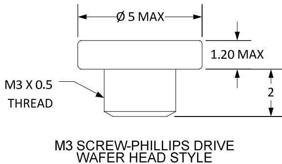
Figure 71. Wafer-Head Style M3 Screw
