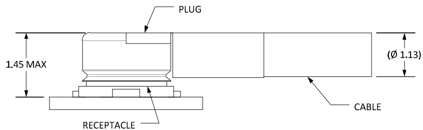
Figure 28. Mated Plug for Ø 1.13 mm Coax Cable
