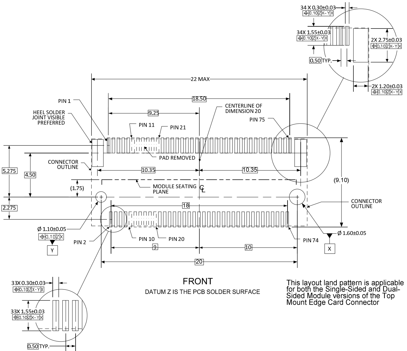
Figure 48. Example of Top Mount MB Land Pattern Diagram Key B Shown
