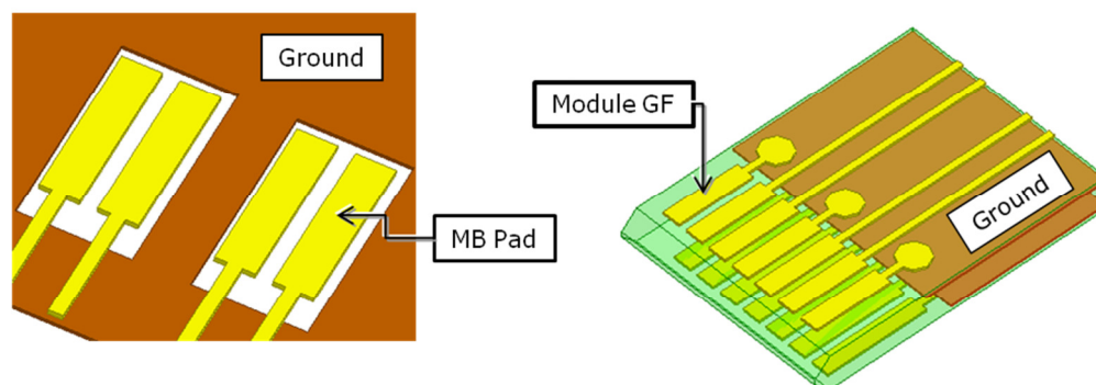
Figure 96. Suggested Motherboard and Module Board Signals and Ground Pad Layout Guideline
