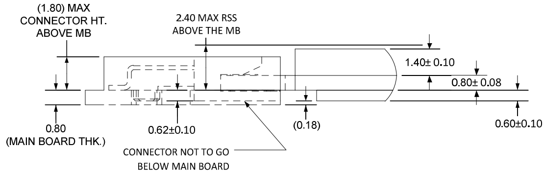
Figure 56. Stack-up Mid-Line (In-line) Double-sided (D4) Module for 1.5 Maximum Top-side Component Height
