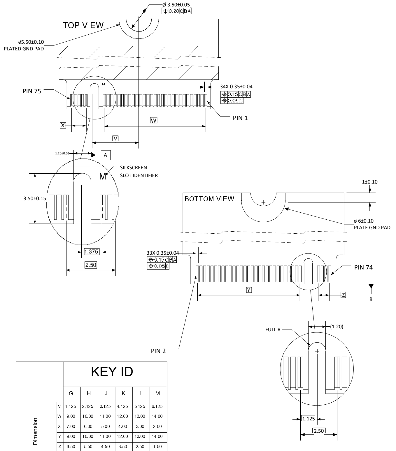
Figure 19. Key Detail for Keys G Thru M
