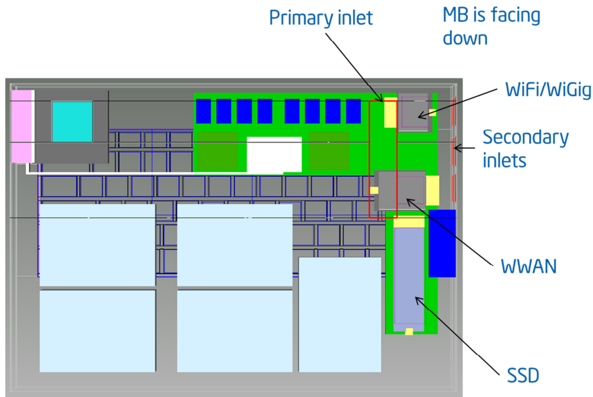
Figure 106. Thin Platform Notebook Layout with Vents and Key Components
