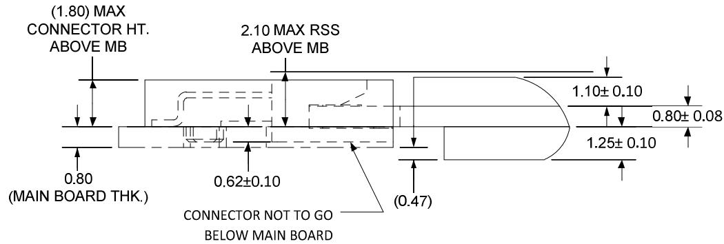
Figure 54. Stack-up Mid-Line (In-line) Double-sided (D1) Module for 1.2 Maximum Top-side Component Height
