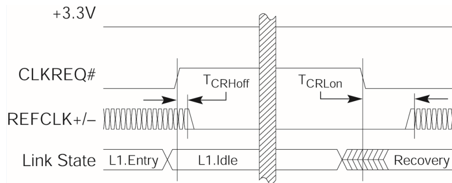
Figure 76. CLKREQ# Clock Control Timings
