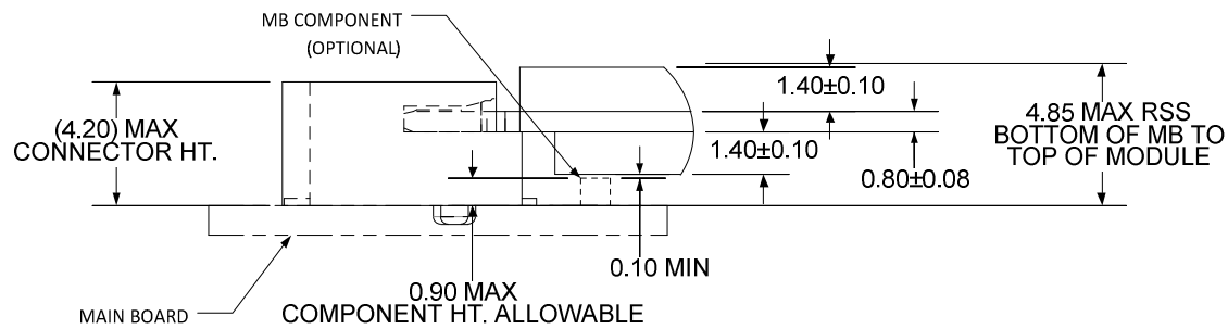
Figure 67. Elevated Double-sided Top Mount Solder Down Stand-off
