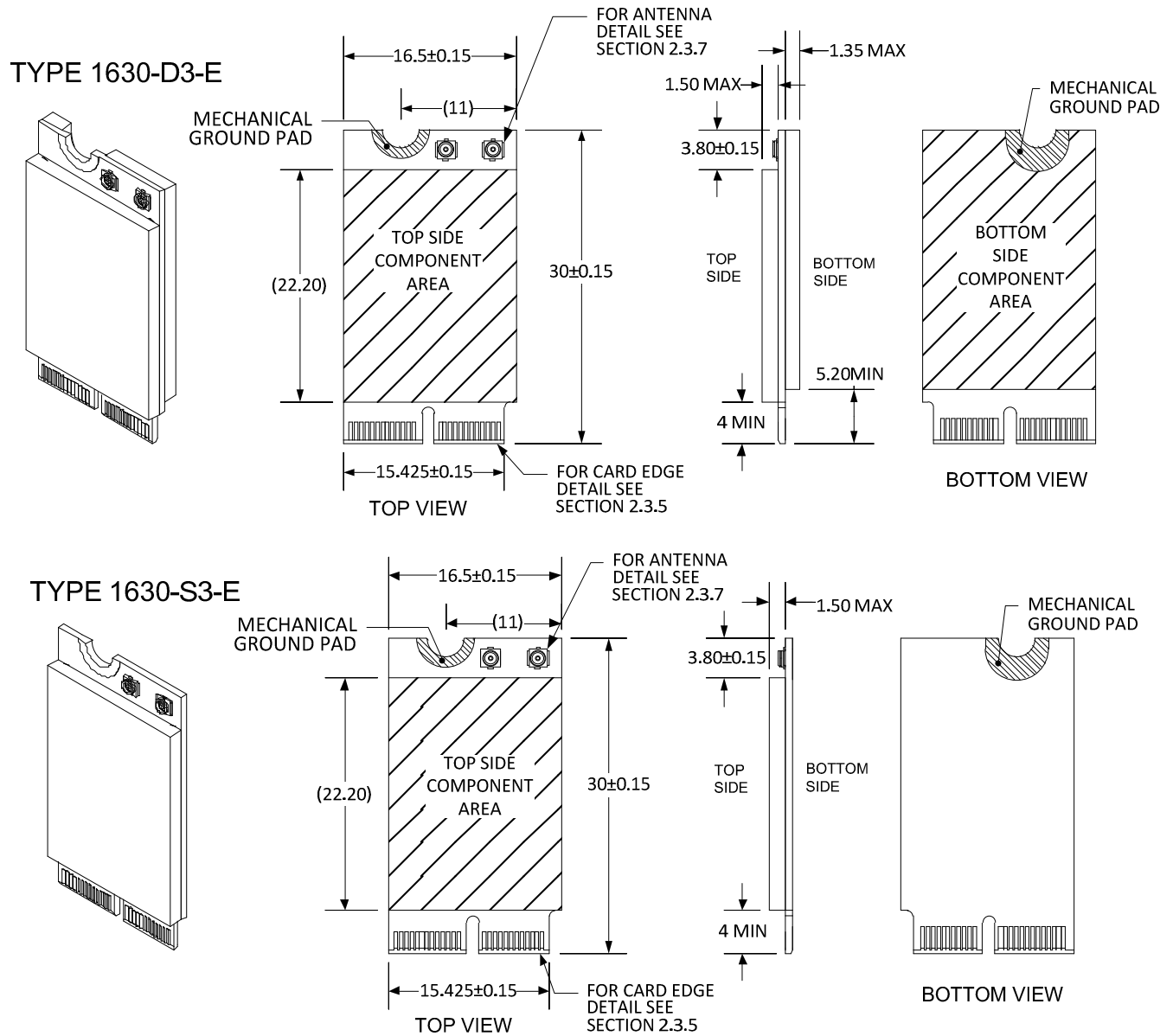
Figure 7. M.2 Type 1630-D3/S3 Mechanical Outline Diagram Examples
