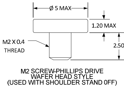
Figure 73. Wafer-Head Style M2 Screw
