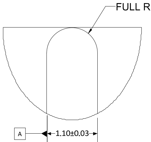
Figure 59. Connector Key
