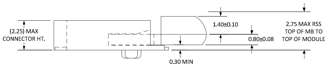
Figure 39. H2.3-S3 - Stack-up Top Mount Single Sided Module for 1.50 Maximum Component Height
