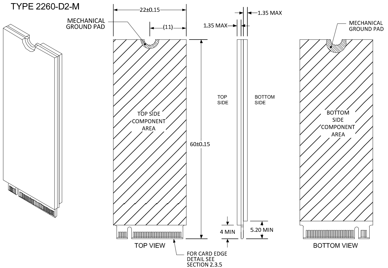
Figure 12. M.2 Type 2260 Mechanical Outline Drawing Example
