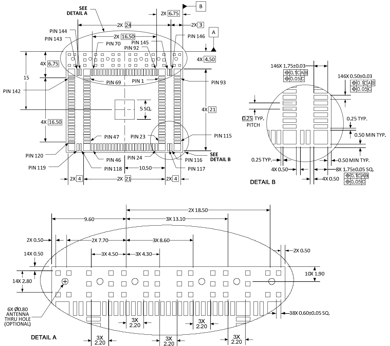
Figure 25. M.2 Type 3026-S3 Mechanical Outline Drawing Details
