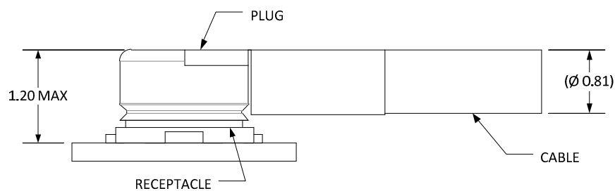
Figure 29. Mated Plug for Ø 0.81 mm Coax Cable
