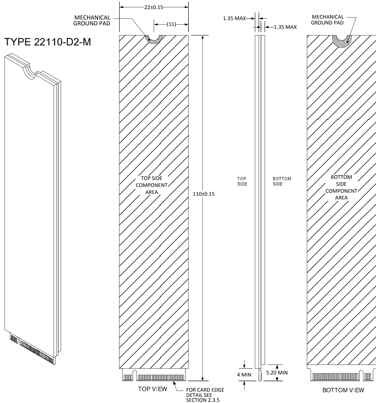
Figure 14. M.2 Type 22110 Mechanical Outline Drawing Example
