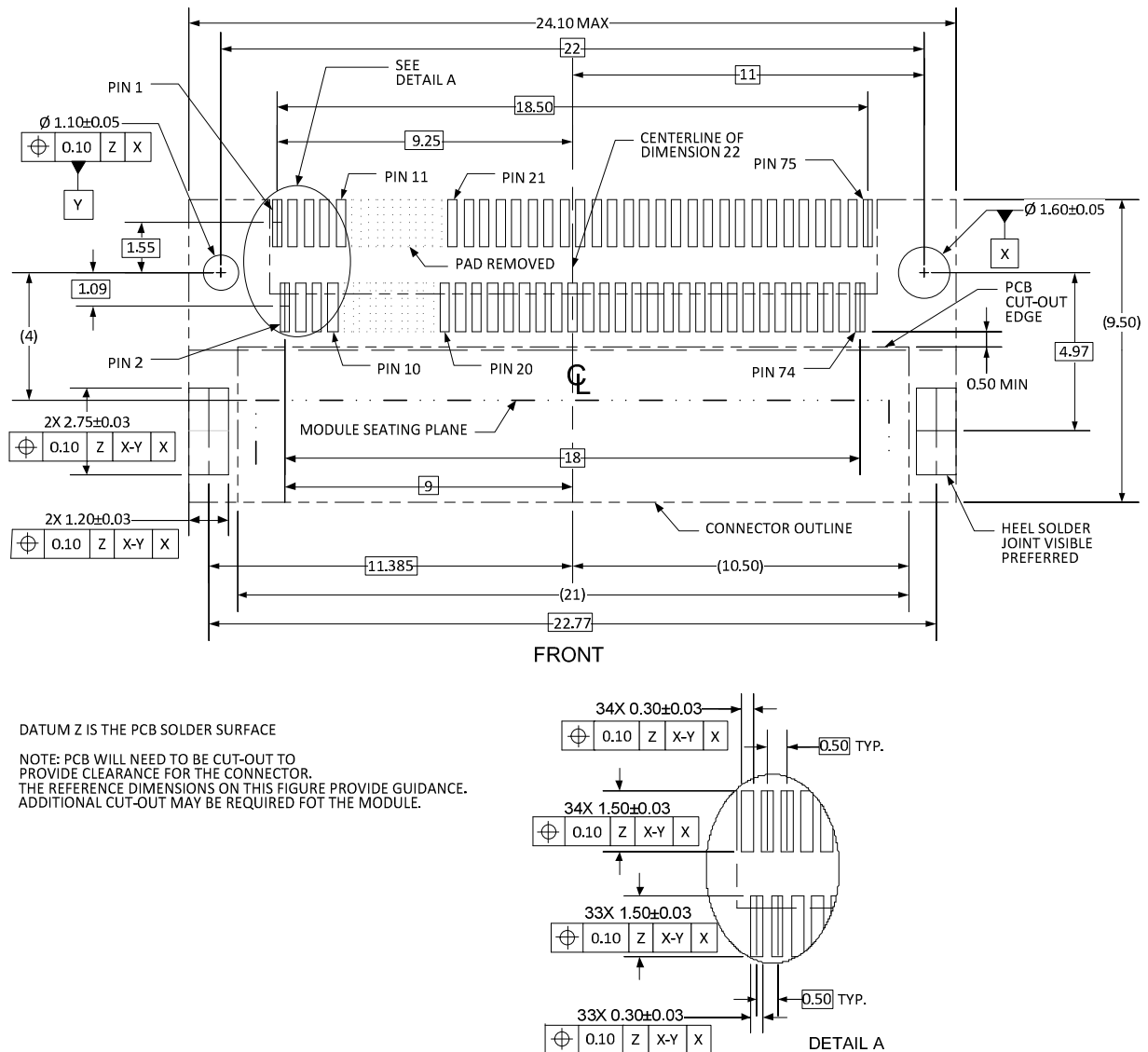
Figure 58. Example of Mid Line MB Land Pattern Diagram – Key B Shown
