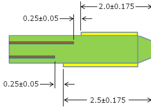
Figure 97. Suggested Ground Void for Module Simulation
