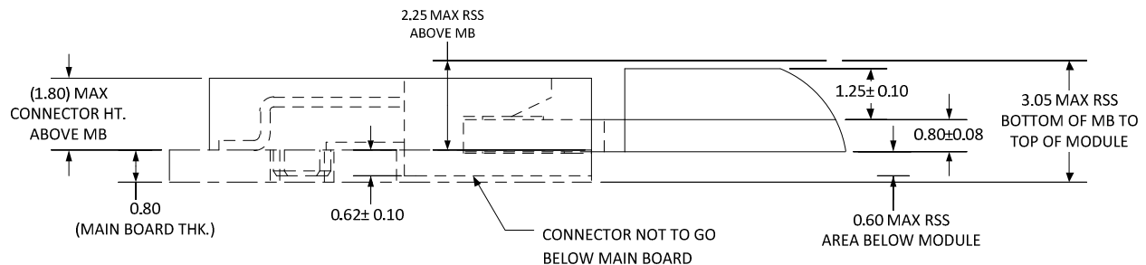
Figure 52. Stack-up Mid-Line (In-line) Single Sided Module for 1.35 Maximum Component Height
