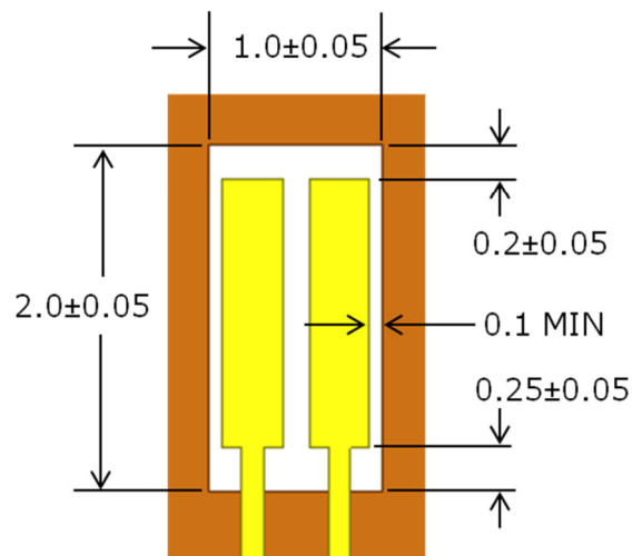
Figure 98. Suggest Ground Void for Main Board
