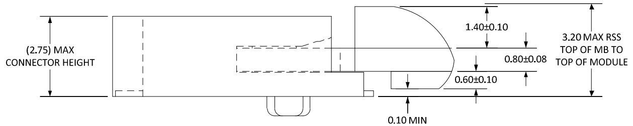
Figure 43. H2.8-D4 - Stack-up Top Mount Double-sided Module for 1.5 Maximum Top-side Component Height with 0.7 Maximum Bottom-side Component Height
