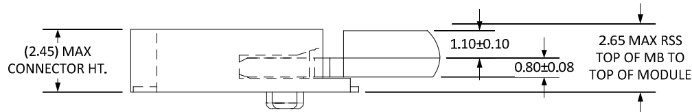
Figure 40. H2.5-S1 - Stack-up Top Mount Single-sided Module for 1.20 Maximum Top-side Component Height and with Higher Clearance above MB
