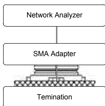
Figure 99. VSWR Test Setup for Receptacle RF Connector
