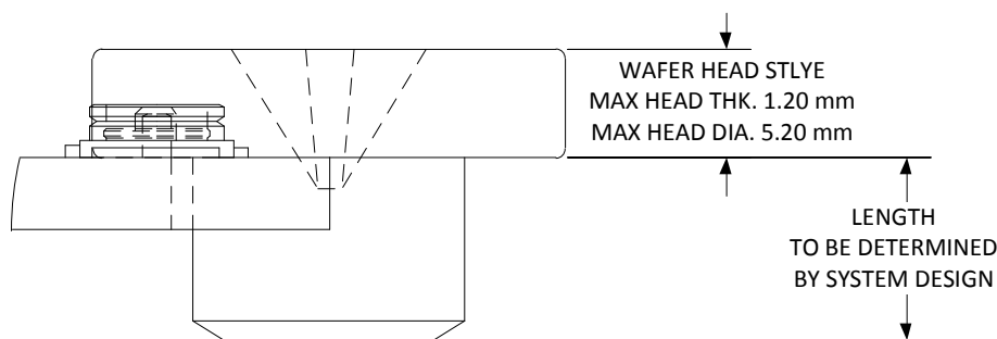
Figure 62. Mid-Line Module Mounting Interface
