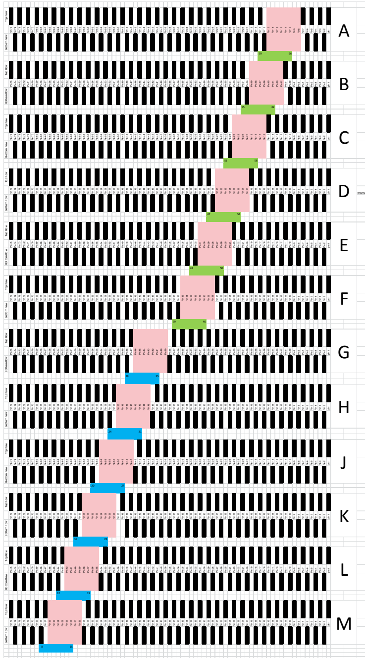
Figure 60. M.2 Connector Keying Diagram
