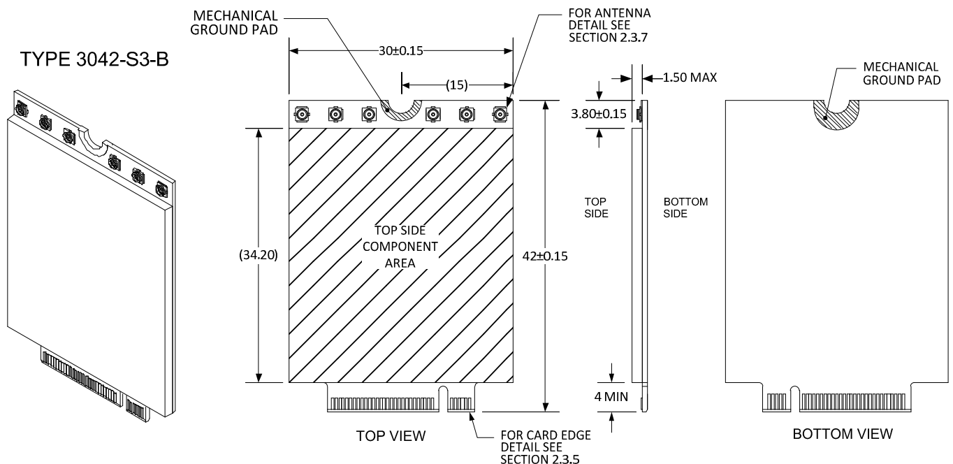
Figure 9. M.2 Type 3042 Single Sided Example Mechanical Outline Diagram Example
