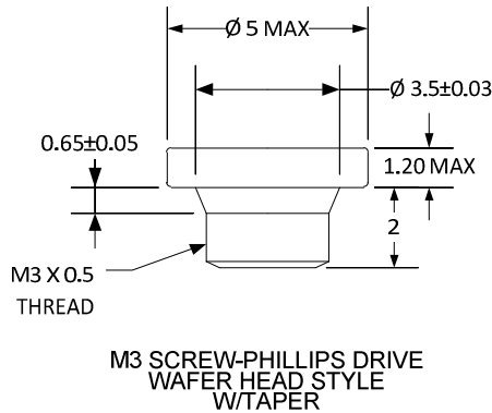
Figure 72. M3 Screw with Tapered Shaft
