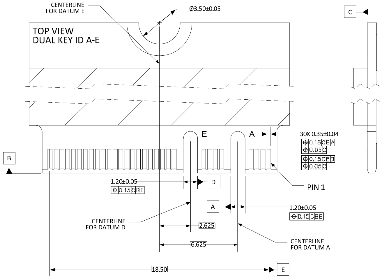
Figure 20. Dual Key A-E Example
