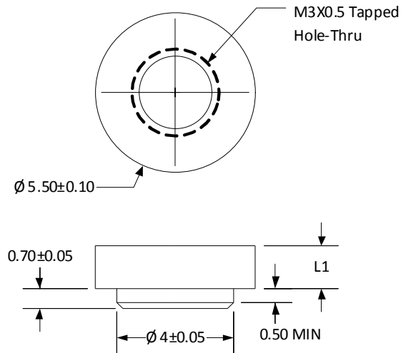
Figure 68. Flat Stand-Off
