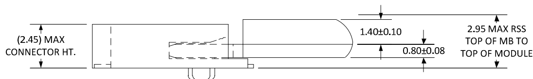
Figure 42. H2.5-S3 - Stack-up Top Mount Single-sided Module for 1.5 Maximum Top-side Component Height and with Higher Clearance above MB
