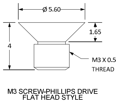
Figure 74. Flat-Head Style M3 Screw
