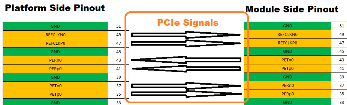
Figure 95. PCIe Signal Direction and Signal Name Changes
