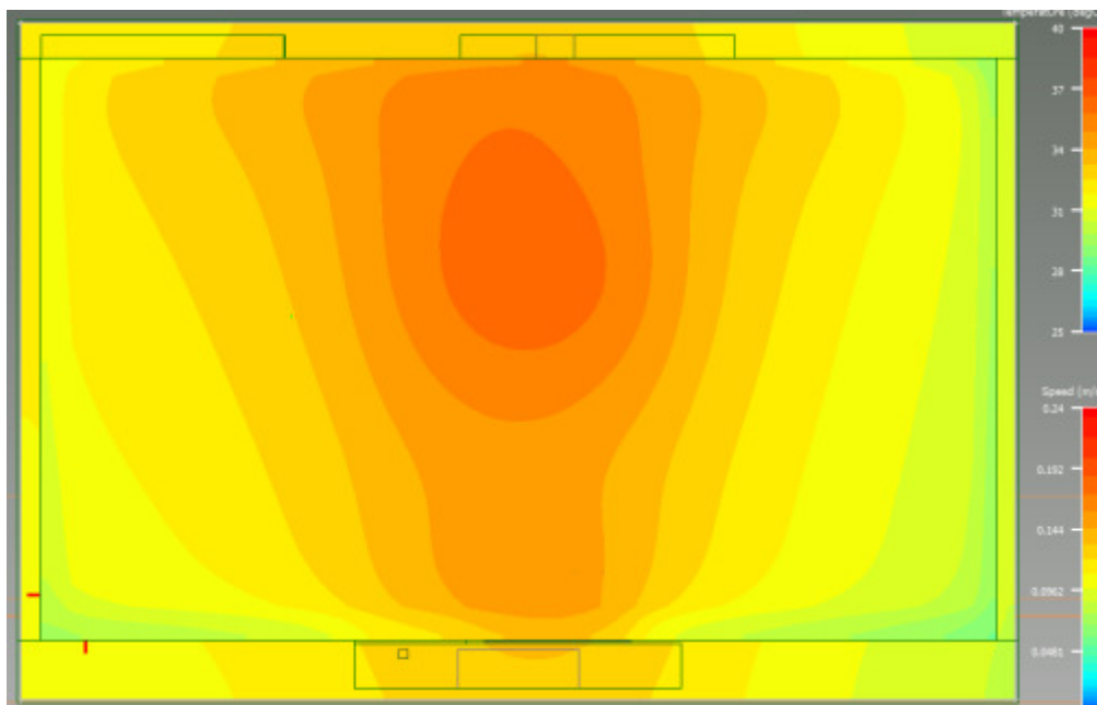
Figure 111. Example View of Display Surface Temperature with WWAN Use Case Estimate II
