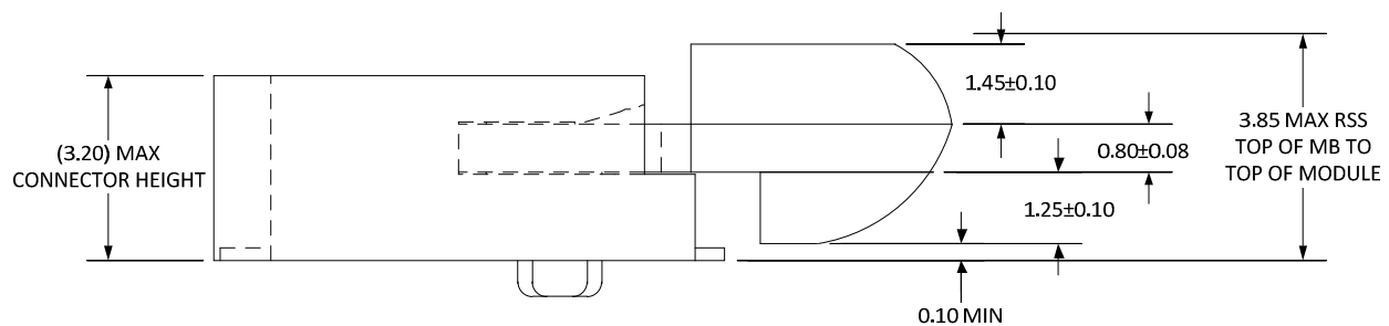
Figure 46. H3.2-D3 - Stack-up Top Mount Double-sided Module for 1.5 Maximum Top-side Component Height
