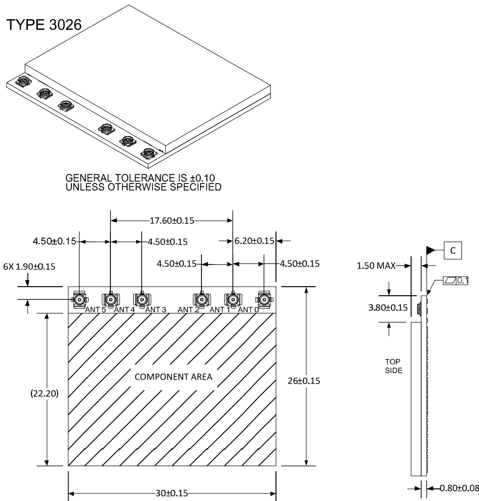
Figure 24. M.2 Type 3026-S3 Mechanical Outline Drawing
