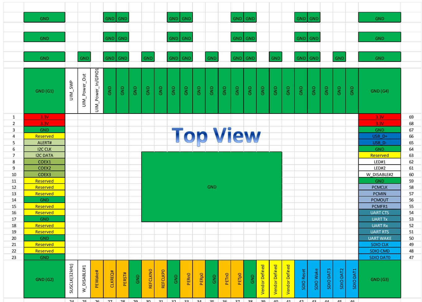
Figure 91. Type 2226 LGA Pin-Out Using Socket 1-SD Based Pin-Out on Platform
