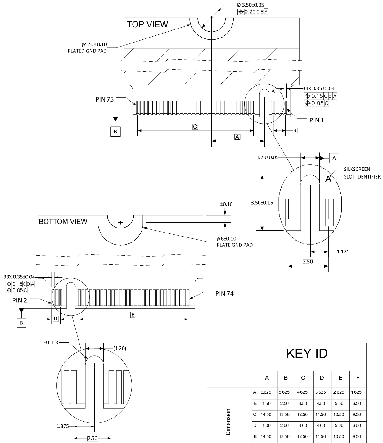
Figure 18. Key Detail for Keys A Thru F
