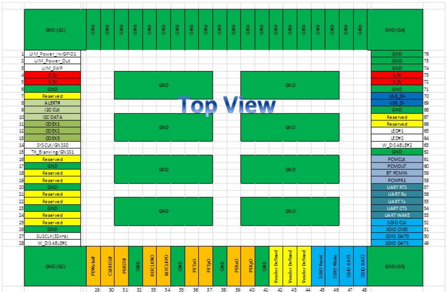
Figure 87. Type 1216 A-SD Based Module-Side Pin-Out
