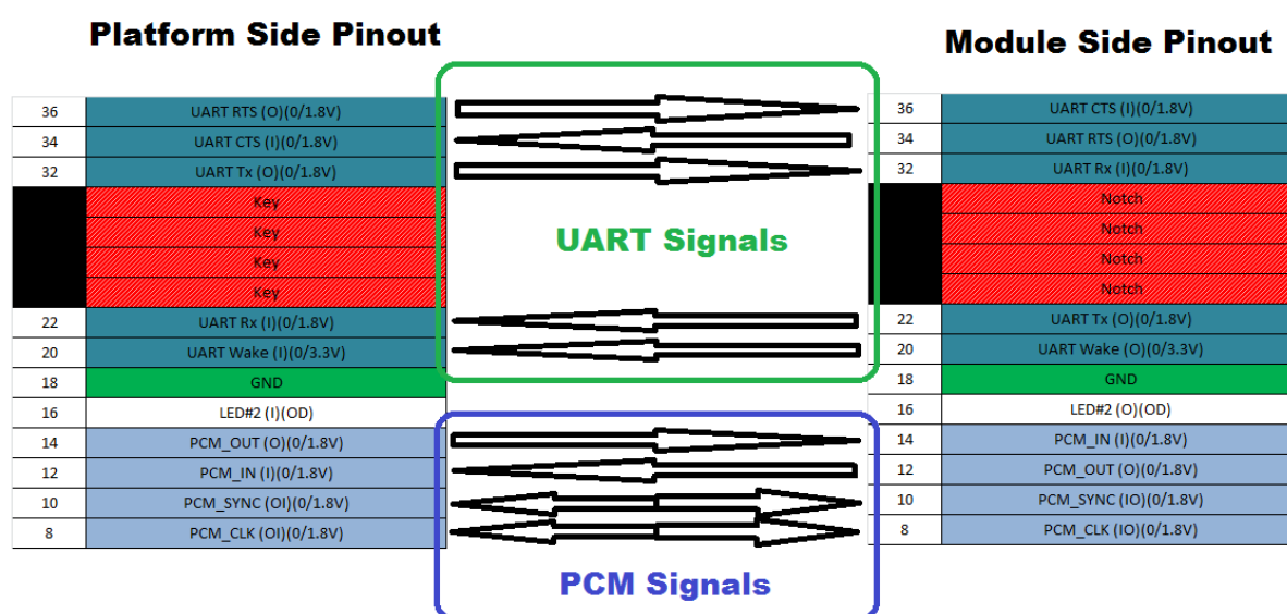
Figure 94. UART and PCM Signal Direction and Signal Name Changes
