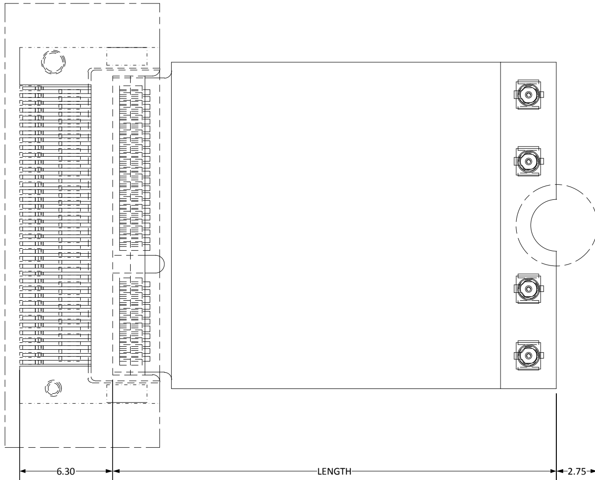
Figure 50. Mid-Line (In-Line) System Length
