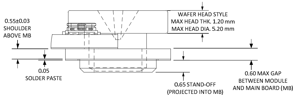
Figure 64. Elevated Single-sided Top Mount Solder Stand-Off
