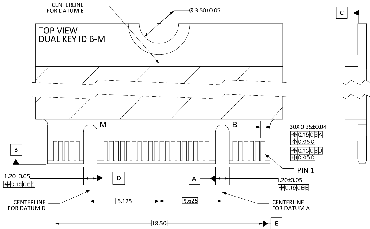
Figure 21. Dual Key B-M Example
