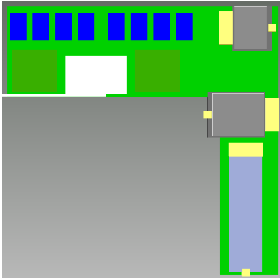
Figure 105. Example View of Motherboard for Thin Platform Notebook with fan
