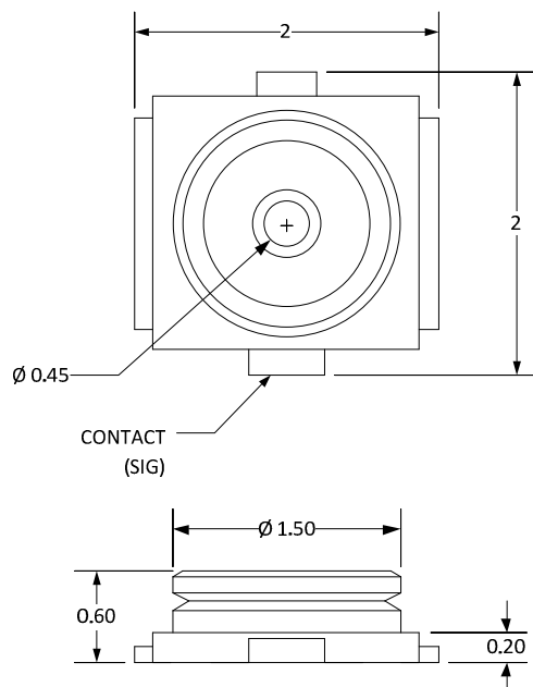
Figure 27. Generic 2x2 mm RF Receptacle Connector Diagram
