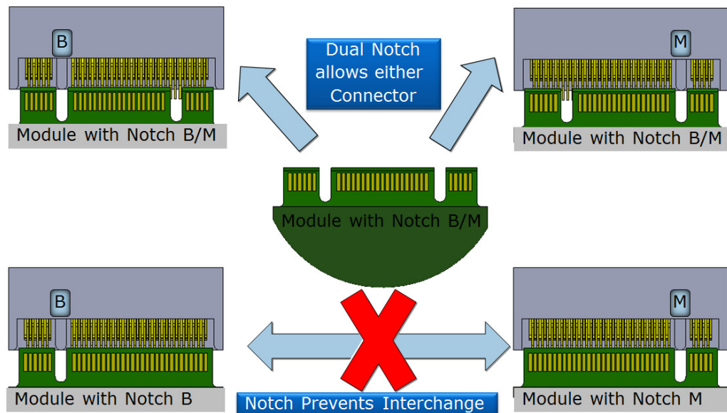
Figure 61. Dual Module key Scheme Example
