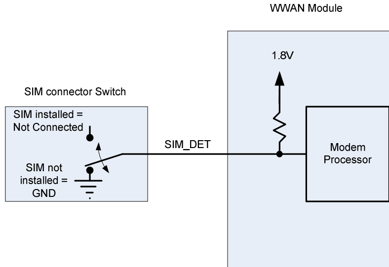
Figure 89. Typical SIM Detect Circuit Implementation
