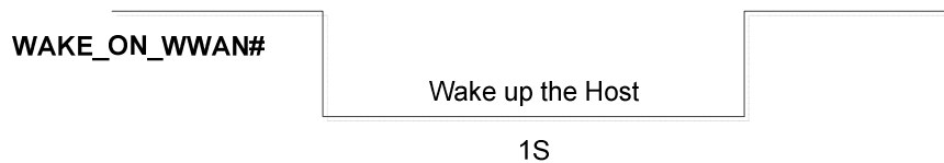
Figure 90. WAKE_ON_WWAN# Signal
