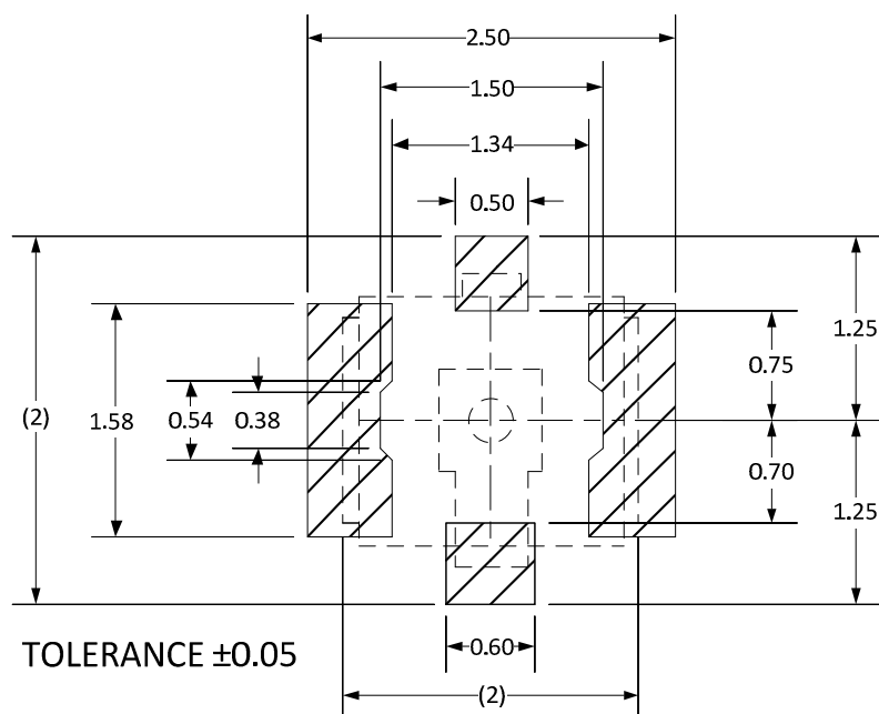
Figure 30. Antenna Connector PCB Recommended Land Pattern
