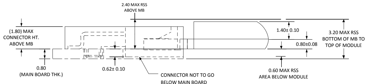
Figure 53. Stack-up Mid-Line (In-line) Single Sided Module for 1.5 Maximum Component Height
