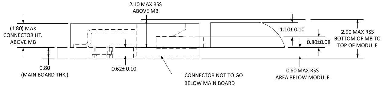
Figure 51. Stack-up Mid-Line (In-line) Single Sided Module for 1.2 Maximum Component Height
