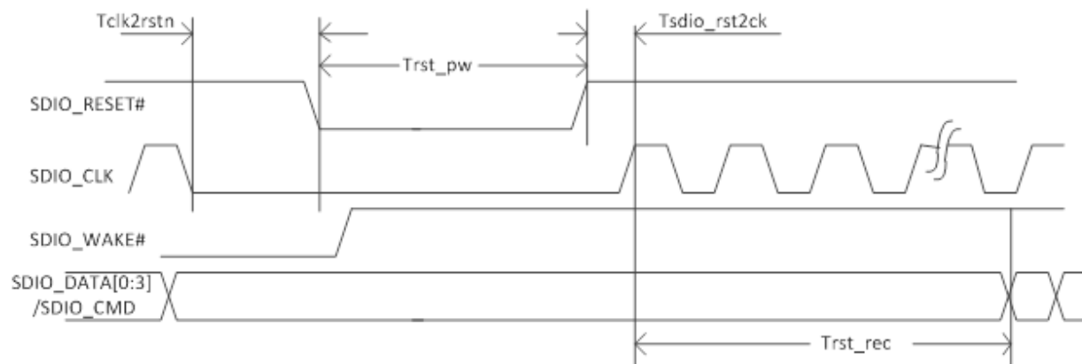
Figure 77. SDIO Reset Sequence
