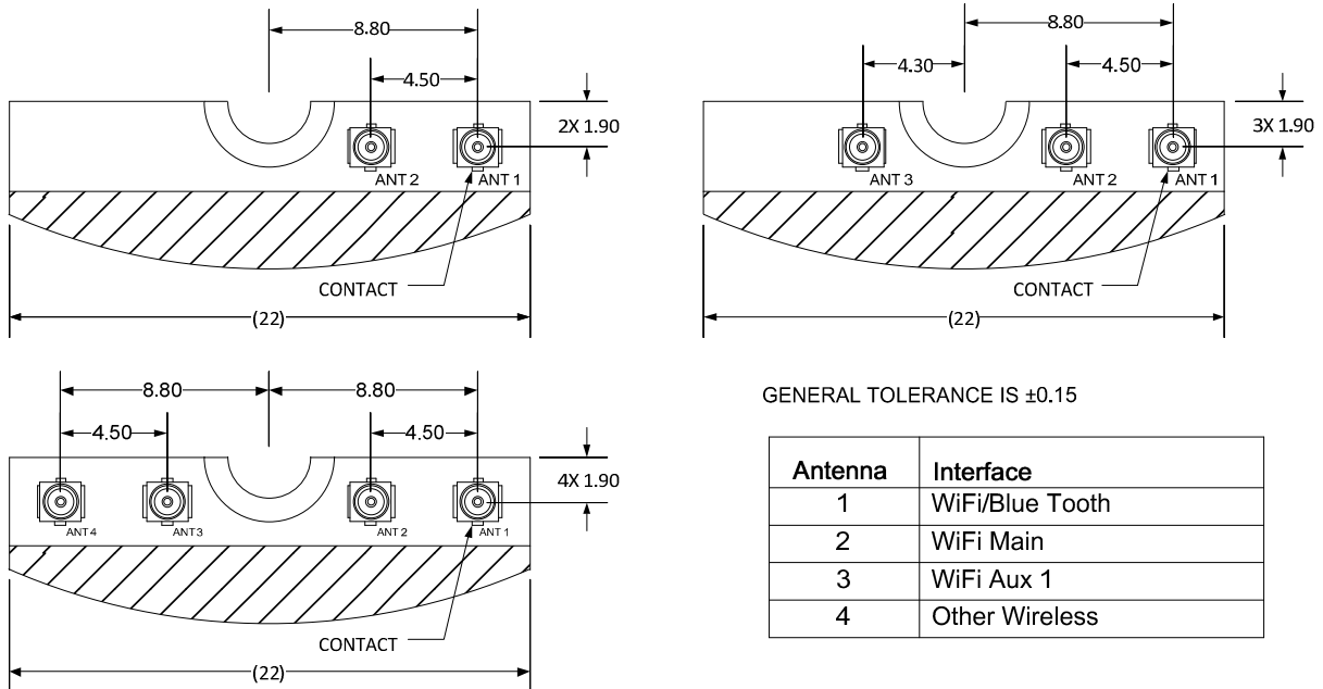
Figure 31. Socket 1 Type 2230 RF Connector Assignment Recommendation
