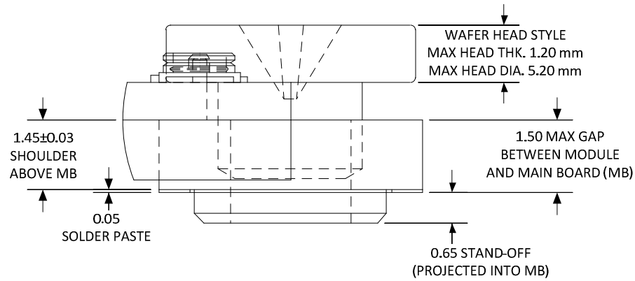
Figure 66. Double-sided Top Mount Solder Down Stand-off
