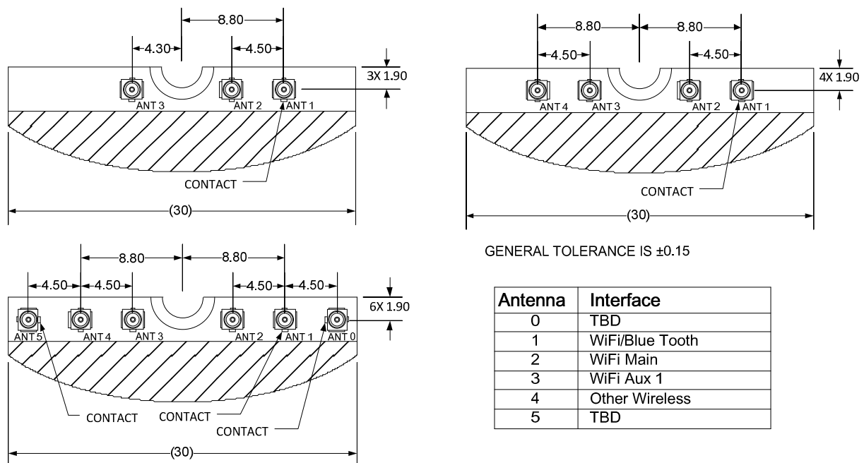
Figure 32. Socket 1 Type 3030 RF Connector Assignment Recommendation
