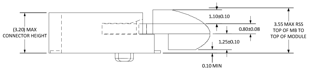
Figure 44. H3.2-D1 - Stack-up Top Mount Double-sided Module for 1.20 Maximum Top-side Component Height
