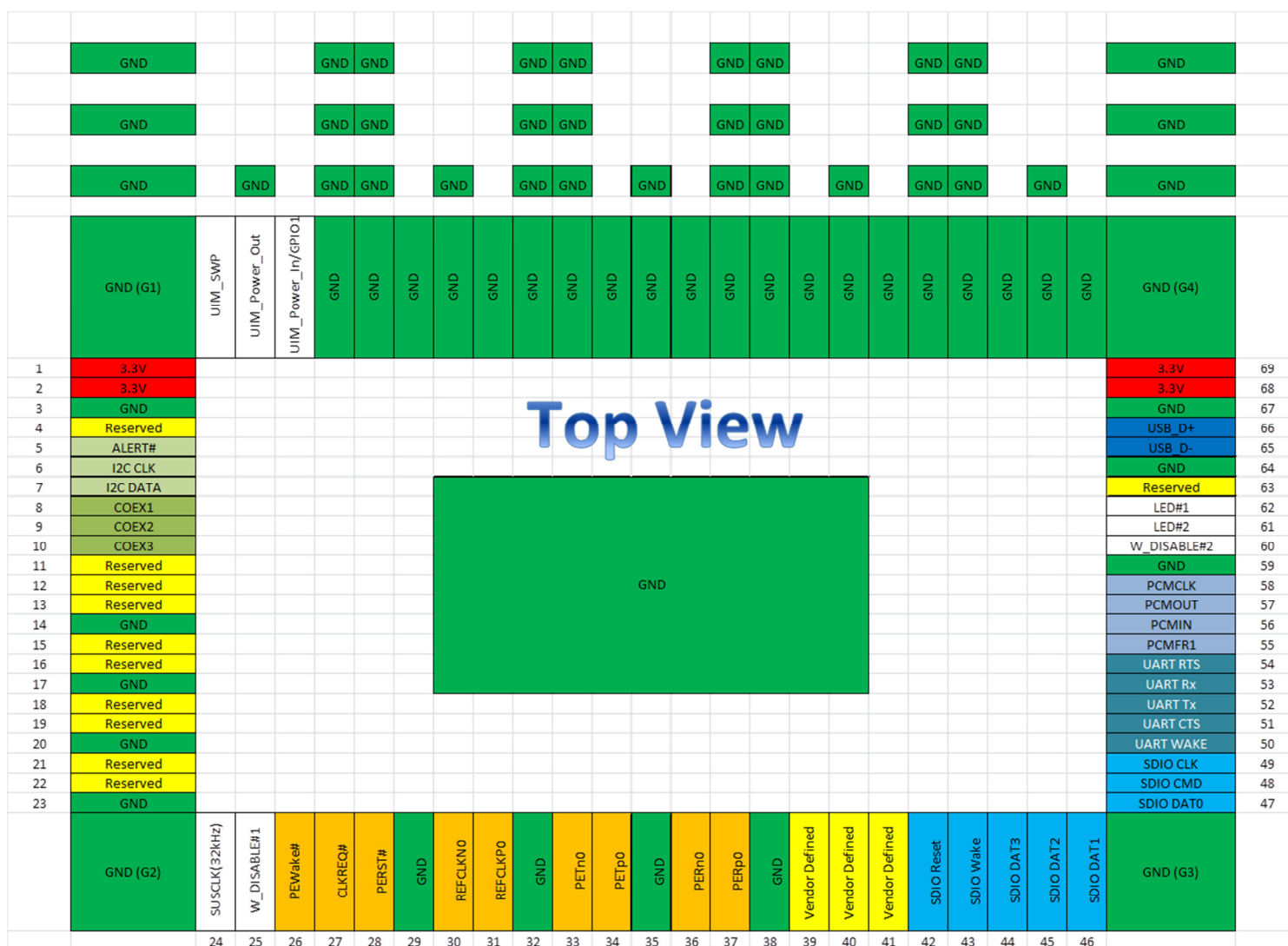
Figure 86. Type 2226 A-SD Based Module-Side Pin-Out
