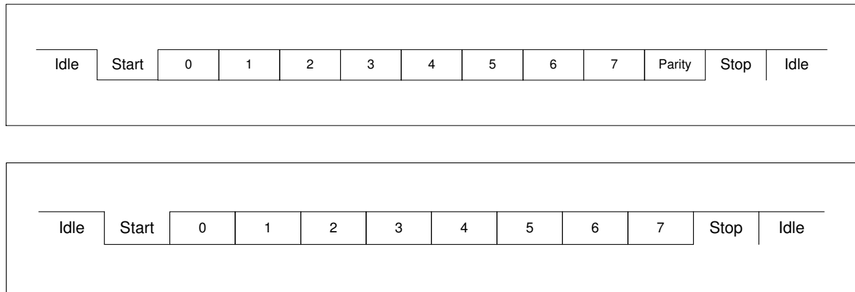
Figure 79. UART Frame Format
