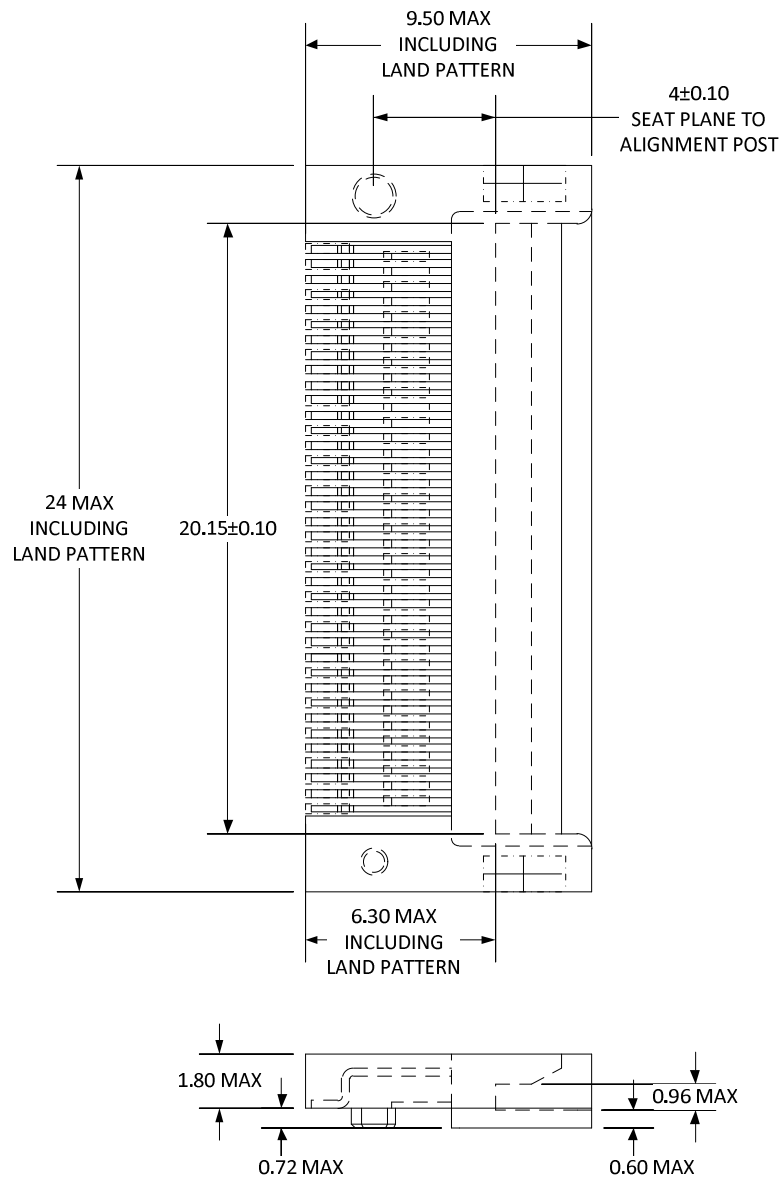
Figure 49. Mid-Line (In-line) Connector Dimensions
