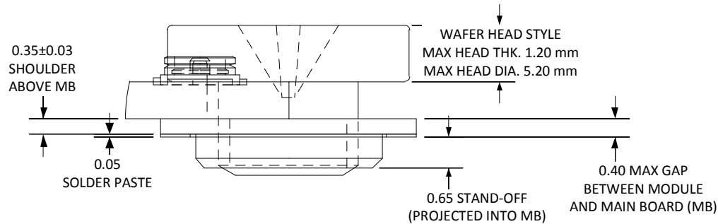
Figure 63. Single-sided Top Mount Solder Down Stand-off
