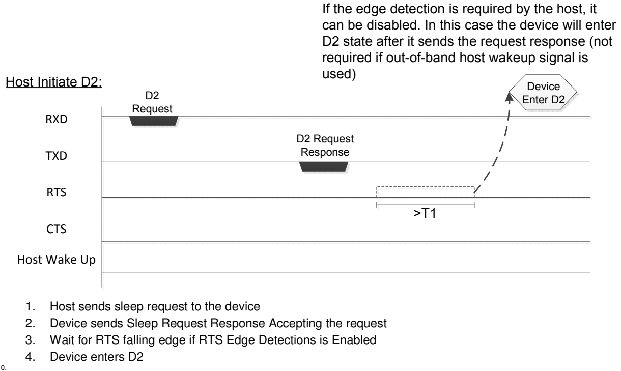
Figure 80. Sleep Request Initiated by the Host
