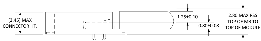
Figure 41. H2.5-S2 - Stack-up Top Mount Single-sided Module for 1.35 Maximum Top-side Component Height and with Higher Clearance above MB
