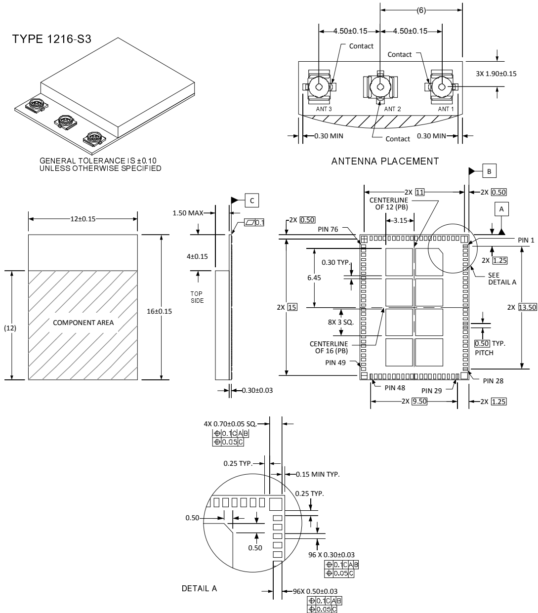
Figure 23. Type 1216 Soldered Down Solution Module Diagram
