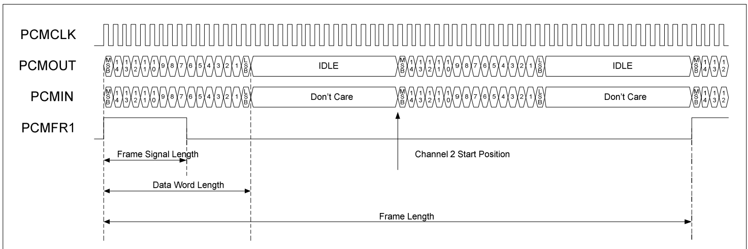
Figure 84. Typical PCM Transaction Timing Diagram
