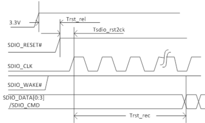
Figure 78. SDIO Power-Up Sequence
