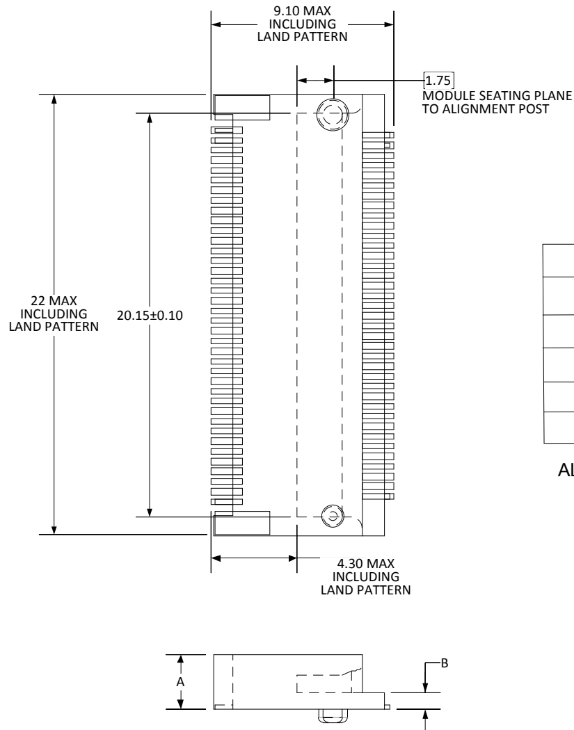
Figure 35. Top Side Connector Dimensions
