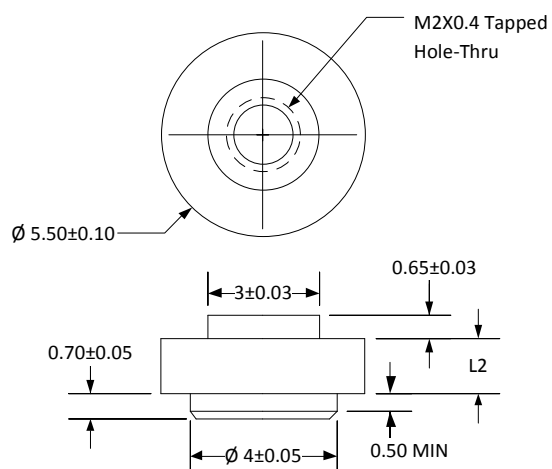
Figure 69. Shouldered Stand-Off
