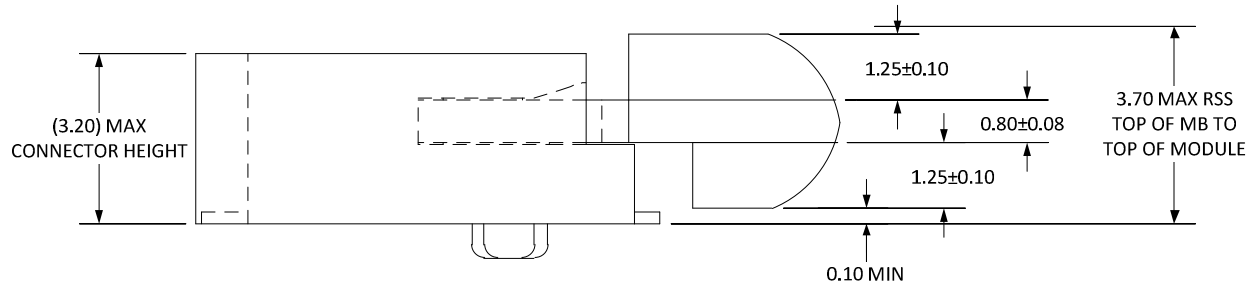
Figure 45. H3.2-D2 - Stack-up Top Mount Double-sided Module for 1.35 Maximum Top-side Component Height
