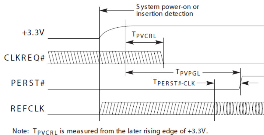
Figure 75. Power-Up CLKREQ# Timing
