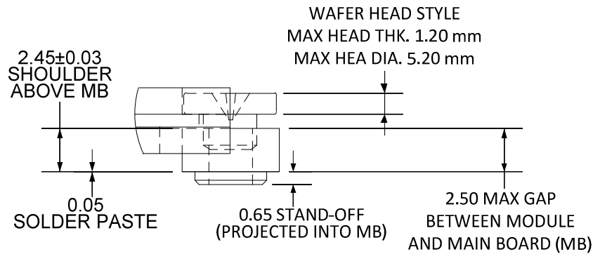
Figure 57. Stack-up Mid-Line (In-line) Double-sided (D5) Module for 1.5 Maximum Top-side and Bottom-side Component Height
