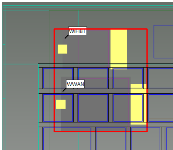
Figure 103. Example View of Region Over Modules
