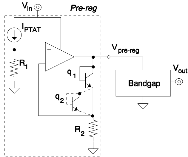
Figure 6.13. Pre-regulated supply voltage realization.
