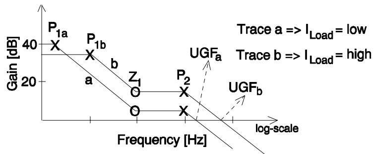
Figure 4.3. System frequency response as a function of load-current.
