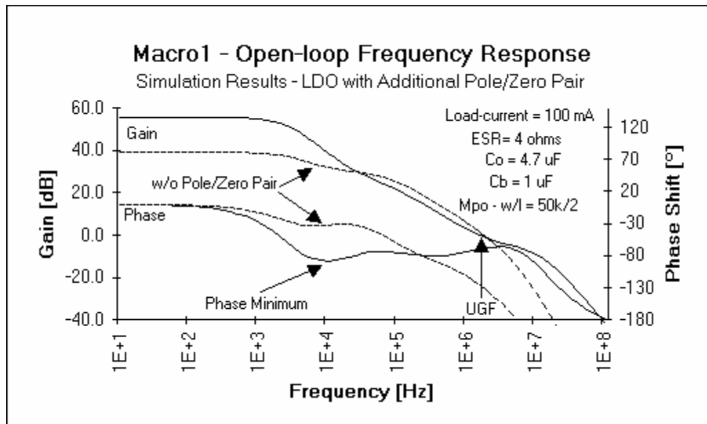
Figure 4.10. AC simulation of LDO with an additional pole/zero pair.
