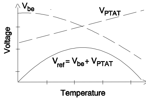
Figure 5.2. Temperature behavior of first order bandgaps.
