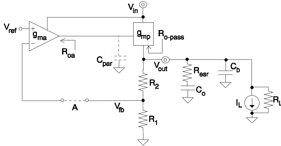
Figure 2.1. System model under loading conditions.
