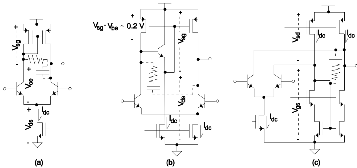
Figure 6.10. Gain stage topologies.
