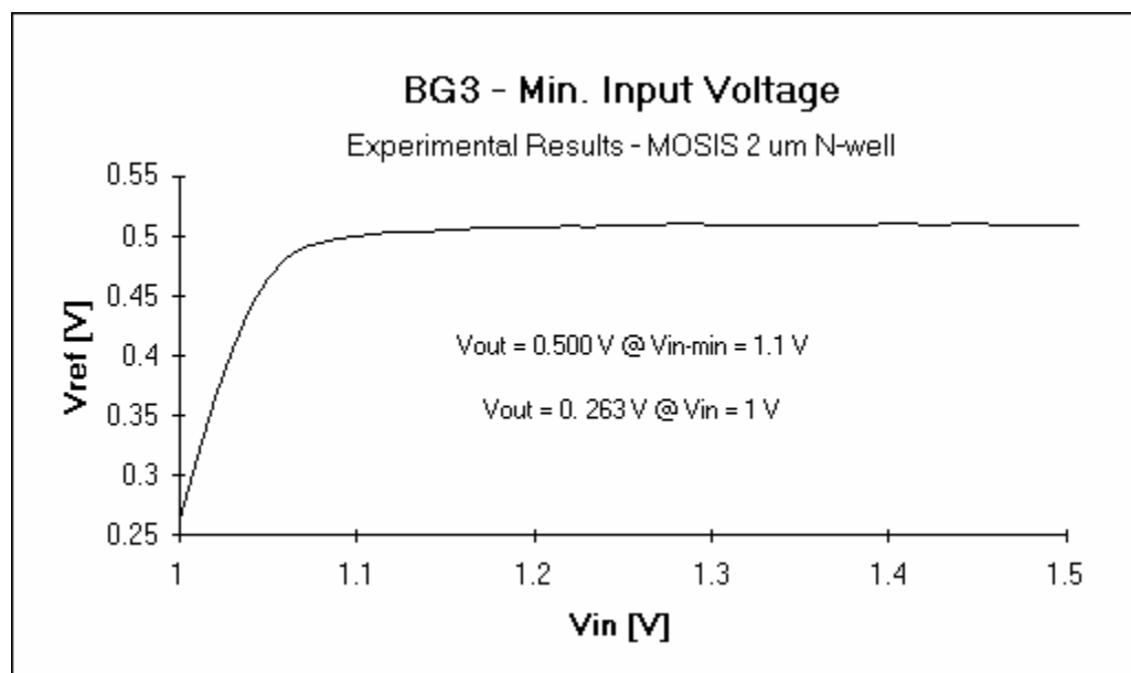
Figure 7.21. Minimum input voltage of the reference.
