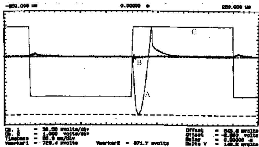
Figure 7.14. Transient response to a full range load-current step (A) with and (B) without the aid of load dependent biasing in the current efficient buffer.
