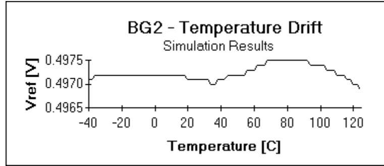
Figure 6.12. Temperature drift performance of the bandgap reference.
