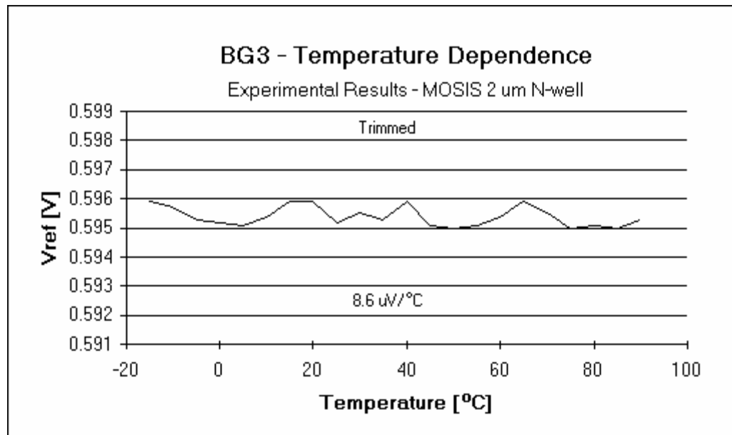
Figure 7.18. Temperature drift performance of the trimmed reference.
