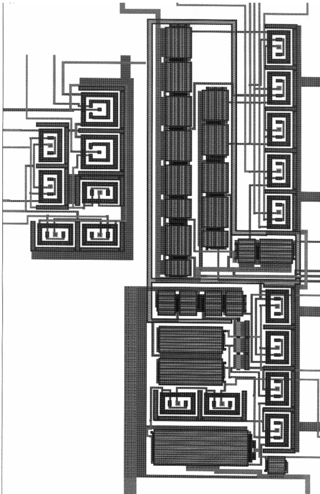
Figure C.2. Zoom-in plot of the start-up and reference ( 290 \times 173 \mu\text{m} & 798 \times 280 \mu\text{m} ).
