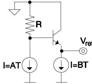
Figure 5.7. \beta curvature corrected bandgap.
