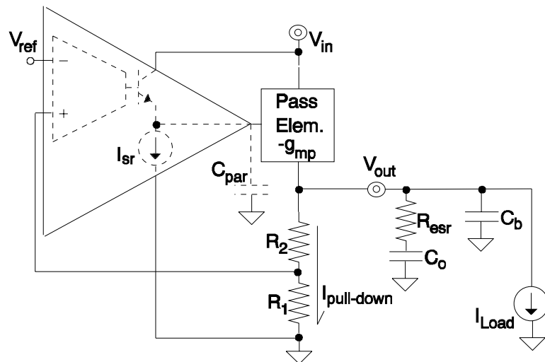
Figure 2.5. Simplified LDO schematic for the purpose of transient analysis.
