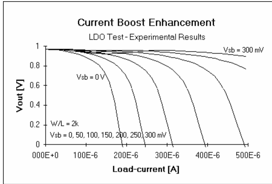
Figure 4.5. Maximum load-current performance of the current boost enhancement.
