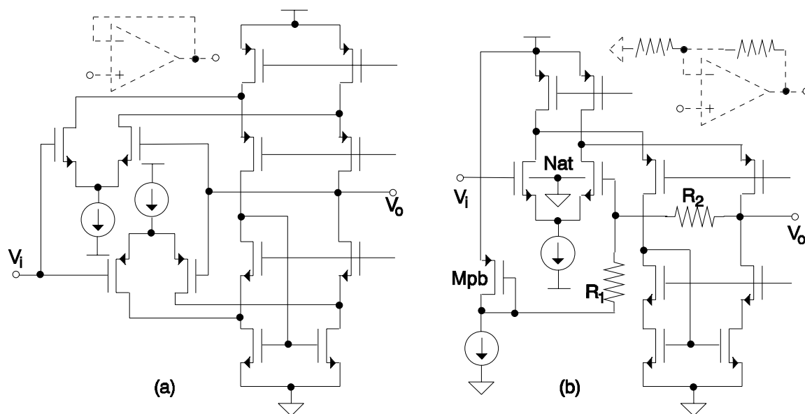
Figure 6.6. Non-inverting amplifier topologies.
