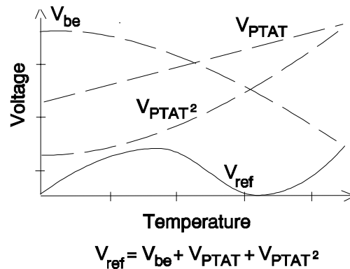
Figure 5.3. Squared PTAT curvature correction method for bandgaps.
