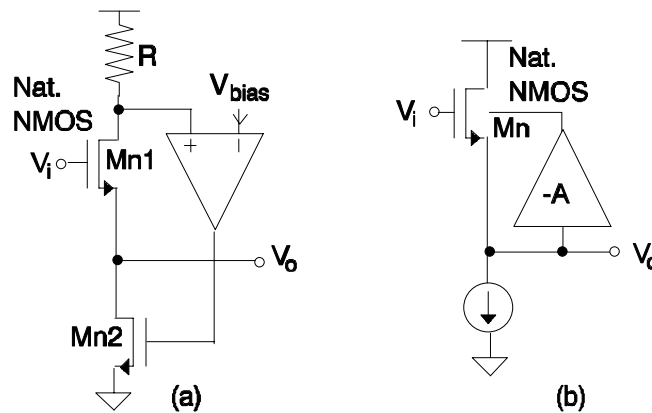
Figure 6.7. Feedback buffer structures.
