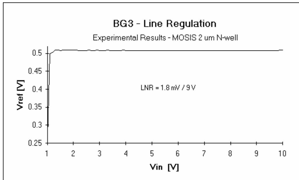
Figure 7.20. Line regulation performance of the reference.
