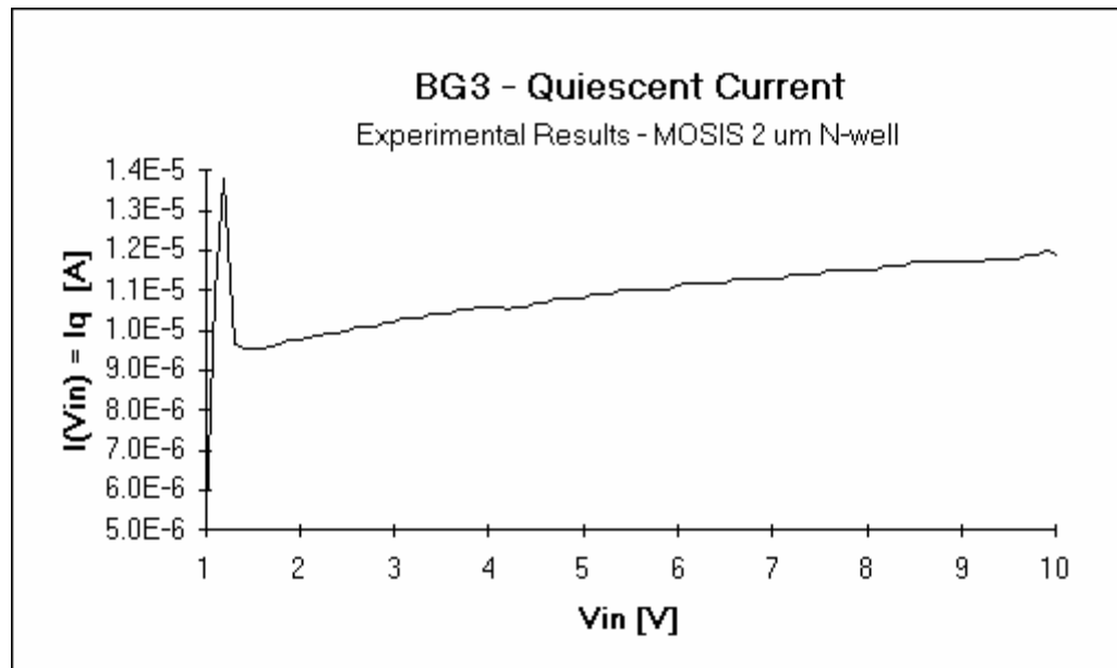
Figure 7.22. Quiescent current flow of the reference.
