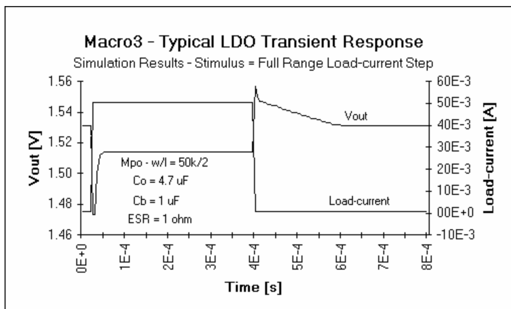
Figure 2.6. Simulated LDO transient response of a circuit similar to that of Figure 2.5.
