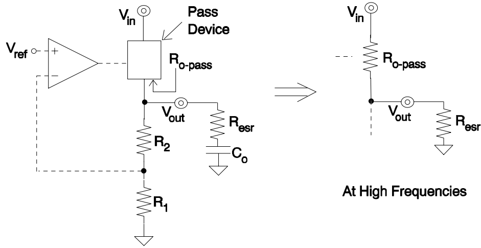
Figure 1.2. PSRR performance implications of high frequency operation.
