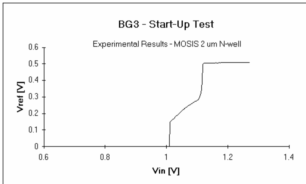
Figure 7.19. Reference start-up test.
