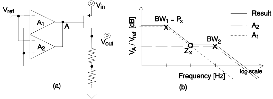
Figure 4.11. Parallel amplifier pole/zero pair realization.
