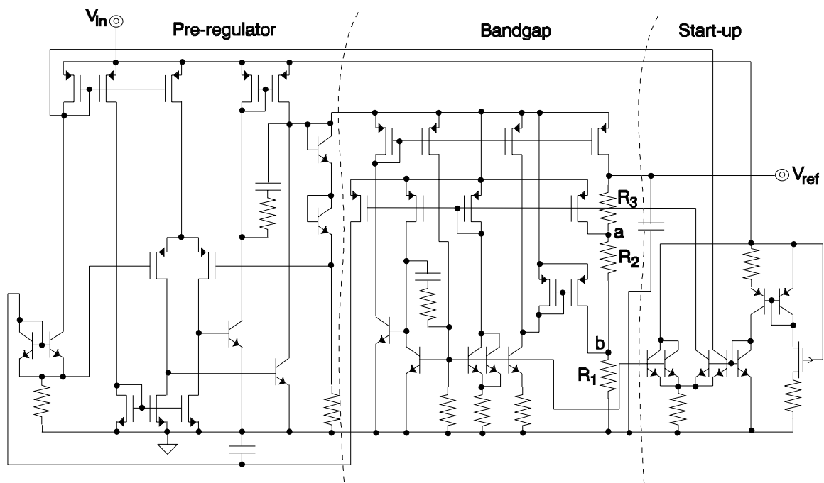
Figure 6.14. Low voltage curvature corrected bandgap.
