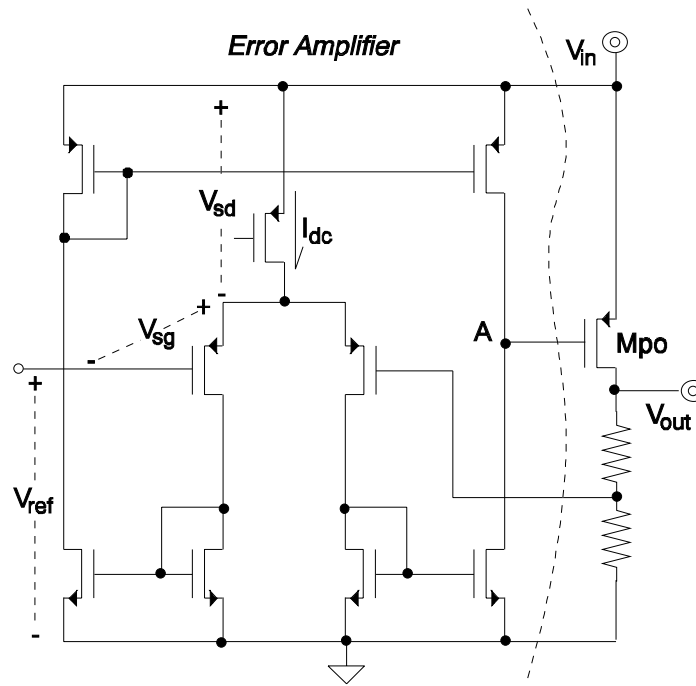
Figure 3.1. CMOS low drop-out regulator topology.
