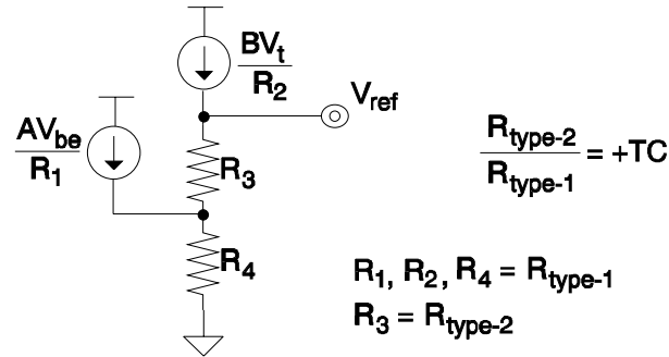
Figure 5.9. Temperature dependent resistor ratio curvature correction.
