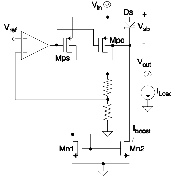
Figure 4.6. LDO with current boosting capabilities.
