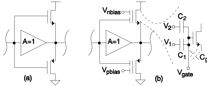
Figure 4.1. Slew-rate dependent boost circuit.
