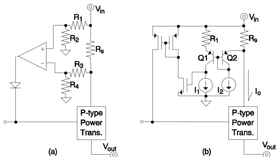
Figure 7.3. Low voltage current limiting circuit protection.
