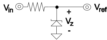
Figure 5.1. Zener diode reference.
