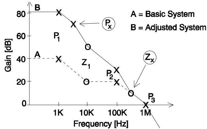
Figure 4.9. System's frequency response with an additional pole/zero pair.
