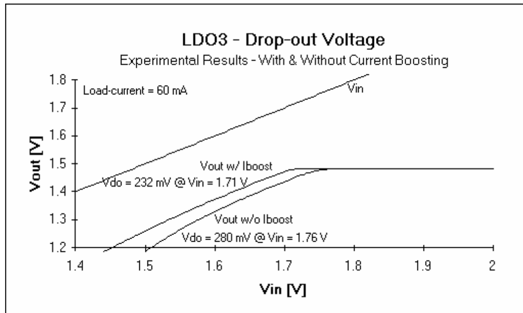
Figure 7.11. Drop-out voltage performance.
