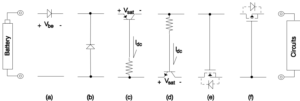
Figure 7.5. Reverse battery protection circuits.
