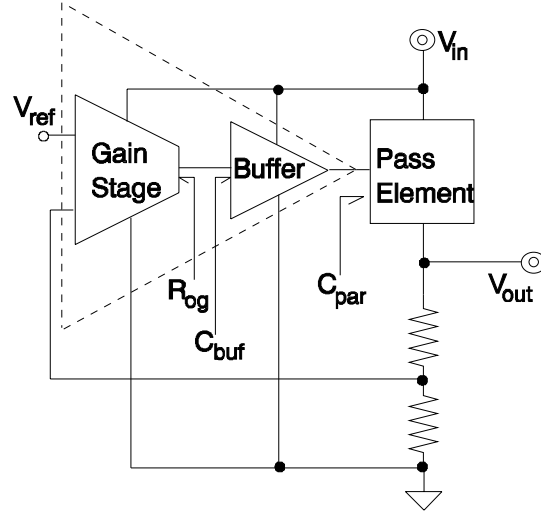
Figure 2.7. LDO buffered architecture.
