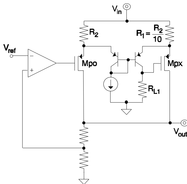
Figure 3.6. Multi-path device regulator.
