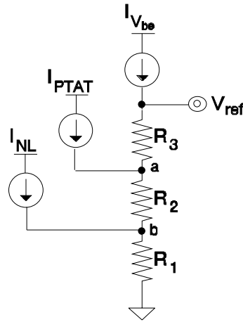
Figure 5.5. IV-mode output topology.
