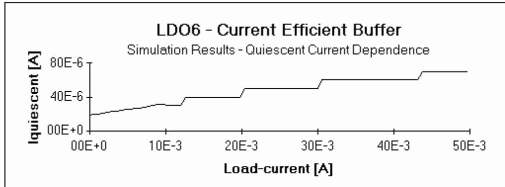
Figure 6.9. Quiescent current dependence of buffer on load-current.
