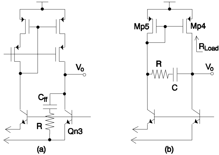
Figure 4.13. Variations of the frequency shaping amplifier.
