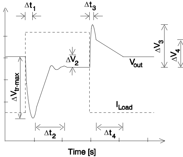
Figure 2.4. Typical LDO transient response to a load-current step.
