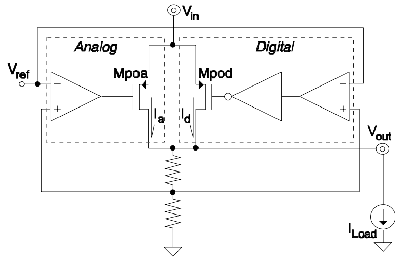
Figure 3.4. Mixed-mode regulator.
