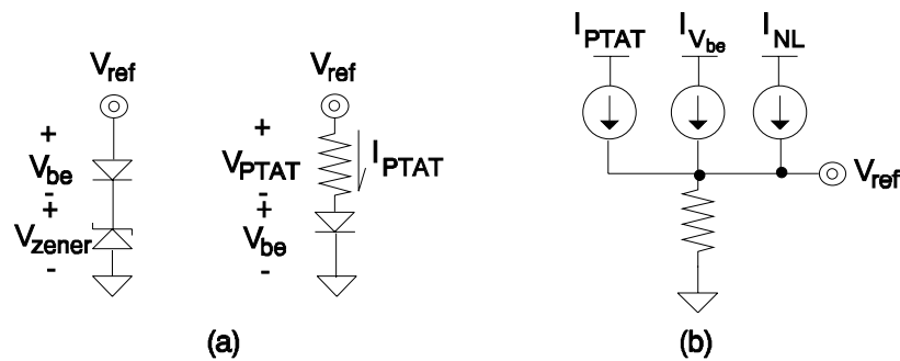
Figure 5.4. Output structures (a) voltage-mode and (b) current-mode.
