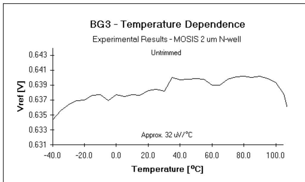
Figure 7.17. Temperature drift performance of the untrimmed reference.
