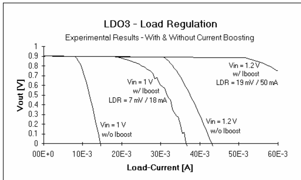
Figure 7.12. Load regulation performance.
