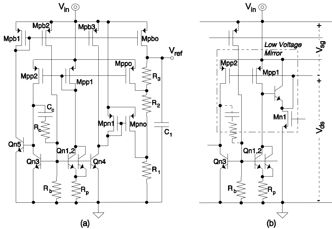
Figure 6.11. Bandgap with current subtraction curvature correction.
