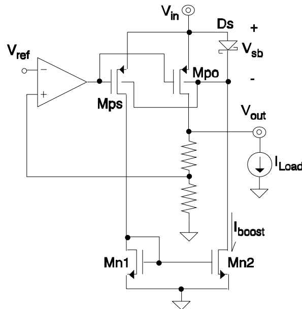
Figure 6.3. Composite PMOS pass device.
