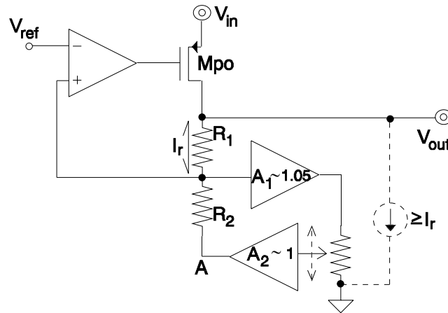
Figure 3.7. Widely adjustable low drop-out regulator structure.
