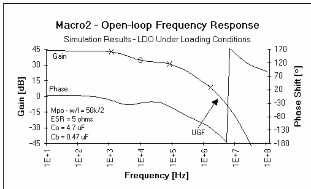
Figure 2.3. AC simulation results of an LDO under loading conditions.
