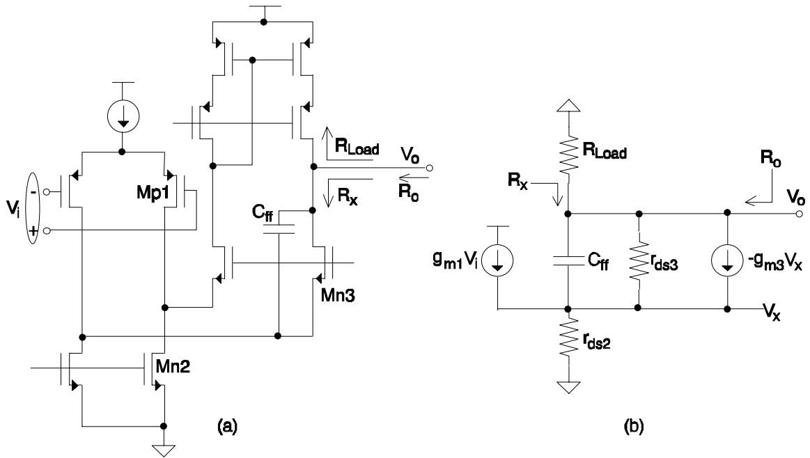
Figure 4.12. Pole/zero pair generation by a feed-forward capacitor.
