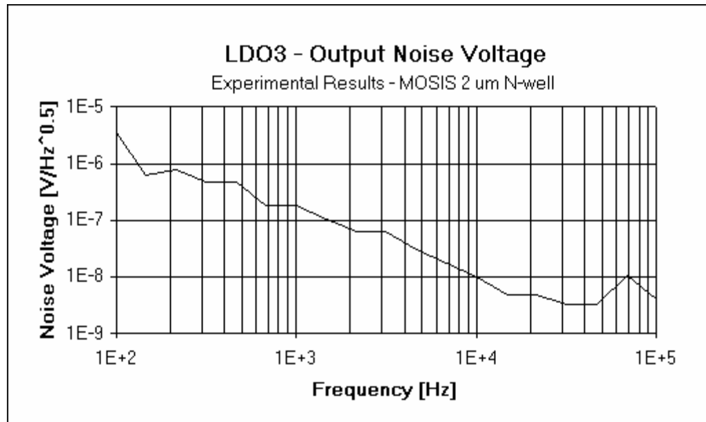
Figure 7.15. Control loop output noise voltage performance.
