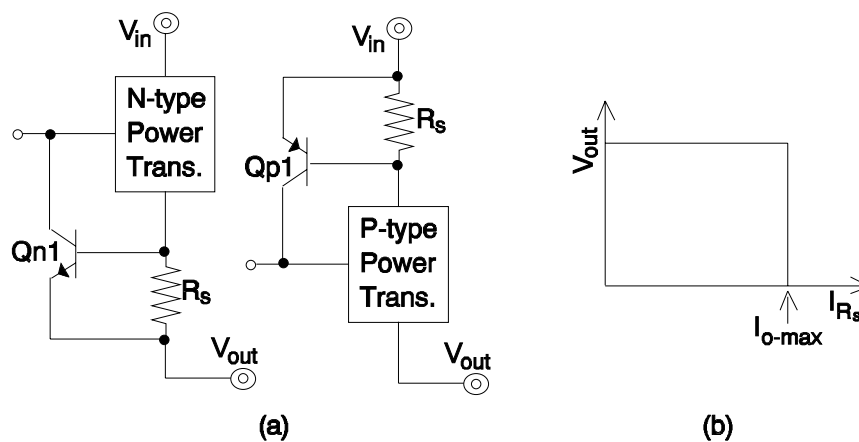
Figure 7.2. Current limiting circuit protection.
