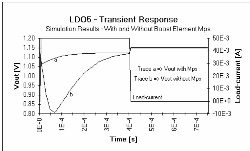
Figure 4.4. LDO output voltage variation with and without the boost element Mps in the current efficient buffer stage.
