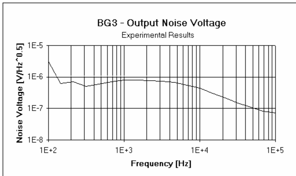
Figure 7.23. Reference output noise voltage performance.
