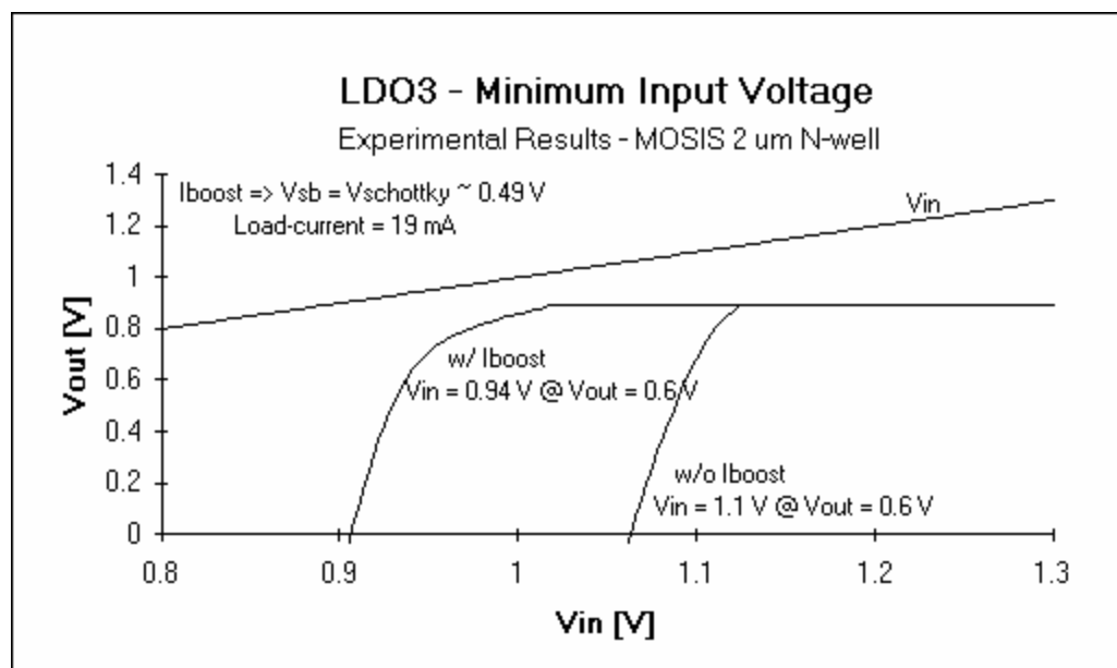
Figure 7.10. Minimum input voltage of the control loop.
