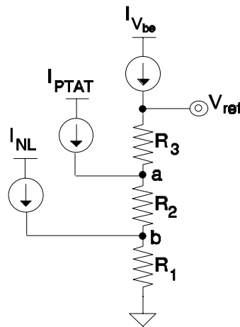
Figure B.1. IV-mode bandgap output structure.
