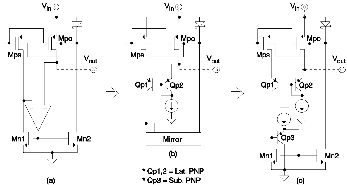
Figure 6.5. Pass device design development for efficient current sensing.
