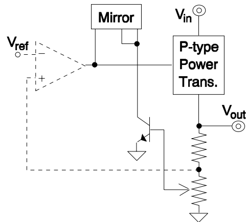
Figure 7.6. Thermal shutdown protection circuit.
