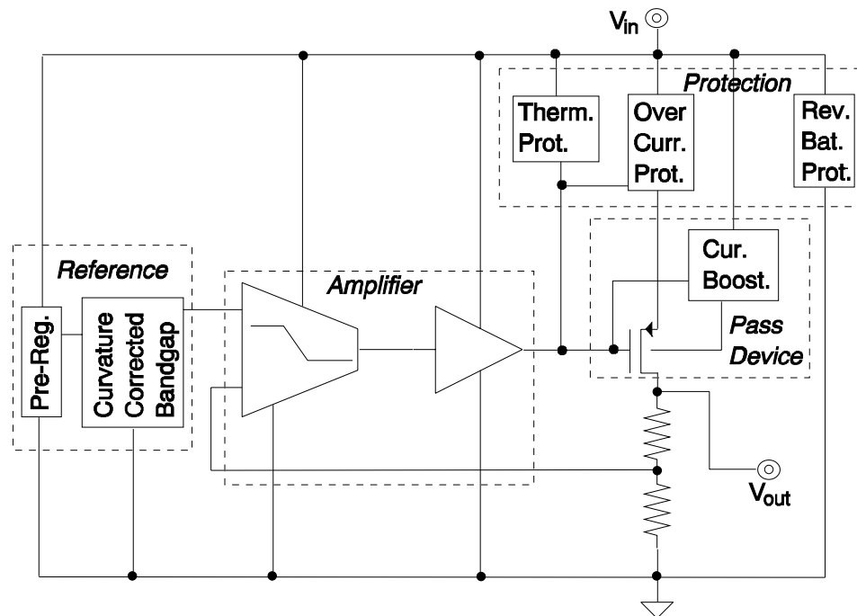
Figure 7.1. Complete system block level diagram.
