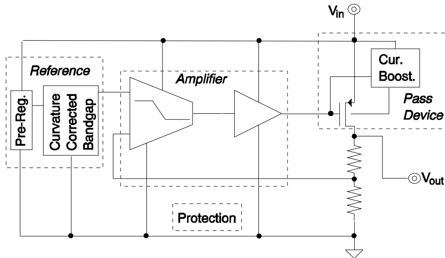
Figure 6.1. Block level diagram of the system.
