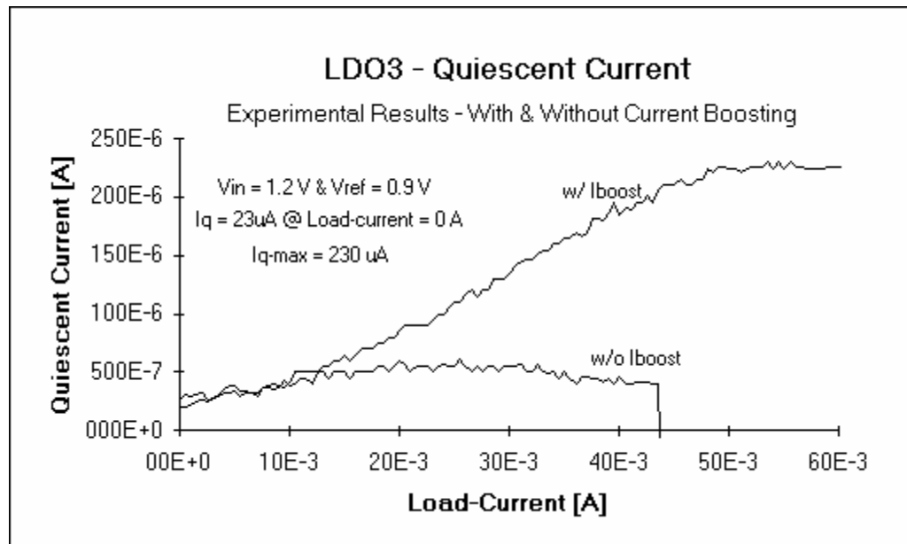
Figure 7.13. Quiescent current flow of the control loop.
