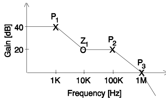
Figure 2.2. LDO frequency response under loading conditions.
