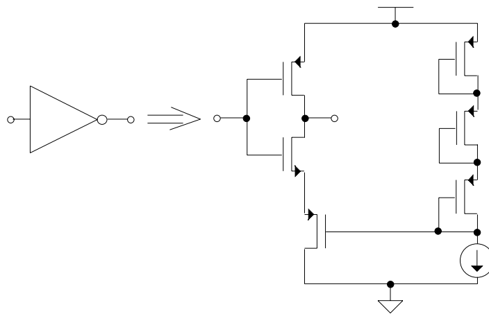
Figure 3.5. Digital inverter for the mixed-mode regulator.
