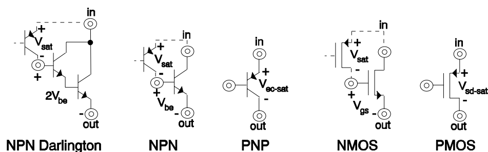
Figure 6.2. Pass element structures.
