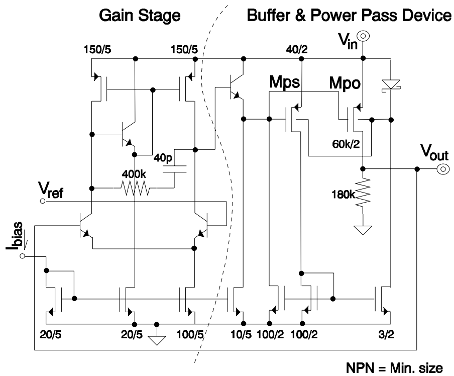
Figure 7.7. Schematic of the control loop circuit.
