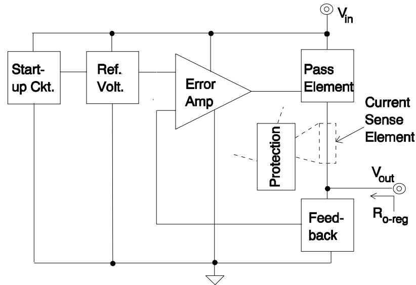
Figure 1.1. Generic low drop-out series linear regulator architecture.
