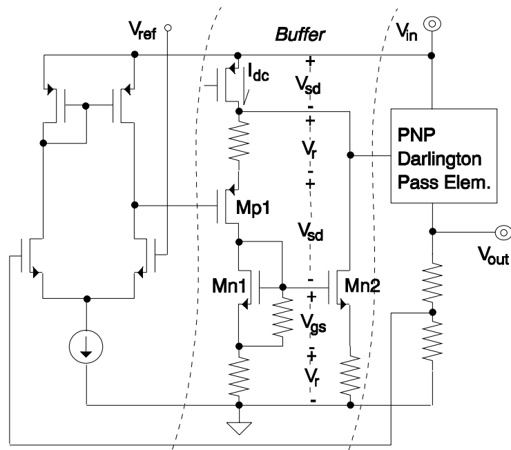
Figure 3.2. Buffered low drop-out regulator architecture.
