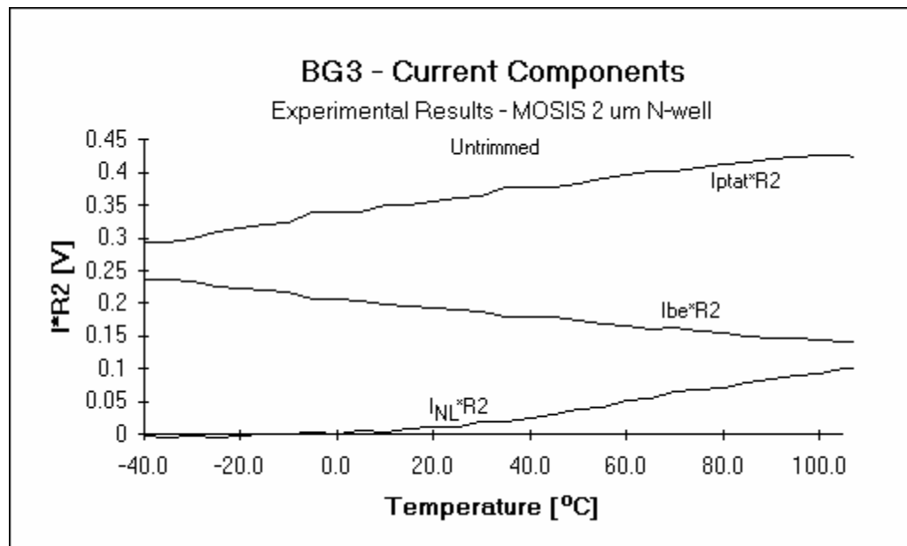
Figure 7.16. Temperature dependent currents in the reference.
