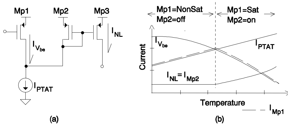
Figure 5.10. Current subtraction method for generating I_{NL} .
