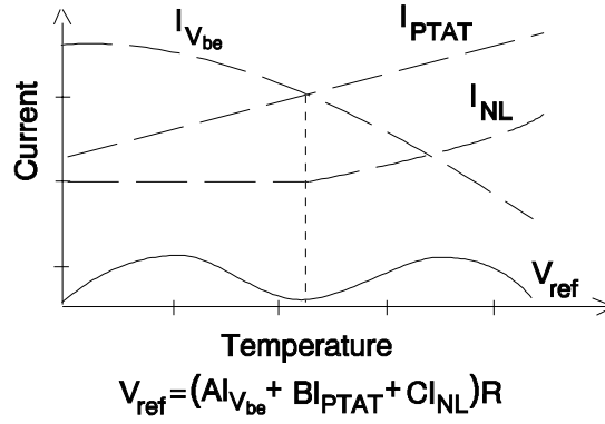
Figure 5.11. Temperature dependence of the curvature corrected bandgap.
