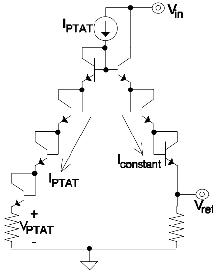
Figure 5.8. Quasi-nonlinear term cancellation bandgap reference.
