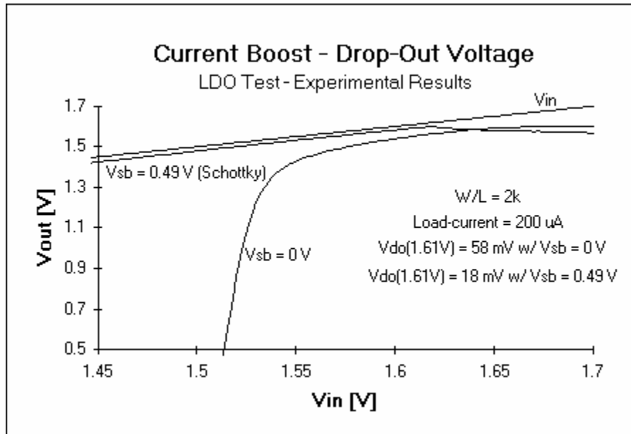
Figure 4.7. Drop-out voltage performance of the current boost topology.
