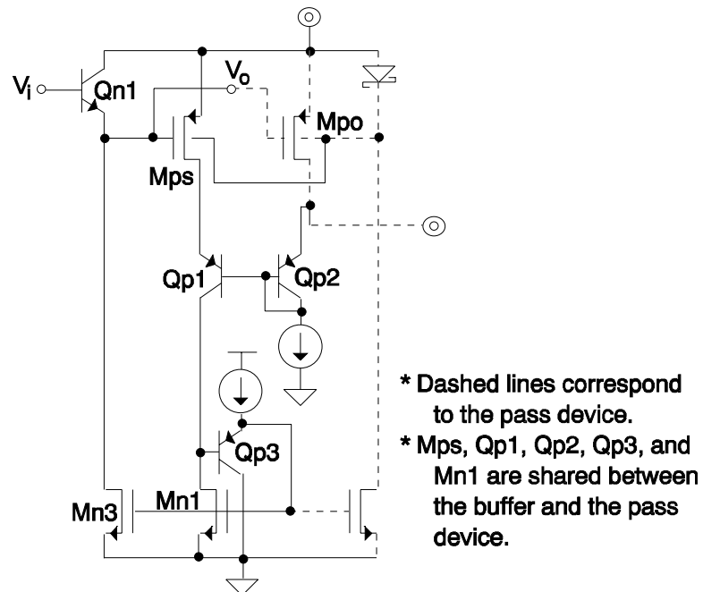
Figure 6.8. Current efficient buffer.
