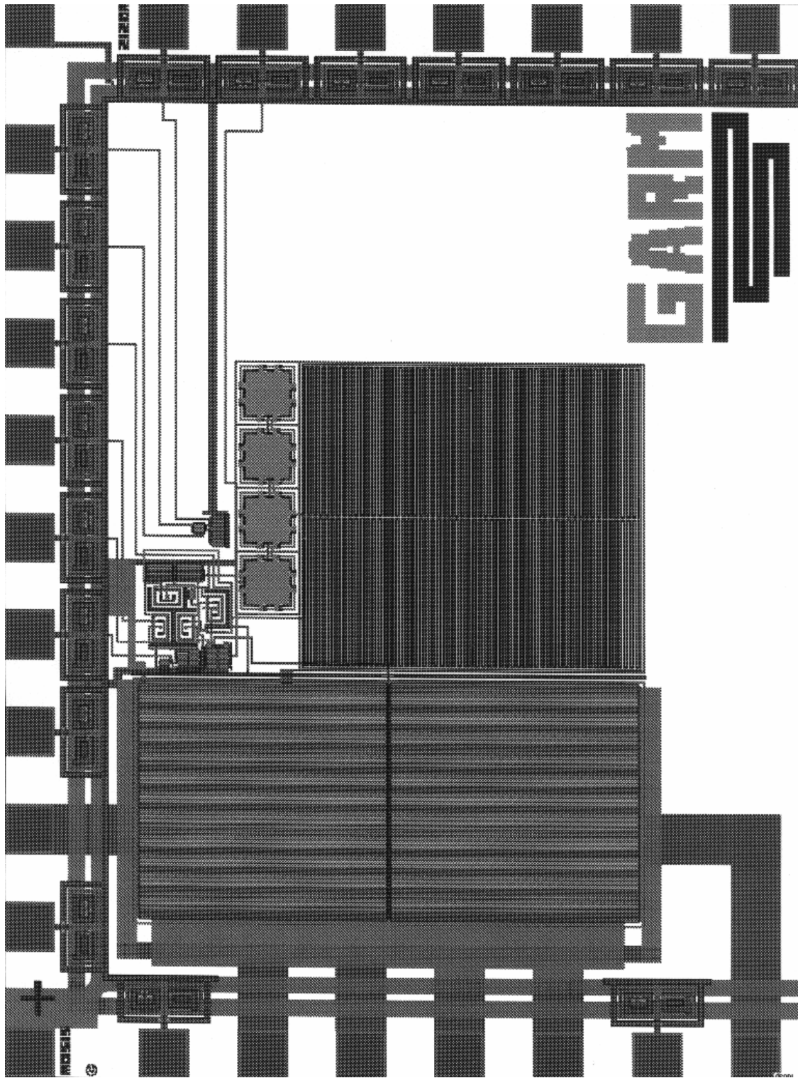
Figure C.3. Layout of the control loop (1103 x 1250 \mu\text{m} ).
