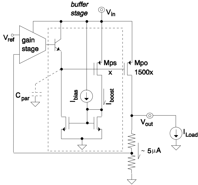
Figure 4.2. Current efficient-transient boost LDO buffer stage.
