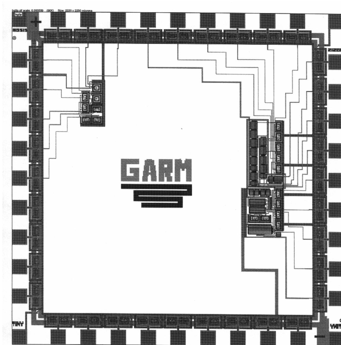
Figure C.1. Layout of the curvature corrected bandgap and associated start-up circuit.
