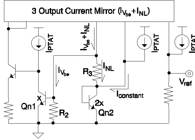
Figure 5.6. V_{be} loop curvature correction method.
