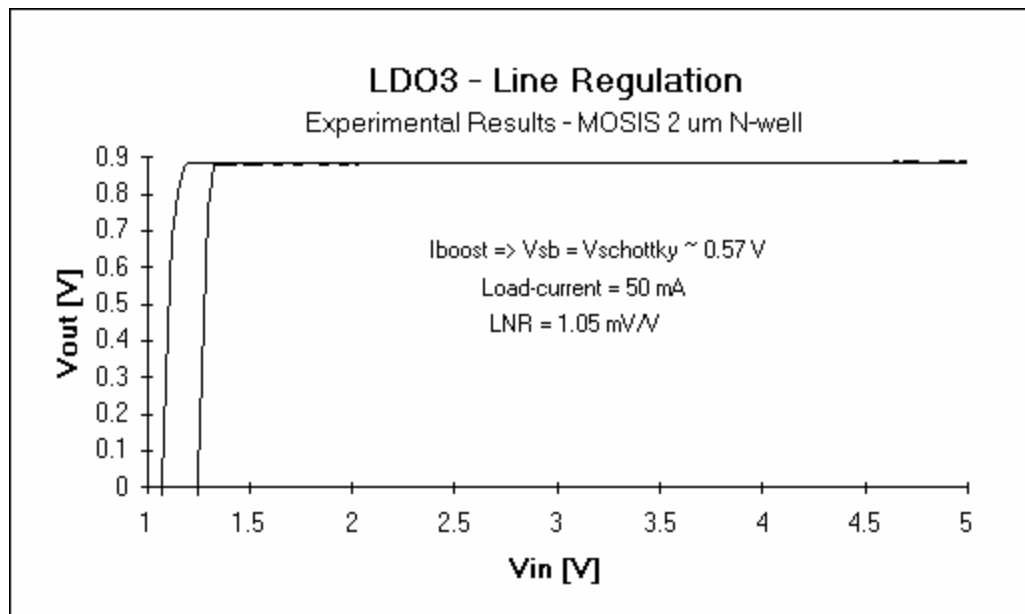
Figure 7.9. Line regulation performance of the control loop.
