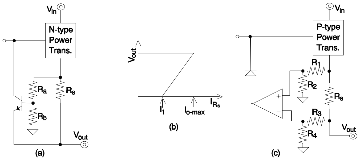
Figure 7.4. Foldback current limiting circuit protection.
