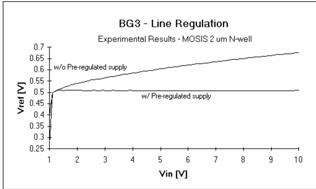
Figure 6.15. Line regulation performance of the bandgap with and without the pre-regulator.
