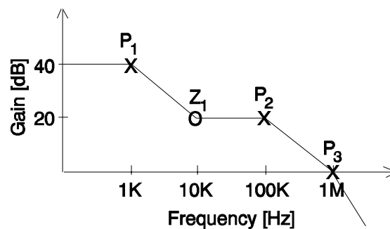
Figure 4.8. Linear regulator frequency response.
