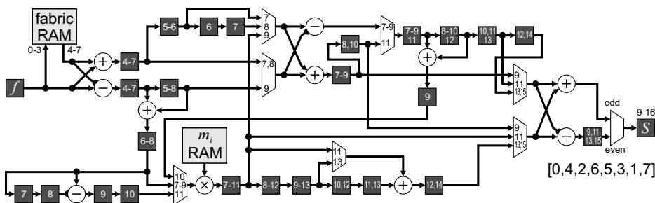
Figure 10.15 A pipelined implementation of Figure 10.14. Numbers on registers and multiplexers refer to the clock cycle they are active relative to the input samples entering on clocks 0 to 7. The registers should be clocked and the corresponding multiplexer inputs selected on these cycles.
