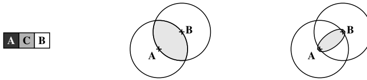
Figure 8.42 Constructs for colour edge enhancement. Left: three pixels, with C on the border between regions A and B ; centre: point C would be the vector median in the shaded region; right: a tighter criterion defined by Equation 8.25.
