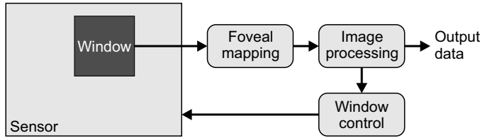
Figure 14.10 Active vision architecture using a foveal mapping.
