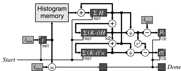
Figure 7.7 Using incremental calculations for the mean and variance.
