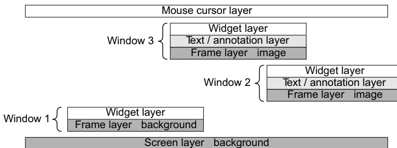
Figure 12.13 Window layering showing the arbitration priority. (Reproduced with permission from D.G. Bailey et al. , “GATEOS: A windowing operating system for FPGAs,” IEEE International Workshop on Electronic Design Test and Applications , 405–409, 2006. © 2006 IEEE.)
