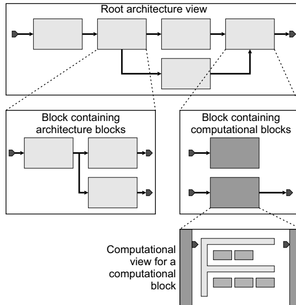
Figure 3.6 Hierarchical structure of a VERTIPH design. (Johnston, 2009; Reproduced by permission of C. Johnston.)
