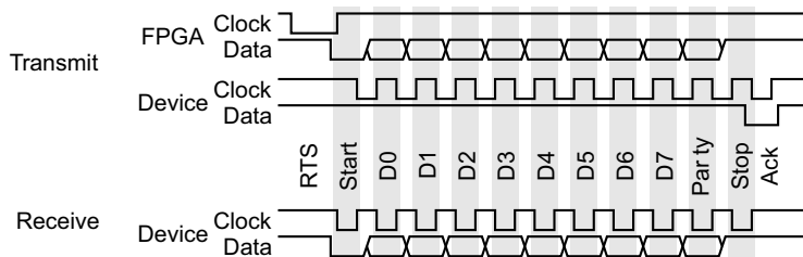
Figure 12.15 PS2 communication sequences. Top: transmission from FPGA to device; bottom: receiving from the device.
