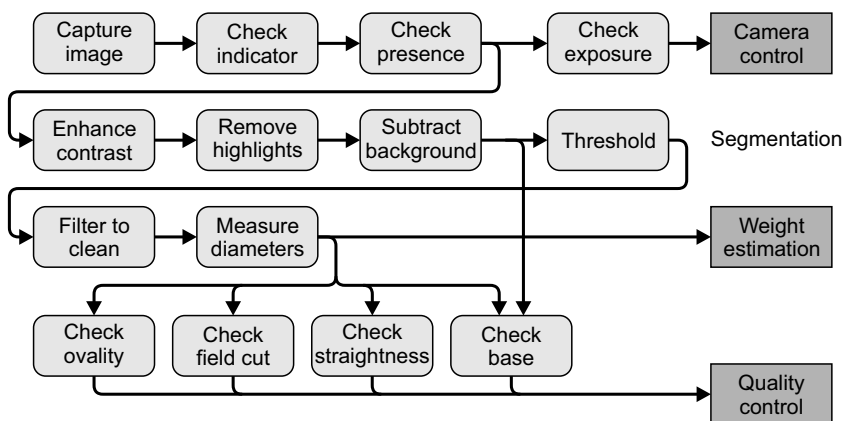
Figure 14.17 Machine vision application for grading asparagus.
