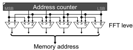
Figure 10.6 Memory read address counter for radix 2 decimation in frequency FFT.
