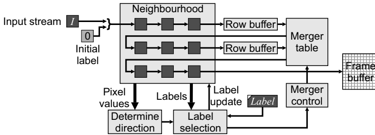
Figure 11.23 Stream based implementation of watershed segmentation.
