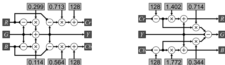
Figure 6.33 Left: conversion from RGB to YCbCr; right: conversion from YCbCr to RGB.
