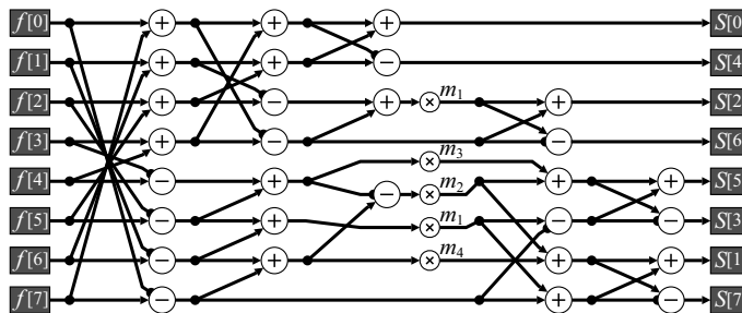
Figure 10.14 Scaled DCT (Kovac and Ranganathan, 1995), where S[u] = 4 \cos(u\pi/16) \times F[u] . The fixed multipliers are m_1 = \cos(2\pi/8) , m_2 = \cos(3\pi/8) , m_3 = \cos(\pi/8) \cos(3\pi/8) , m_4 = \cos(\pi/8) + \cos(3\pi/8) .
