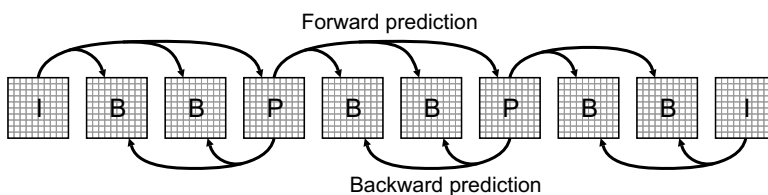
Figure 10.27 Prediction within a group of pictures, showing the relationships between I, P and B frames.
