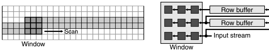
Figure 5.11 Row buffering caches the previous rows so they do not need to be read in again.
