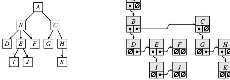
Figure 5.15 A representation of a tree.
