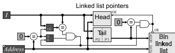
Figure 11.25 Bin sort using an array of linked lists.
