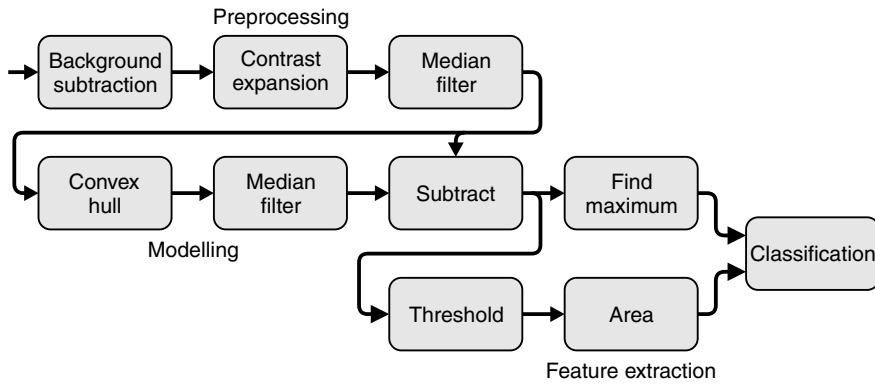
Figure 1.9 Image processing algorithm for detecting surface defects on kiwifruit (Bailey, 1985).
