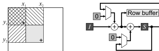
Figure 9.12 Left: using a summed area table to find the sum of pixel values within an arbitrary rectangular area; right: efficient streamed implementation to create a summed area table.
