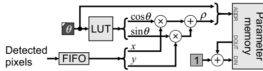
Figure 11.30 Vote accumulator for line Hough transform.
