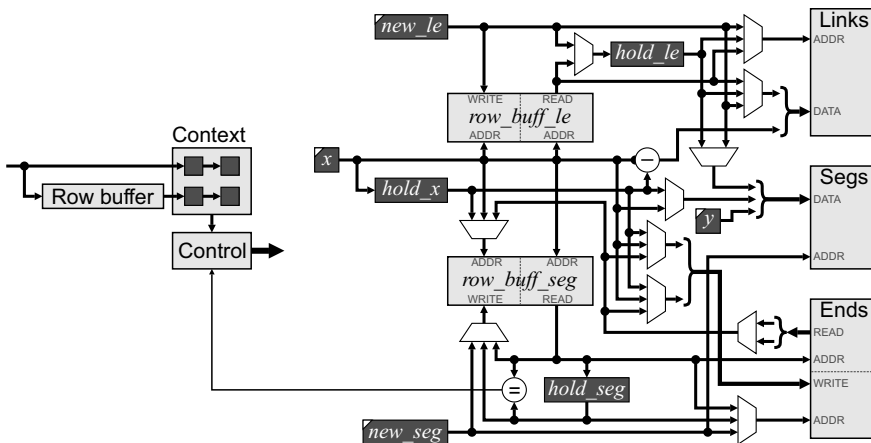
Figure 11.9 Block diagram of raster based crack code follower.
