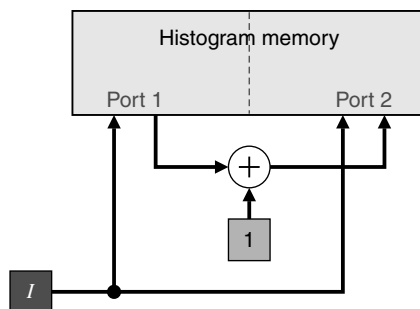
Figure 7.3 Histogram accumulation using dual port memory.
