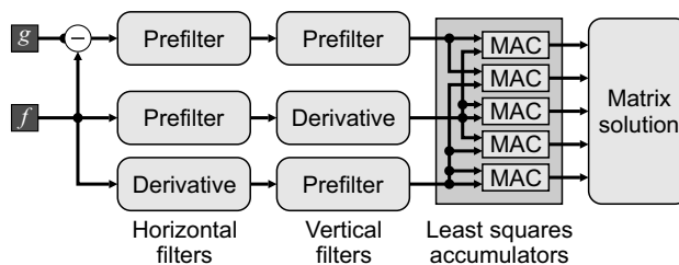
Figure 9.28 Basic approach of gradient based registration.
