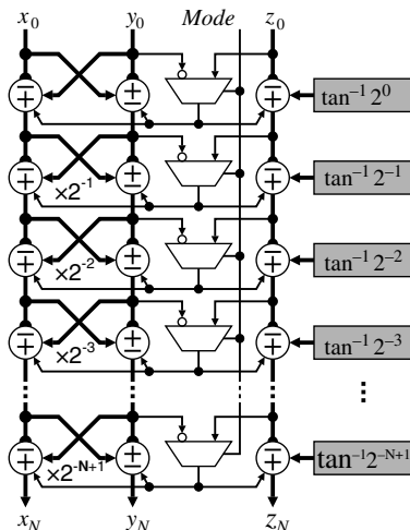
Figure 5.34 Unrolled CORDIC implementation.
