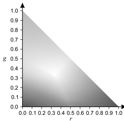
Figure 6.41 Device dependent r g chromaticity. (See colour version of this figure in colour plate section)
