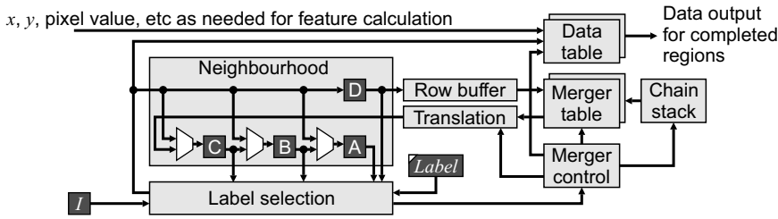
Figure 11.15 Single pass connected components analysis with label reuse.
