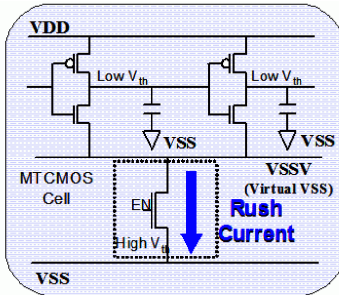
Figure 5-14 Rush Current Upon Power-Up
