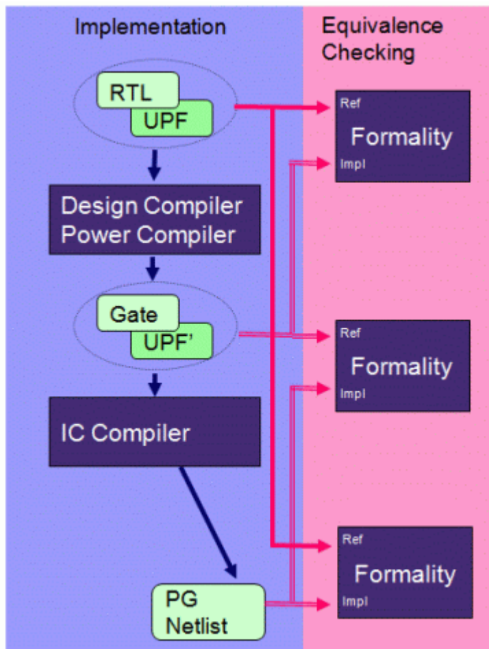
Figure 5-13 Formality Equivalence Checking With UPF
