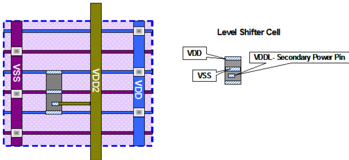
Figure 5-8 Level Shifter With Dual Power Pins
