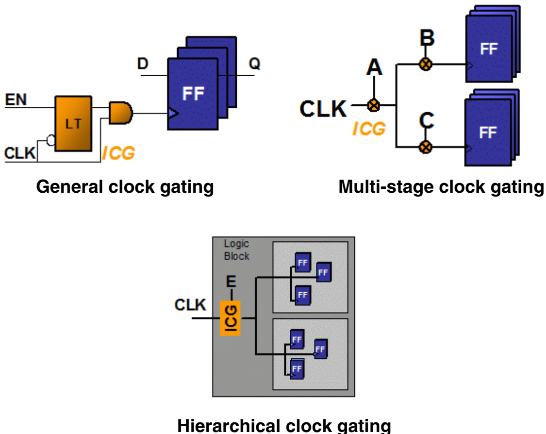
Figure 5-6 Clock-Gating Styles
