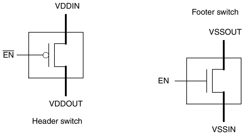
Figure 2-5 Power-Switch Cells
