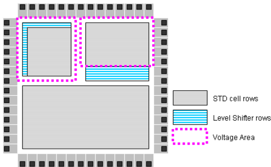
Figure 5-9 Multivoltage Floorplan
