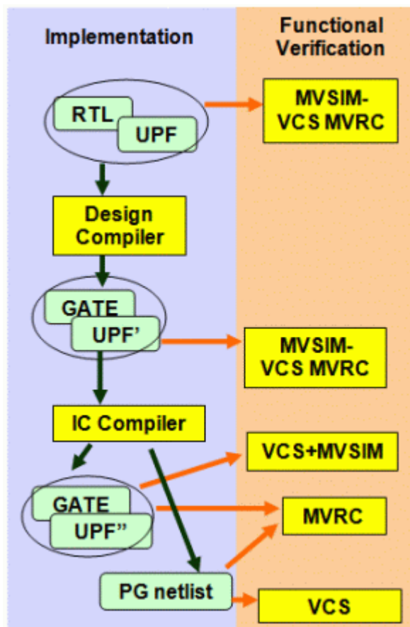
Figure 5-2 Power-Aware Verification Flow
