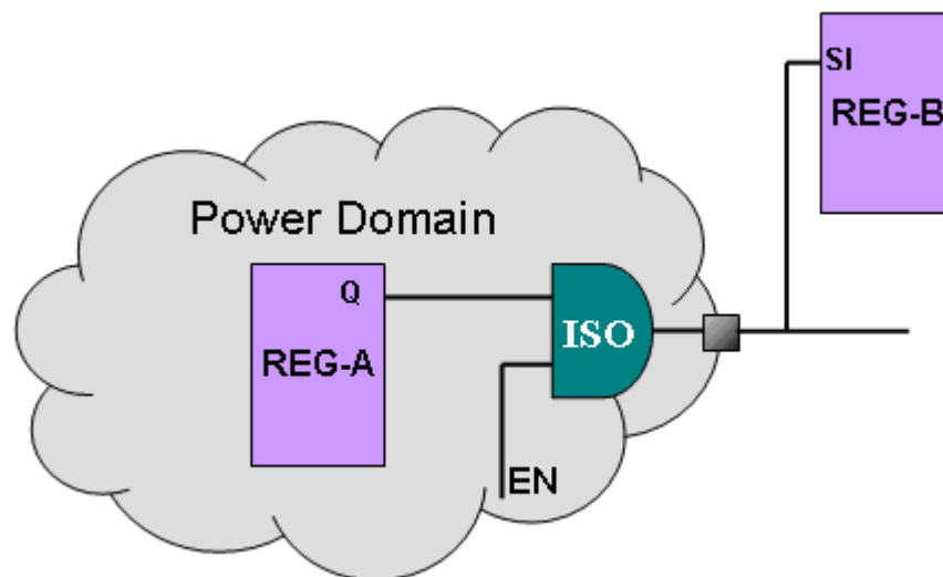
Figure 5-7 Scan Insertion Through Isolation Cell
