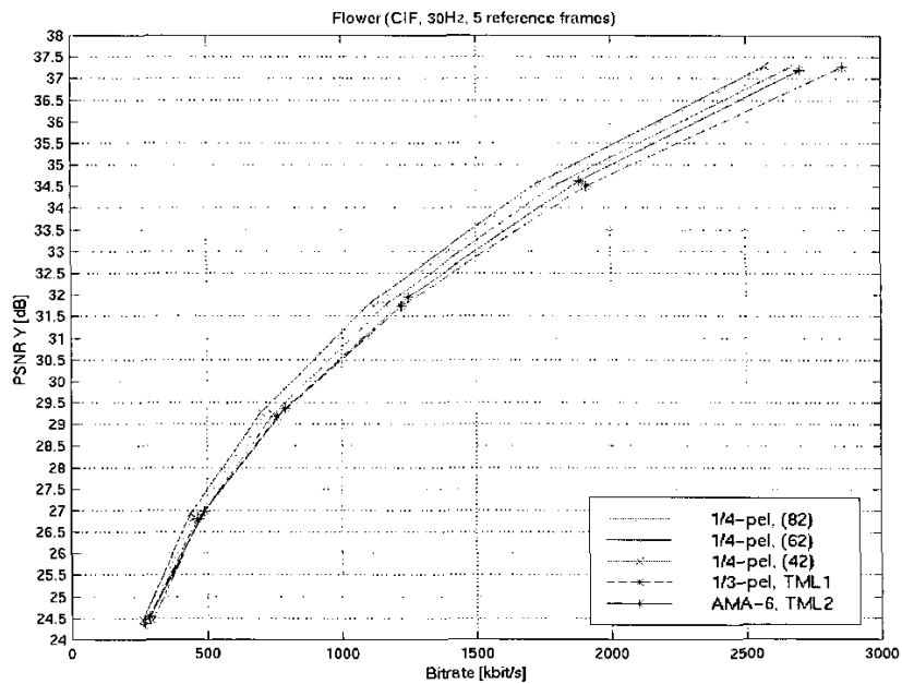
Fig. 41. Rate distortion graph for \frac{1}{4} - pel accuracy for Flower CIF sequence [2]
