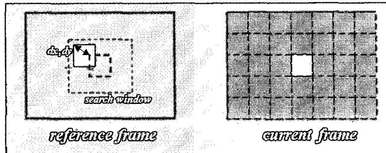
Fig. 31. Block based motion estimation dx, dy represent the differential motion vectors
