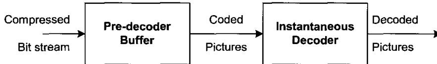
Fig. 3. A Hypothetical Reference Buffer [1]
