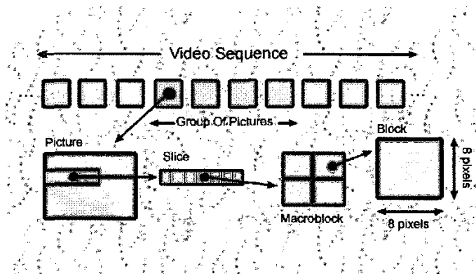
Fig. 18. Sequence-GOP-picture-slice-macroblock-block
