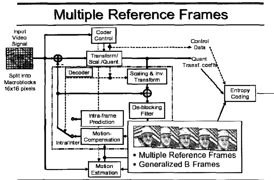
Fig. 24. Block Diagram illustrating multiple reference frames [10]
