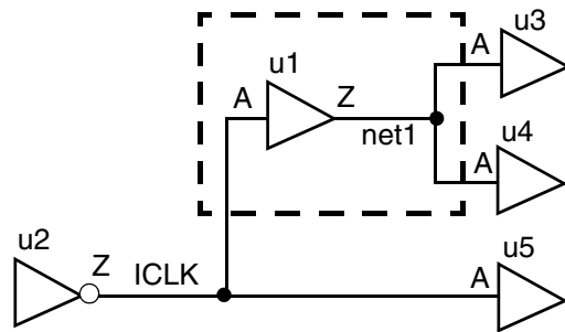
Figure 3-5 New Circuit
