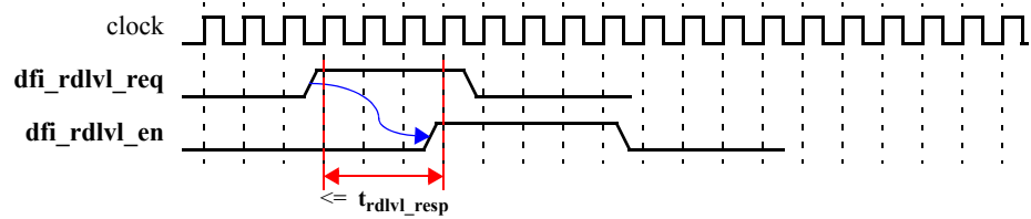
Data Eye Training Request Timing
