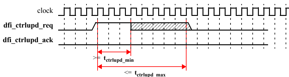
MC-Initiated Update with No Response
