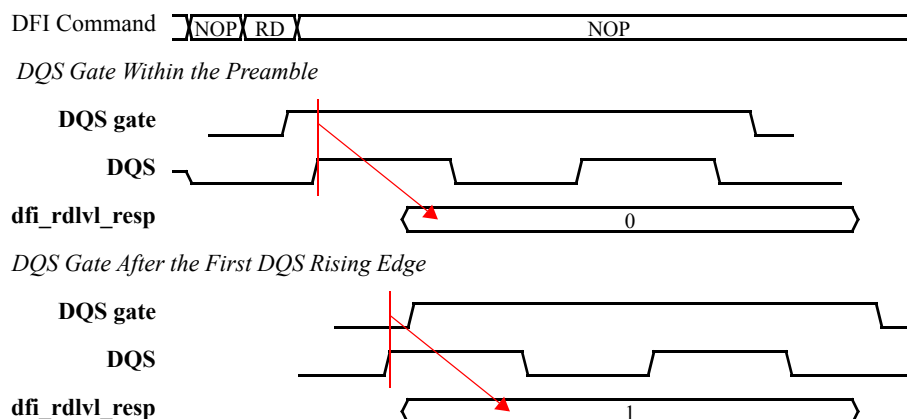
Gate Training Response During Gate Training for a Single Data Slice
