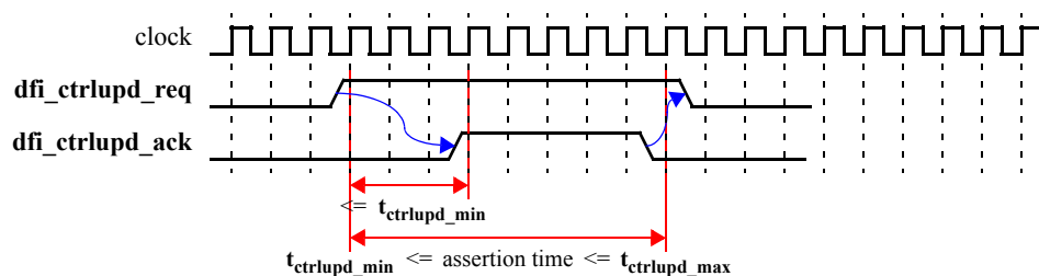
MC-Initiated Update Timing Diagram
