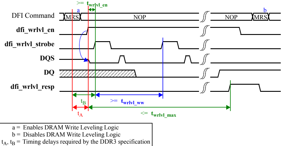
Write Leveling in PHY Evaluation Mode
