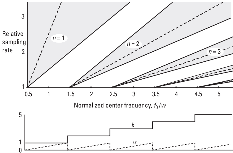
Figure 4.8 Relative sampling rates (uniform sampling).
