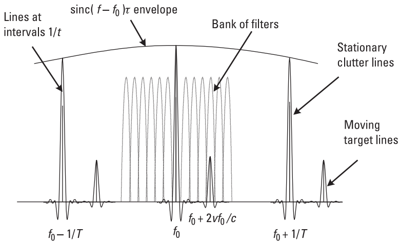
Figure 3.21 Spectrum of pulse Doppler radar waveform.
