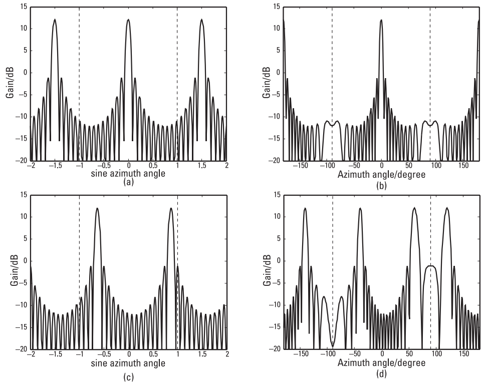
Figure 7.2 Beam patterns for a uniform linear array: (a) broadside beam, u -space; (b) broadside beam, angle space; (c) beam at 60 degrees, u -space; (d) beam at 60 degrees, angle space.
