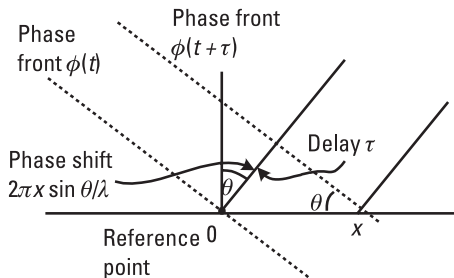
Figure 7.1 Aperture phase shift.
