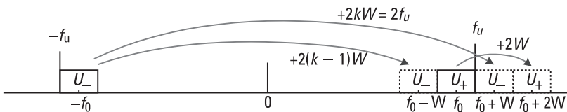
Figure 4.4 Allowed spectral shifts.
