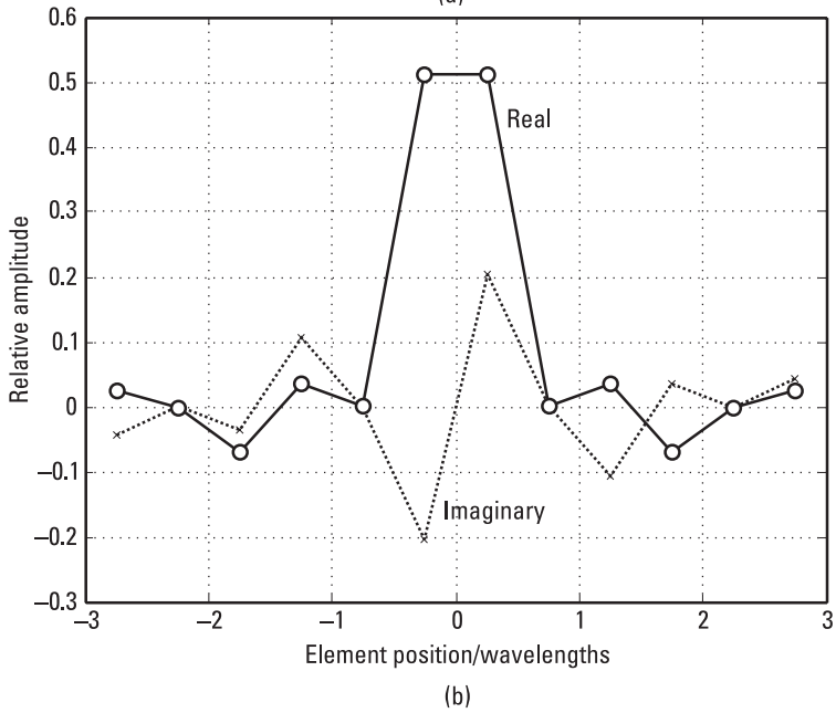
Figure 7.8 Steered sector beam with reflector-backed elements: (a) beam patterns; (b) element weights.
