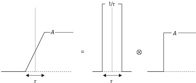
Figure 3.6 Rising edge of width \tau .
