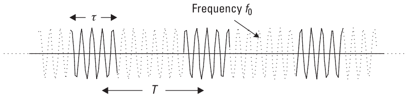
Figure 3.19 Carrier gated by a regular pulse train.
