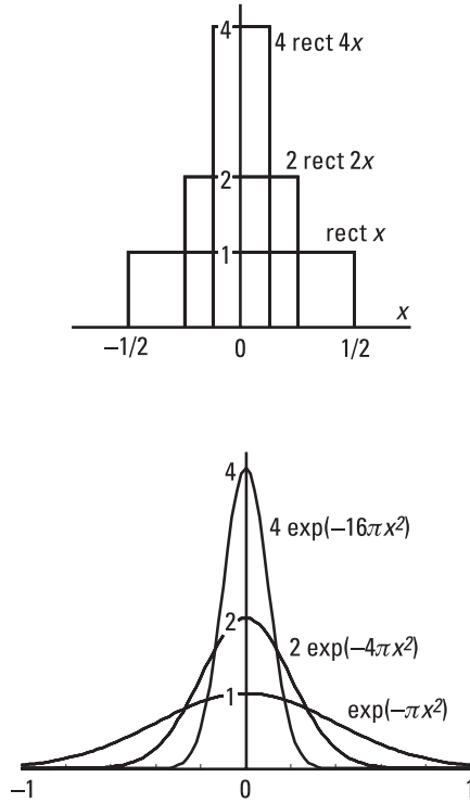
Figure 2.3 Two series approximating \delta -functions.
