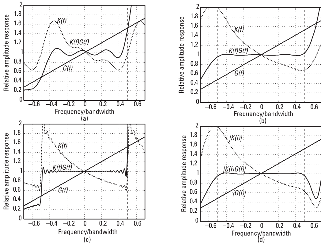
Figure 6.4 Equalization of linear amplitude distortion: (a) m = 7, q = 1 ; (b) m = 7, q = 1.5 ; (c) m = 47, q = 1 ; (d) m = 7, q = 1.5 , delay 0.5.
