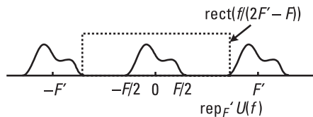
Figure 5.6 Optimum rectangular gate for oversampled time series.
