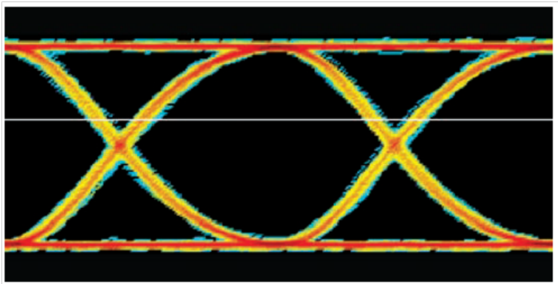
Figure 22. Duty Cycle Distortion Caused by Incorrect Detection Threshold
