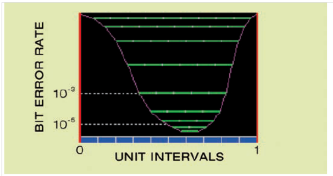
Figure 28. Measuring Eye Width Over Time to Determine Bit Error Ratio
