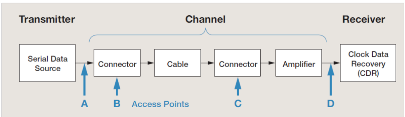
Figure 26. Common Measurement Points for Setting System Jitter Budgets
