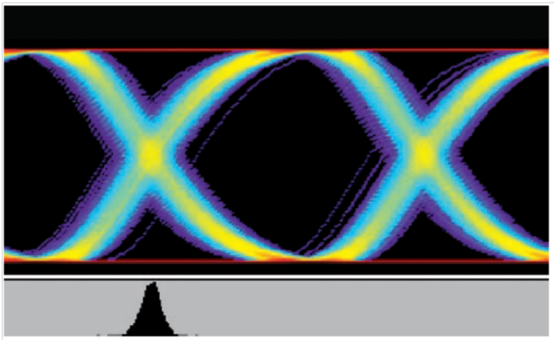
Figure 15. An Eye Diagram and Histogram of Gaussian Jitter
