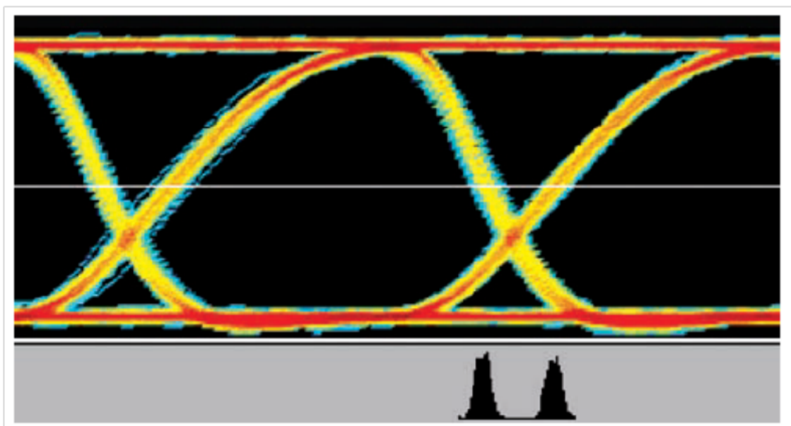
Figure 21. Duty Cycle Distortion Caused by Non-symmetrical Rise/Fall Times
