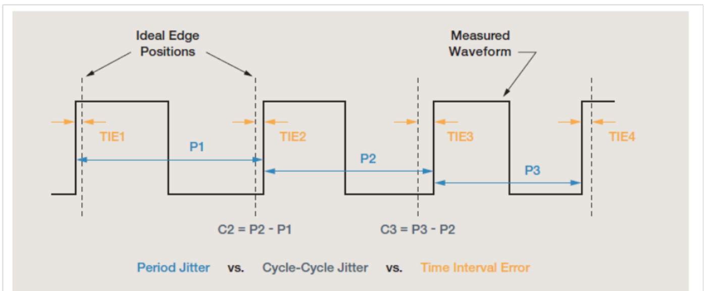
Figure 1. Different Measurements of Jitter
