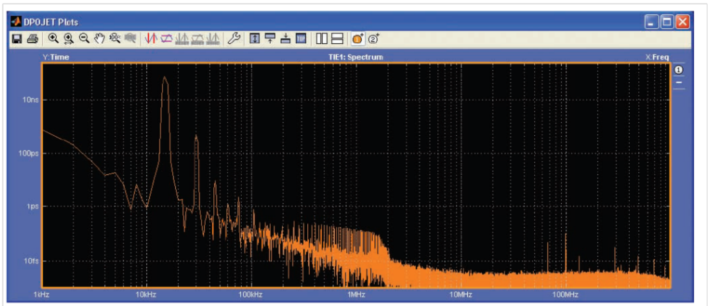
Figure 9. Time Interval Error of a Modulated Signal plotted as a Spectrum
