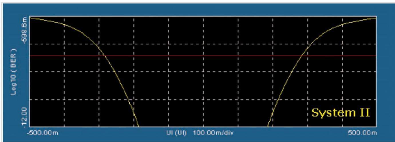
Figure 30. BER Plot of System with Dominant Deterministic Jitter
