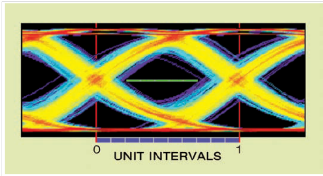
Figure 27. Eye Width is used to Determine Performance
