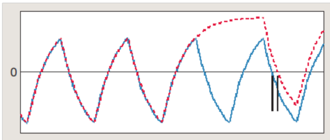
Figure 19. Limited Bandpass One Source of Data Dependent Jitter
