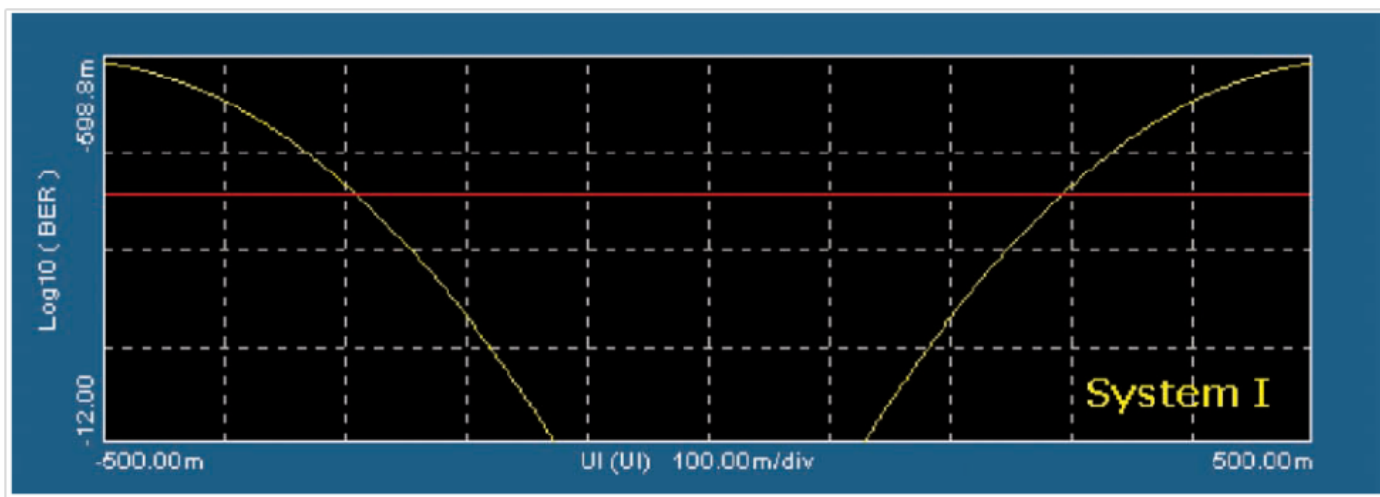
Figure 29. BER Plot of System with Dominant Random Jitter
