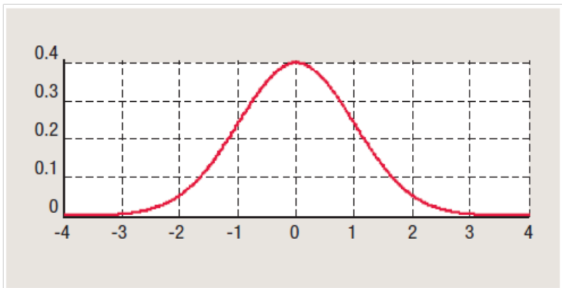
Figure 14. Gaussian Distribution
