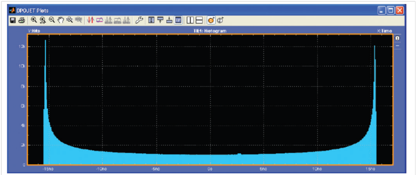
Figure 7. Time Interval Error of a Modulated Signal plotted as a Histogram.
