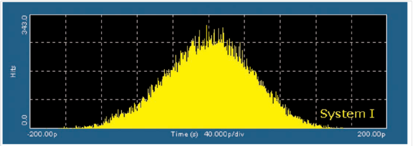
Figure 24. A Histogram of a Jitter Distribution with Dominant Random Jitter
