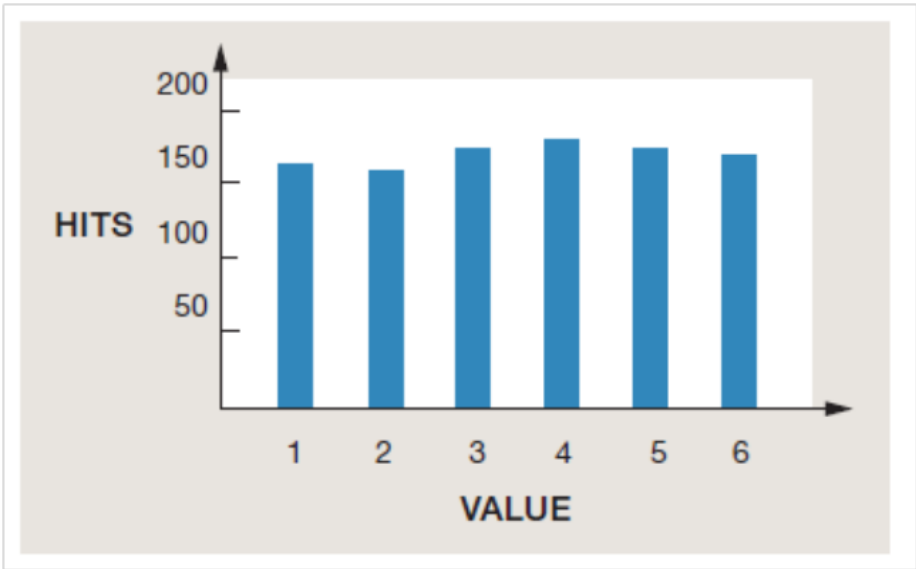
Figure 4. Measurement Histogram
