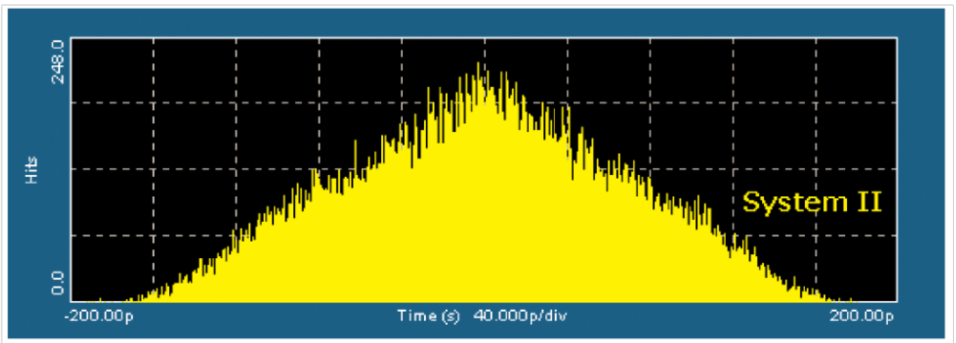
Figure 25. A Histogram of a Jitter Distribution with Dominant Deterministic Jitter
