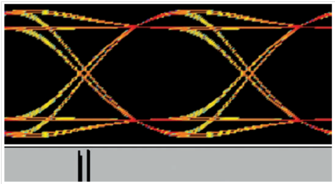
Figure 20. An Eye Diagram and Histogram of Data Dependent Jitter
