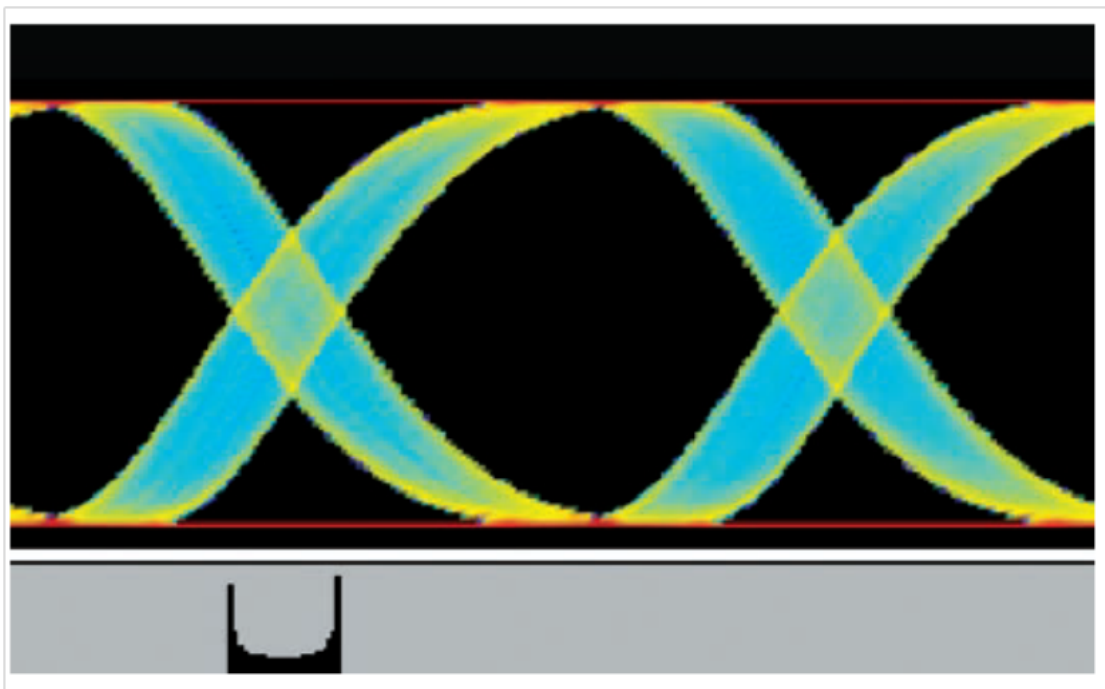
Figure 17. An Eye Diagram and Histogram of non-Gaussian Jitter
