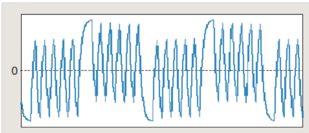
Figure 18. Data Signal with Data Dependent Jitter
