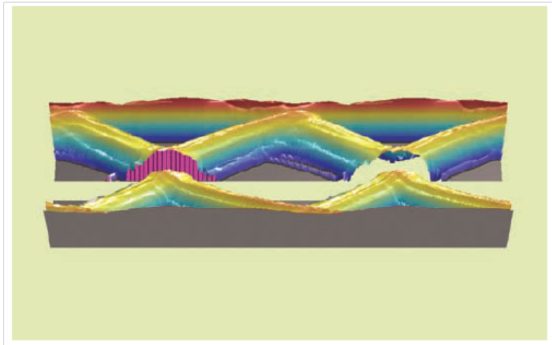
Figure 12. In a Waveform Database, Colors can Represent Population Jitter & BER
