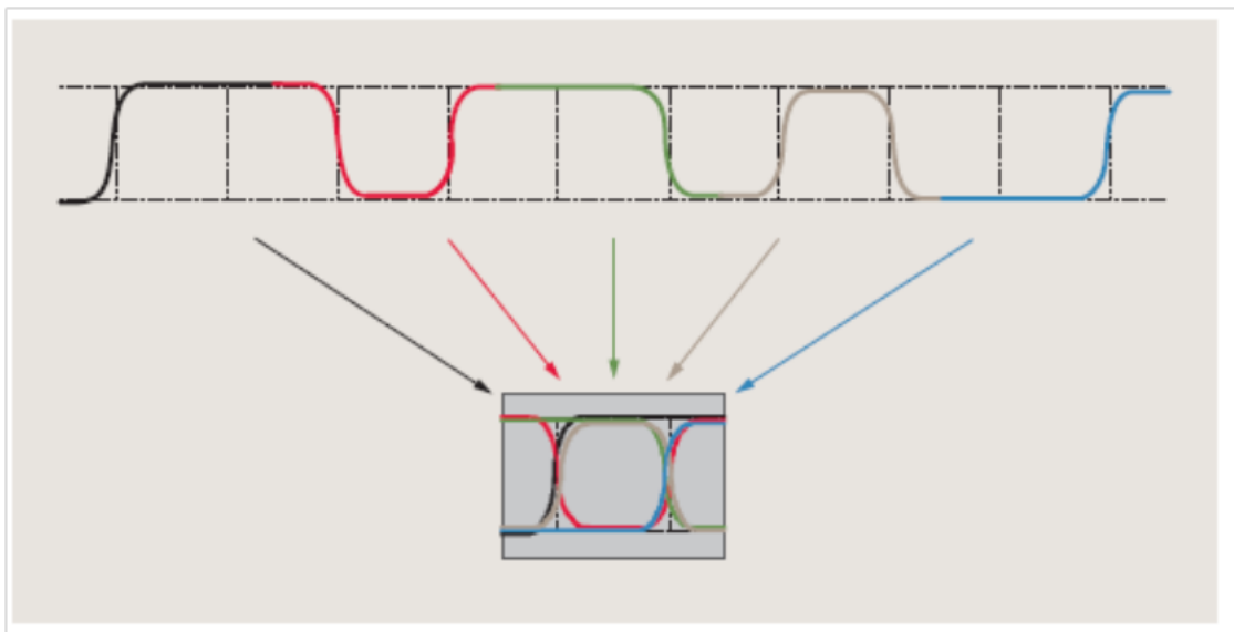
Figure 10. Constructing a Real-Time Eye Diagram
