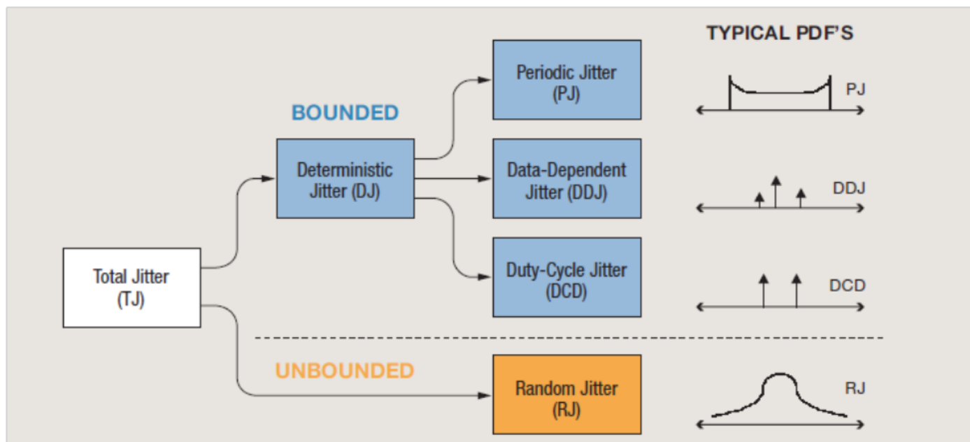
Figure 13. Jitter is Composed of Random and Deterministic Parts
