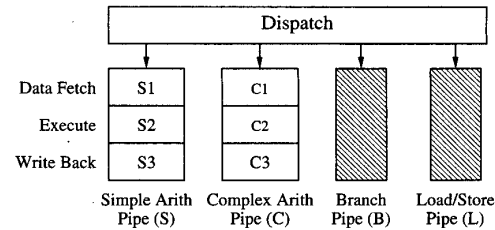
Figure 3: The structure of the NorthStar pipeline
