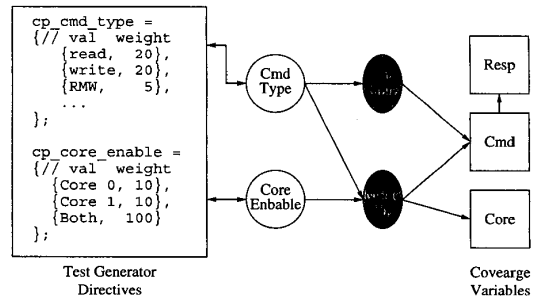
Figure 2: Bayesian Network of CDG
