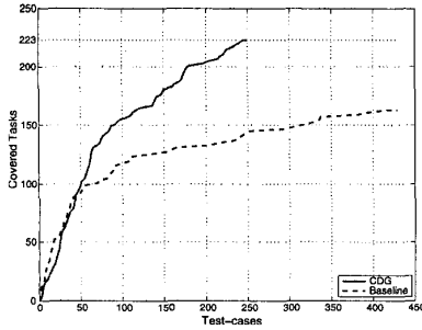
Figure 6: Coverage progress of the CDG process
