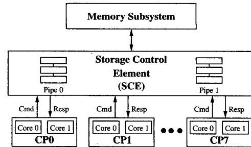
Figure 5: The structure of SCE simulation environment
