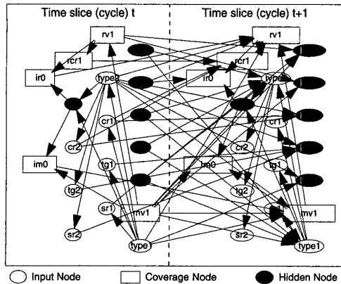
Figure 4: two-slice DBN for the NorthStar experiment
