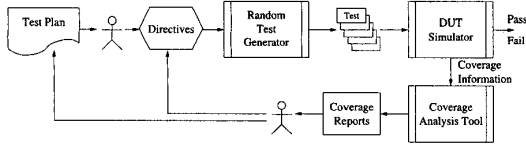
Figure 1: Verification process with automatic test generation
