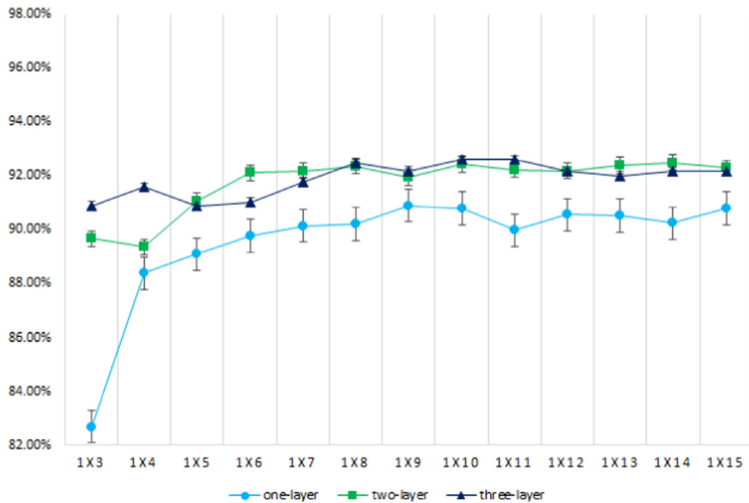
Fig. 5. Performance of convnet with increasing filter size M .
