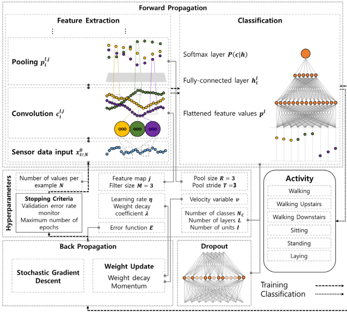
Fig. 3. The overview of the convolutional neural network used for this paper.
