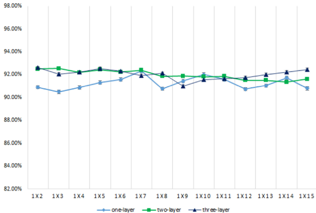
Fig. 6. Performance of convnet with increasing pooling size R .
