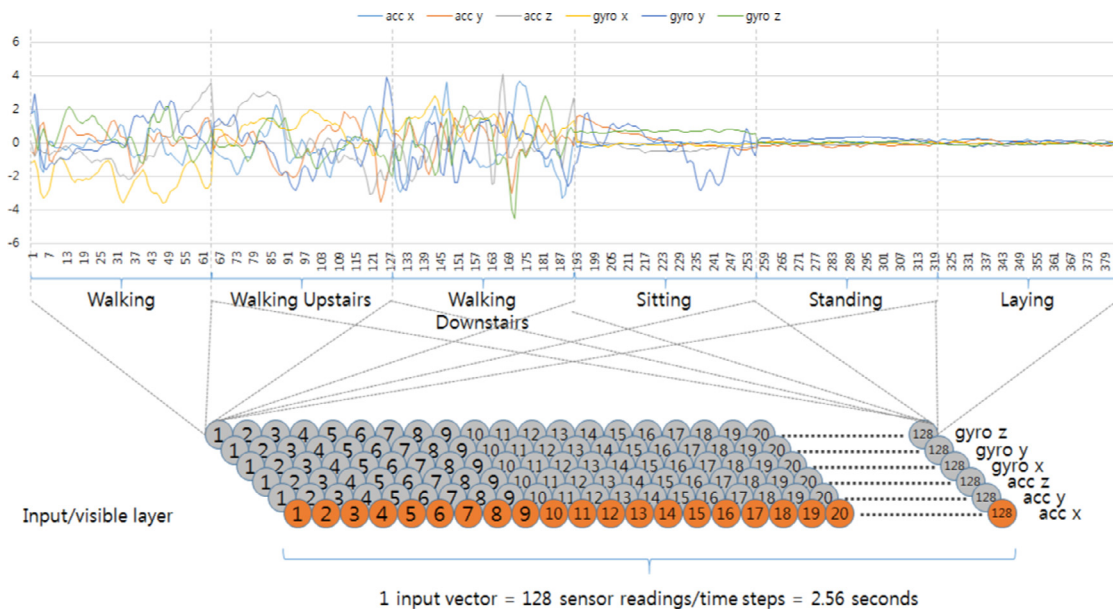
Fig. 1. 1D time-series multi-axes sensor input signal.
