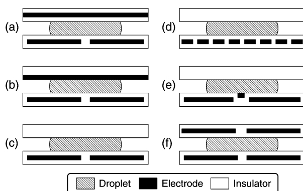
Fig. 3 Alternative microactuator electrode arrangements.
