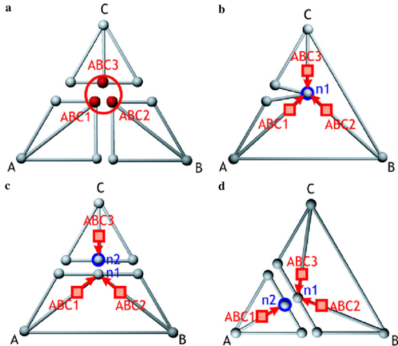
Fig. 5. Virtual nodes for a progressive face subdivision.
