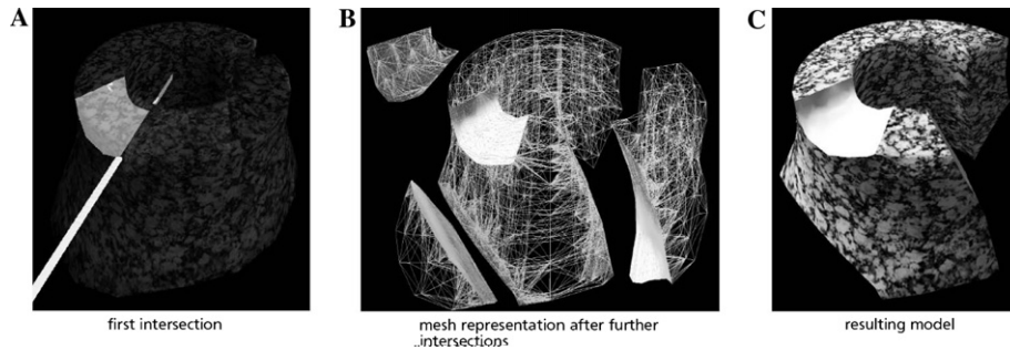
Fig. 16. Virtual sculpting.
