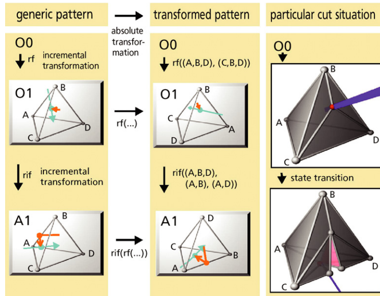
Fig. 7. Simple example for transformations.
