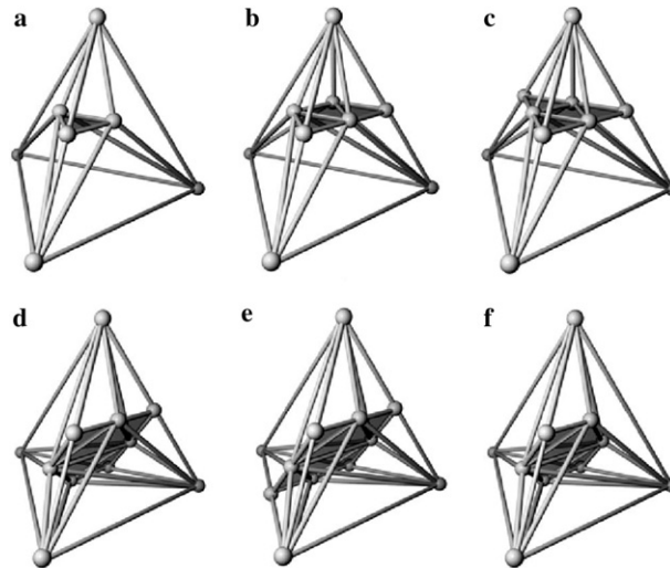
Fig. 2. Individual subdivision patterns for each subdivision topology of a tetrahedron.
