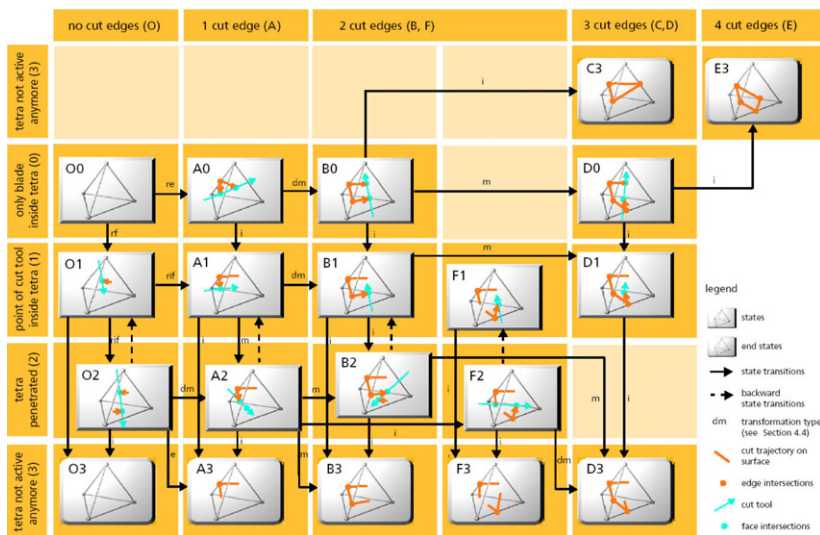
Fig. 3. State machine diagram.
